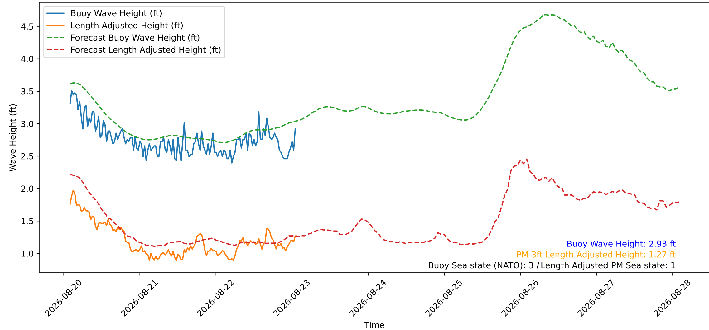
Wave Heights over Time for Green Beach at 2026-08-23 01:51:14
