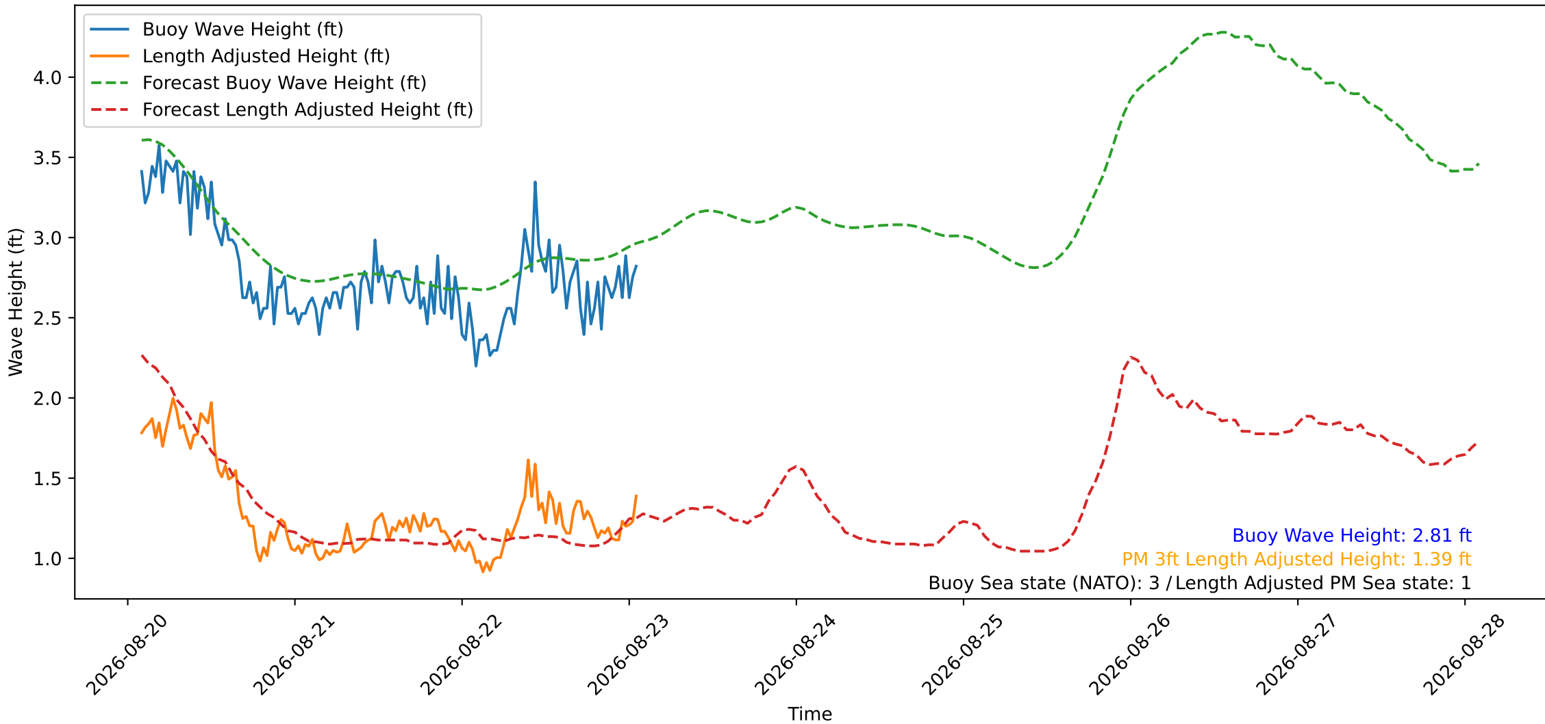
Wave Heights over Time for Oceanside Harbor at 2026-08-23 01:50:29
