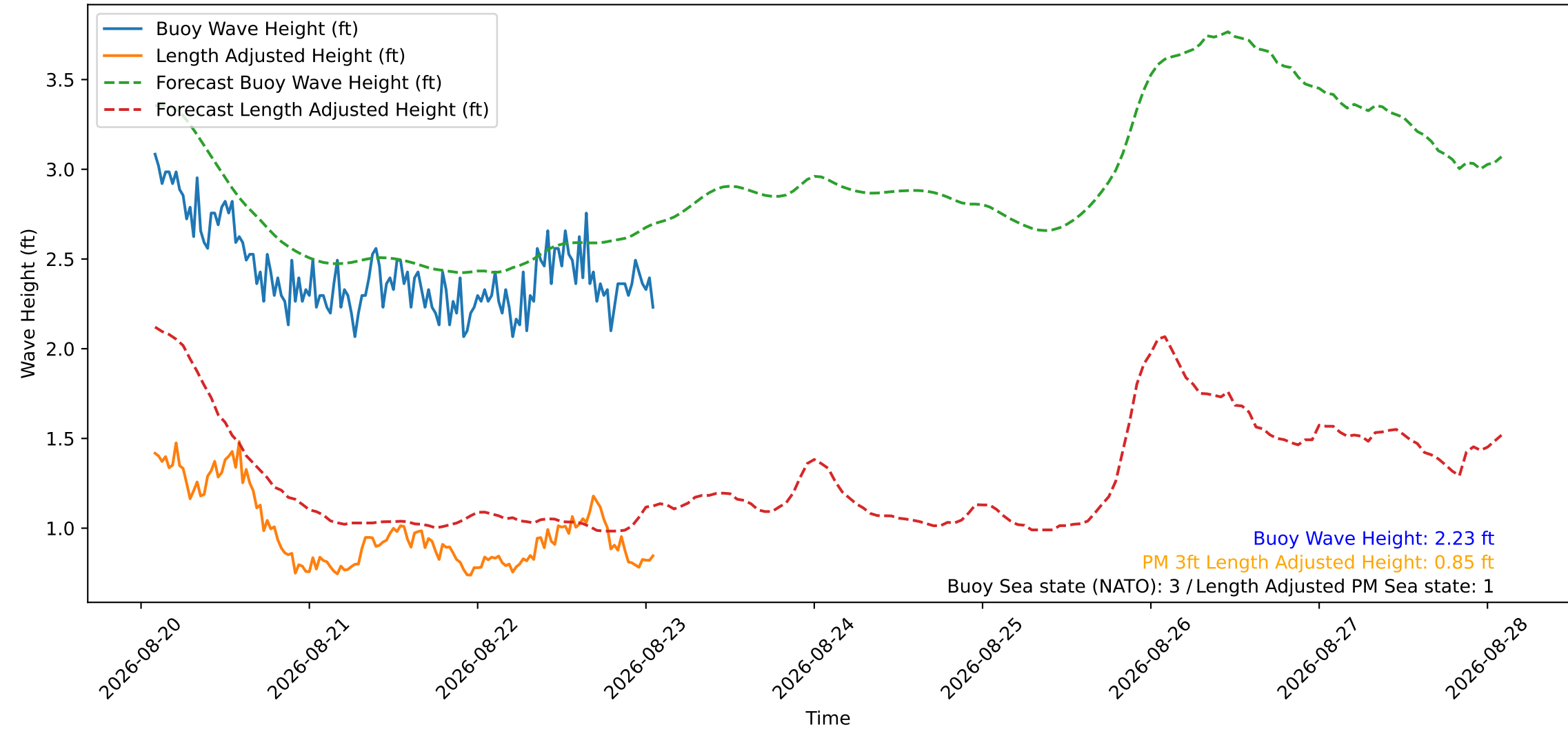
Wave Heights over Time for Red Beach at 2026-08-23 01:50:50
