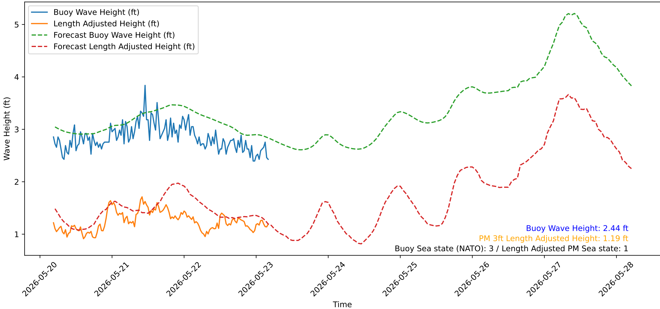
Wave Heights over Time for Oceanside Harbor at 2026-05-23 04:30:32
