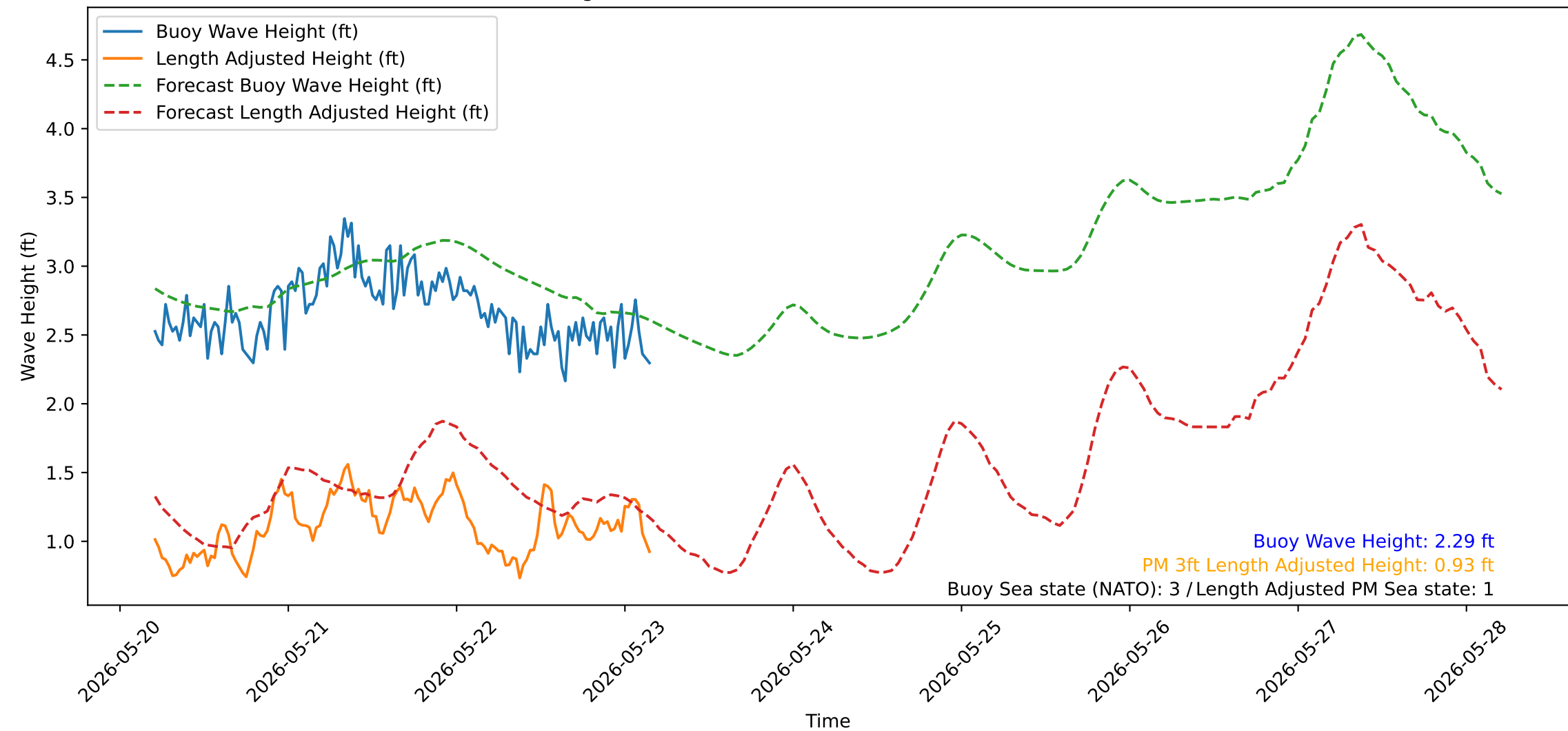
Wave Heights over Time for Red Beach at 2026-05-23 04:30:51
