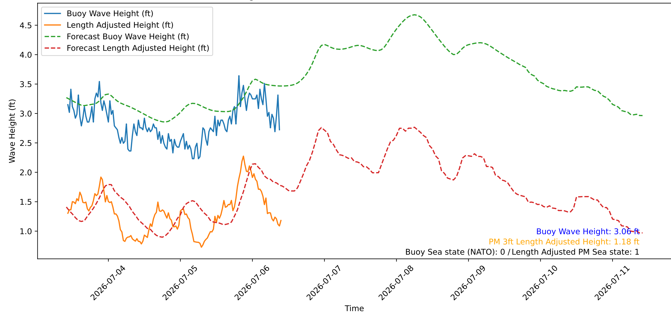
Wave Heights over Time for Red Beach at 2026-07-06 10:10:45
