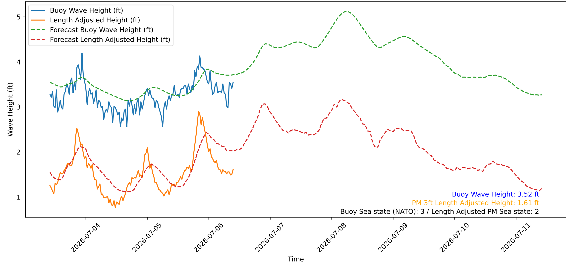
Wave Heights over Time for Green Beach at 2026-07-06 10:11:08
