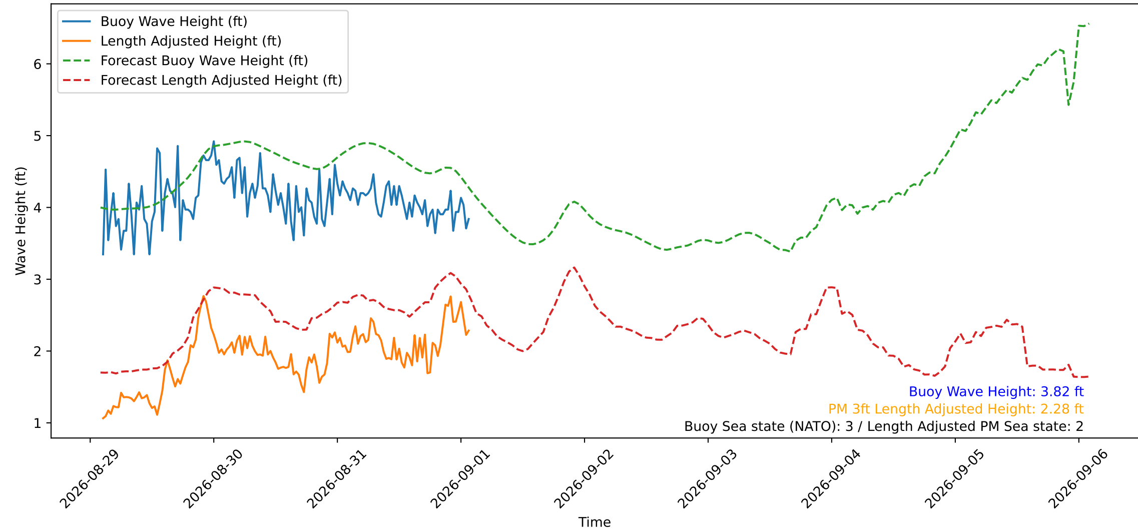
Wave Heights over Time for Green Beach at 2026-09-01 02:11:13
