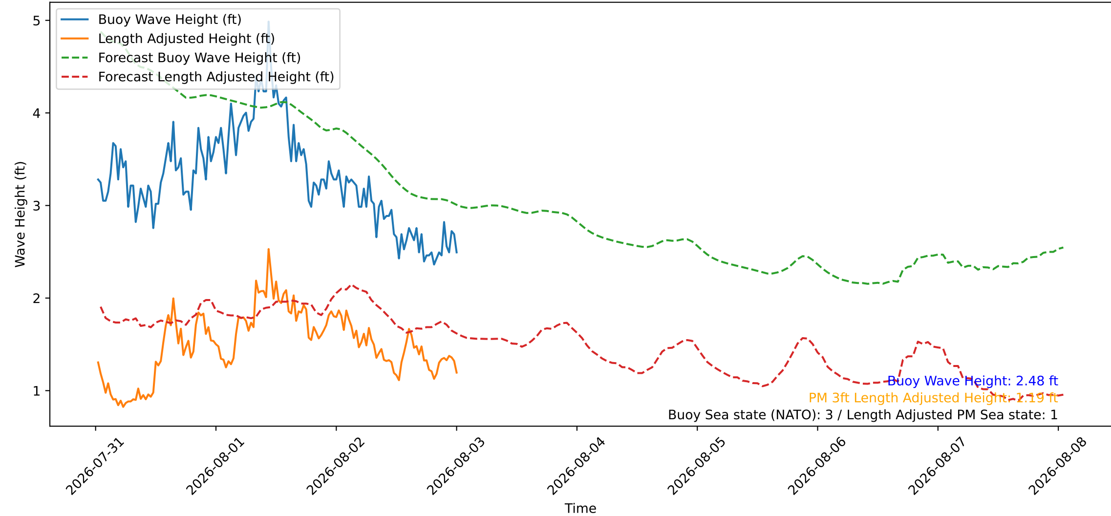
Wave Heights over Time for Green Beach at 2026-08-03 00:41:09
