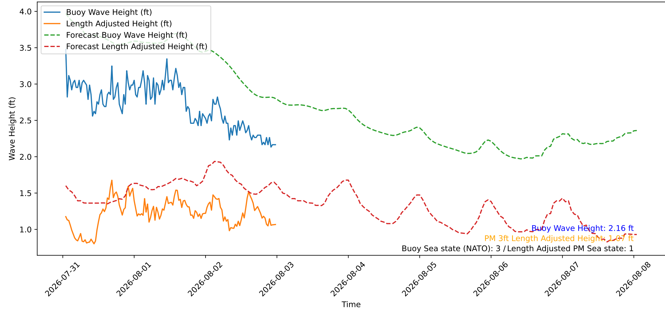
Wave Heights over Time for Red Beach at 2026-08-03 00:40:46
