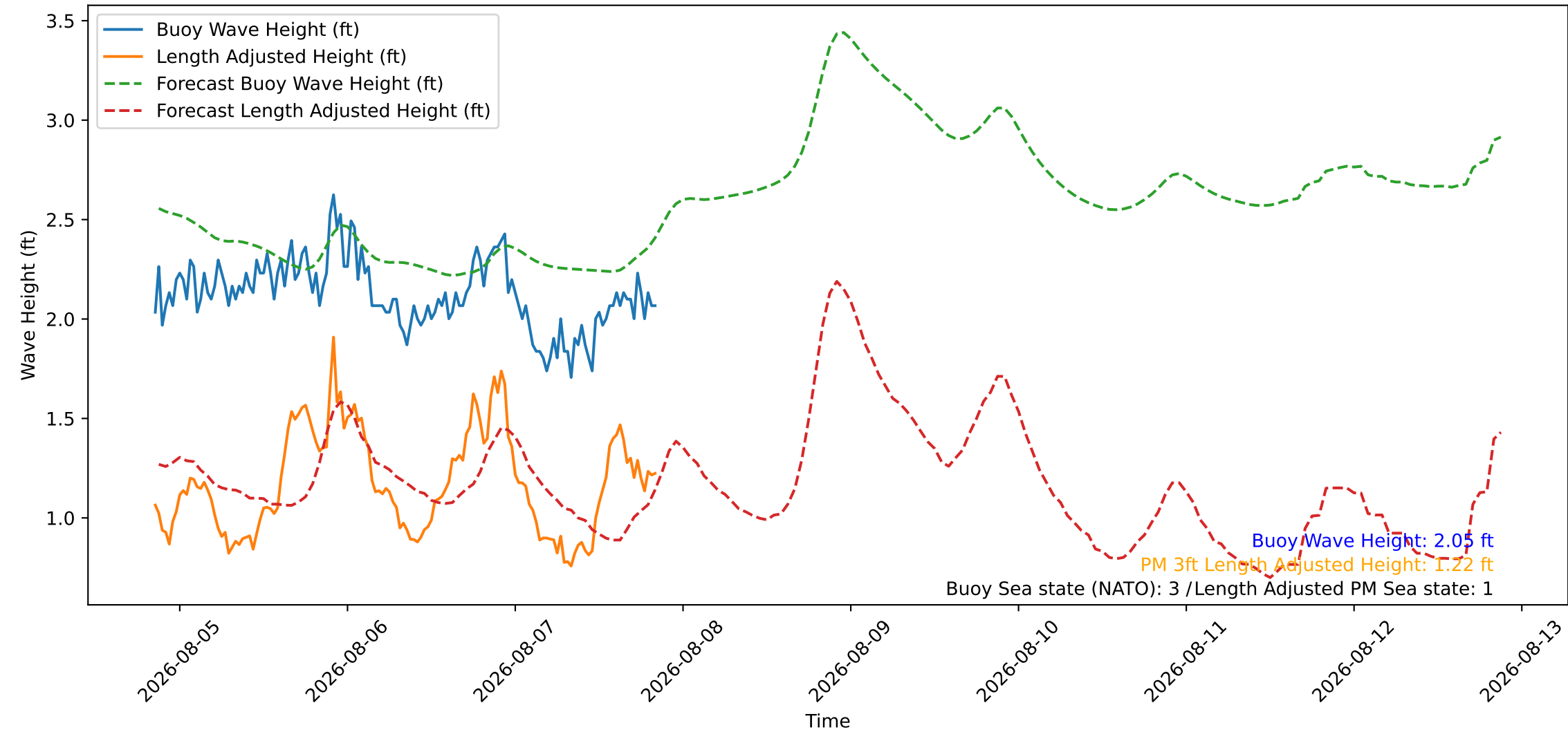
Wave Heights over Time for Green Beach at 2026-08-07 20:41:08
