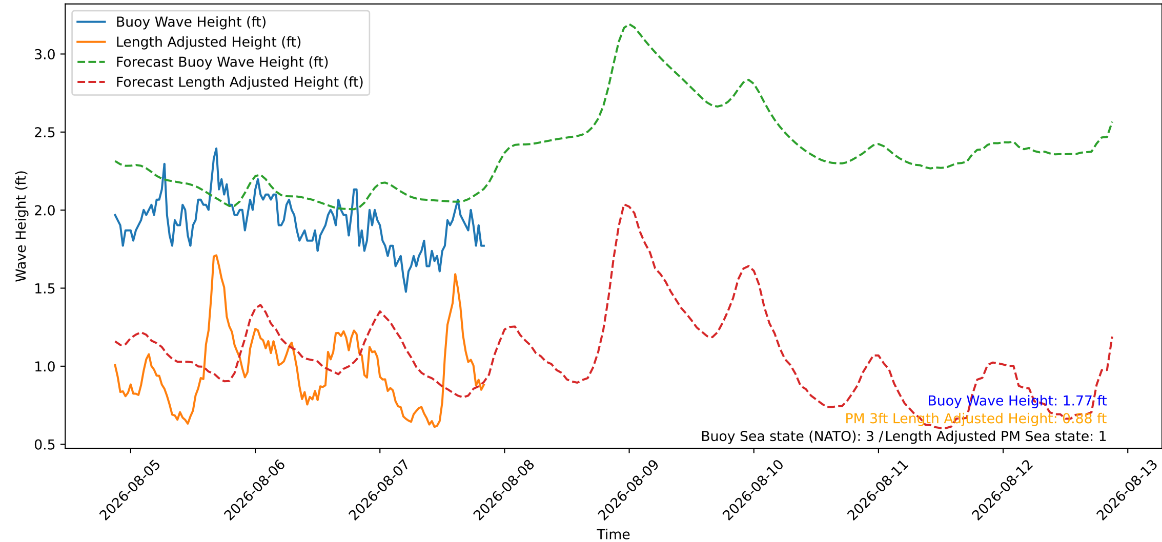
Wave Heights over Time for Red Beach at 2026-08-07 20:40:46
