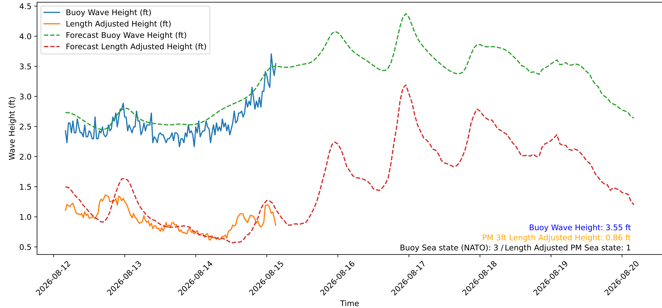
Wave Heights over Time for Red Beach at 2026-08-15 03:40:46
