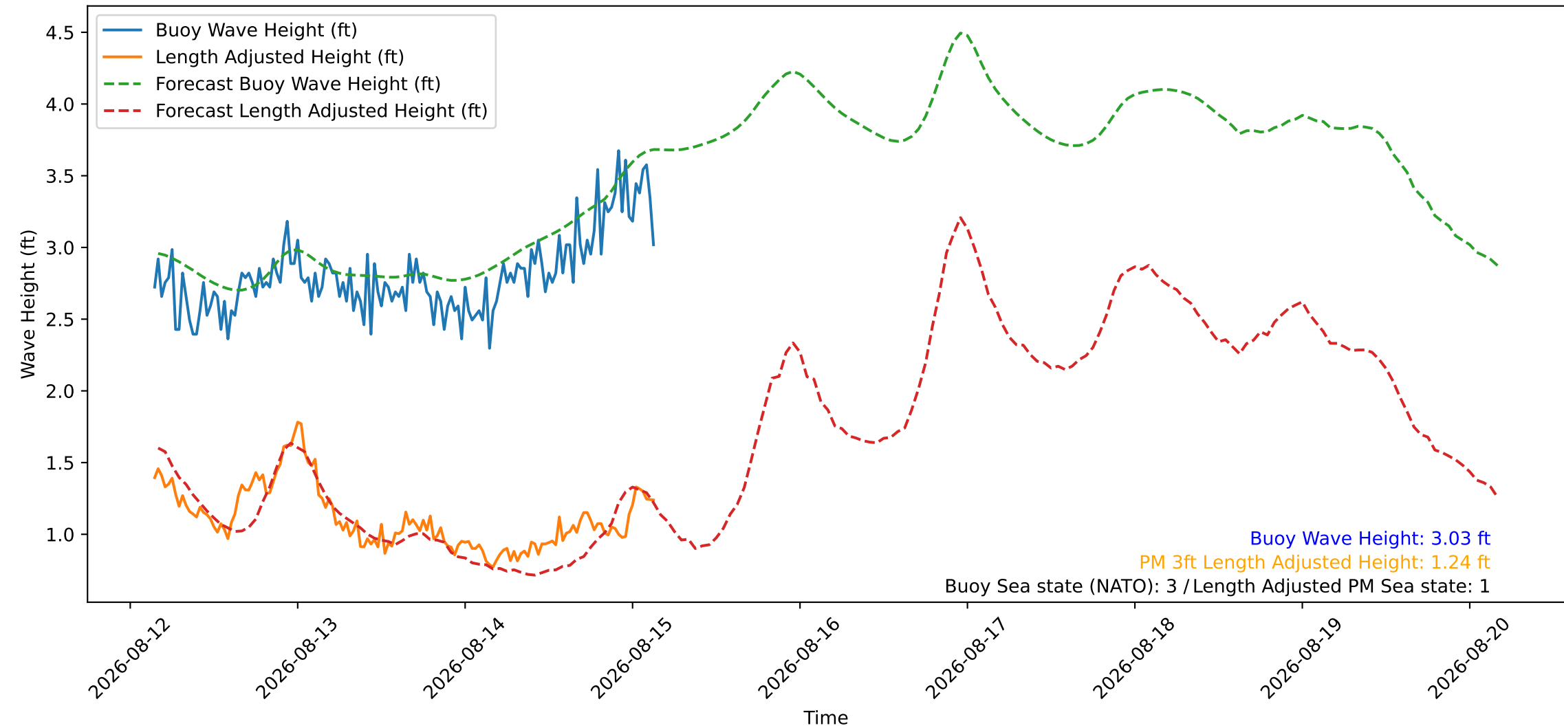
Wave Heights over Time for Oceanside Harbor at 2026-08-15 03:40:27
