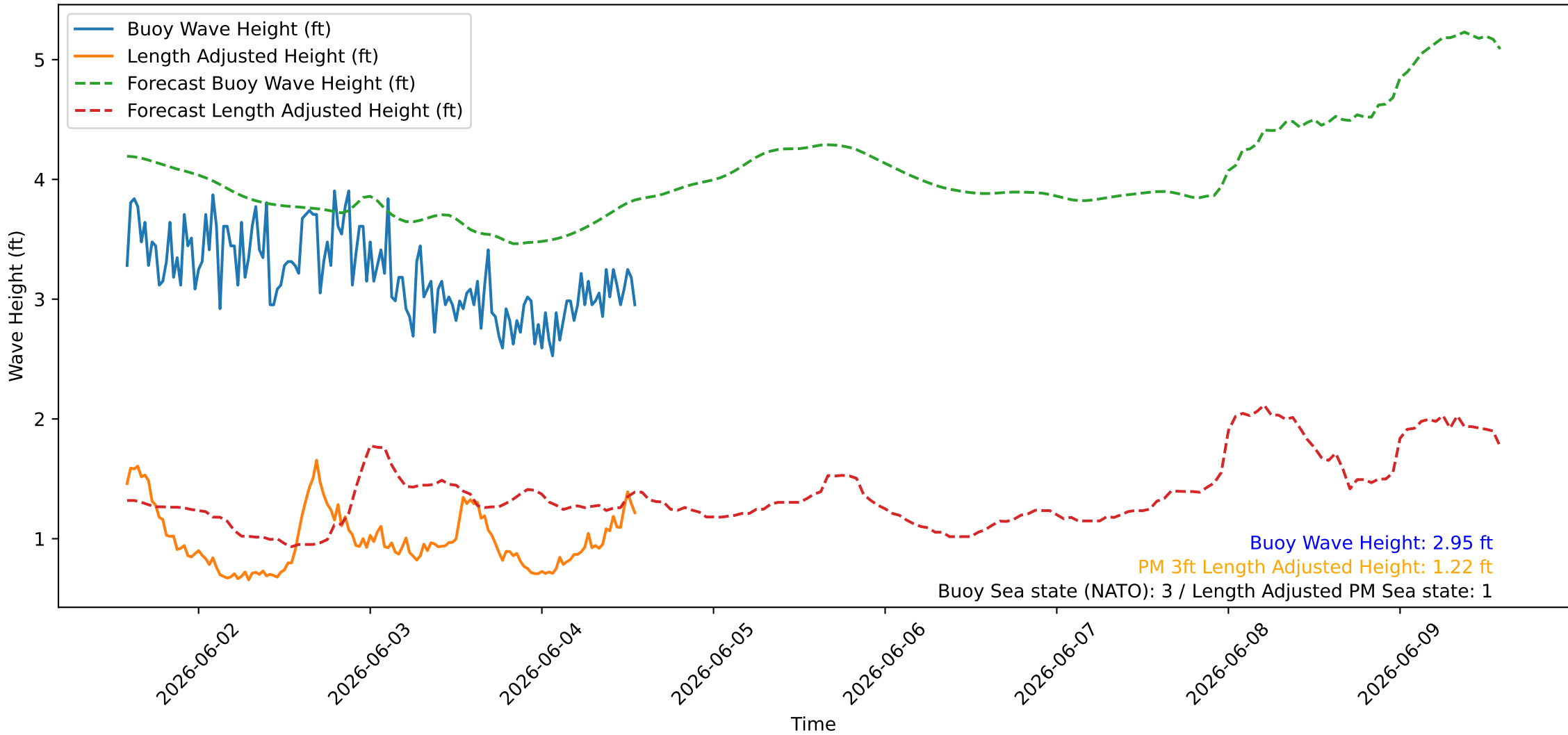
Wave Heights over Time for Red Beach at 2026-06-04 13:50:47
