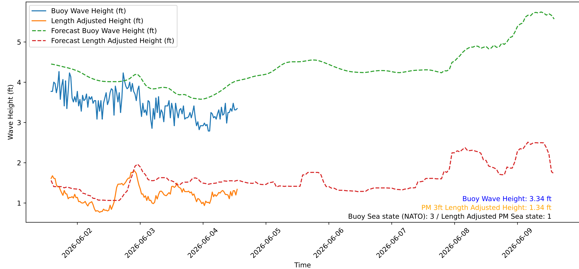
Wave Heights over Time for Green Beach at 2026-06-04 13:51:09
