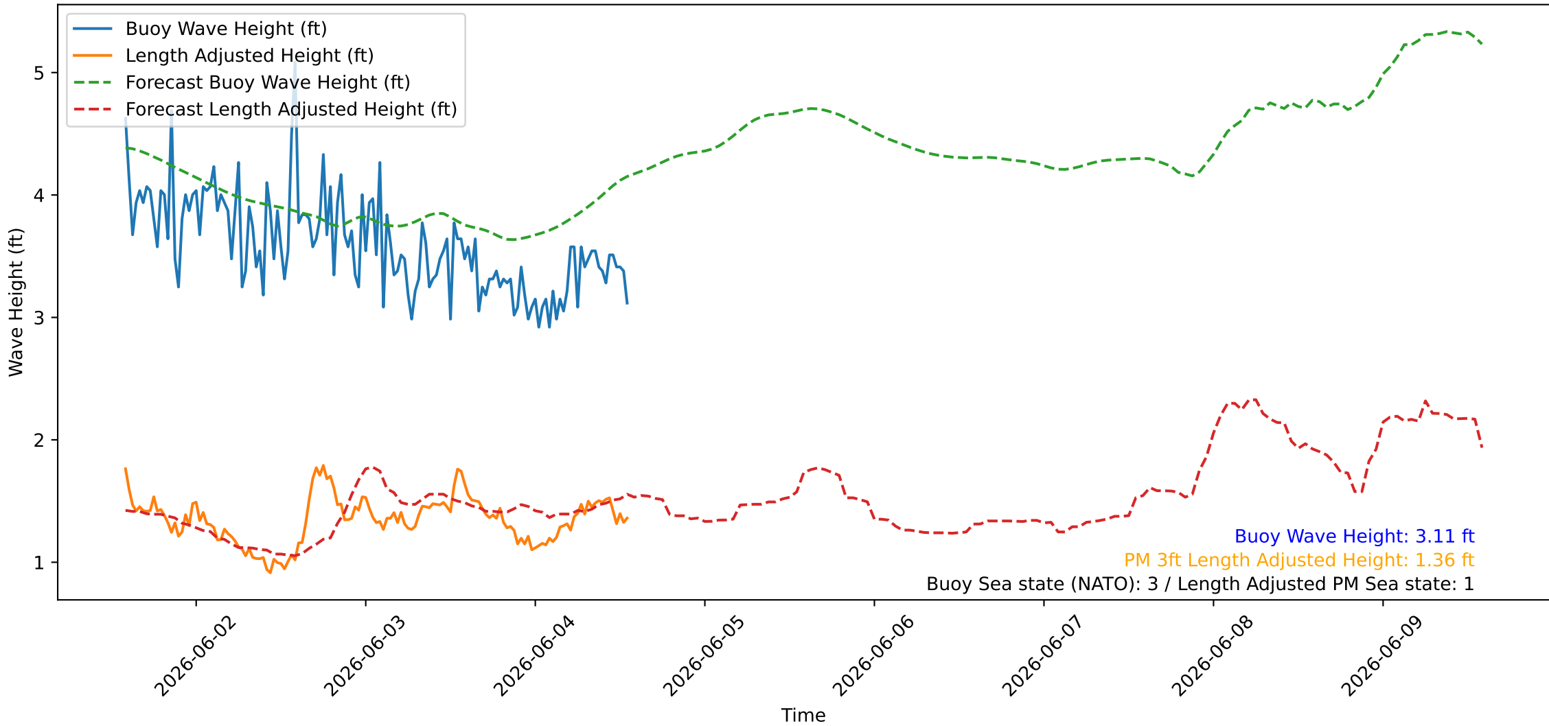
Wave Heights over Time for Oceanside Harbor at 2026-06-04 13:50:26
