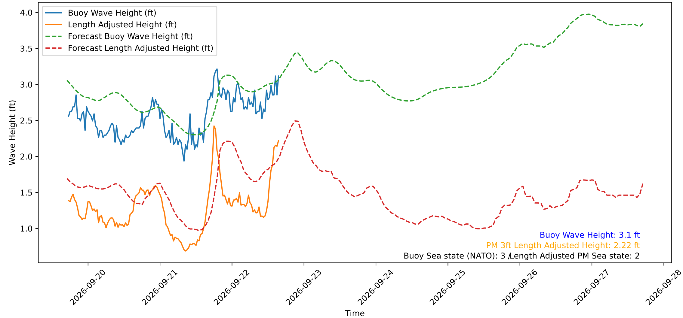
Wave Heights over Time for Green Beach at 2026-09-22 17:01:13
