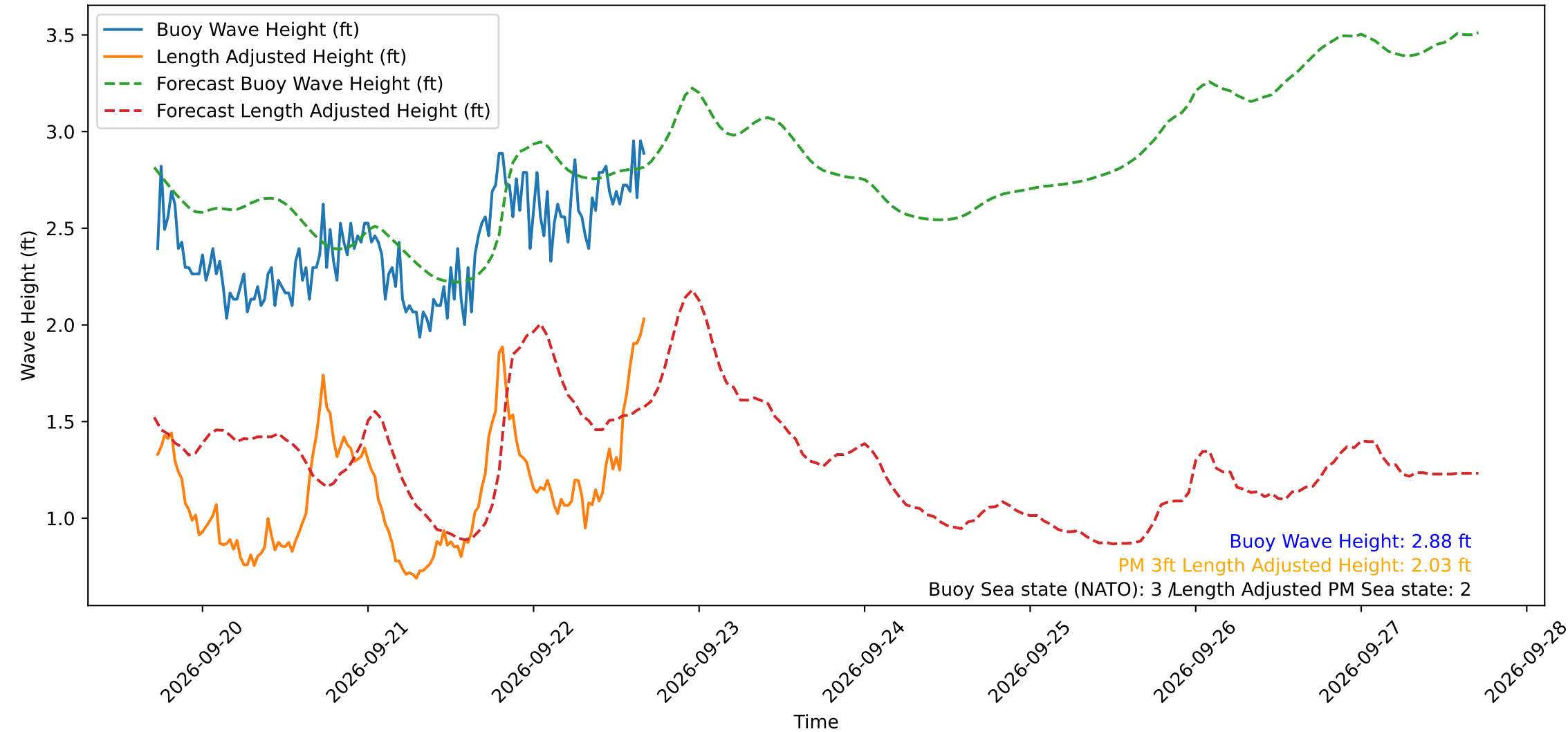
Wave Heights over Time for Red Beach at 2026-09-22 17:00:51
