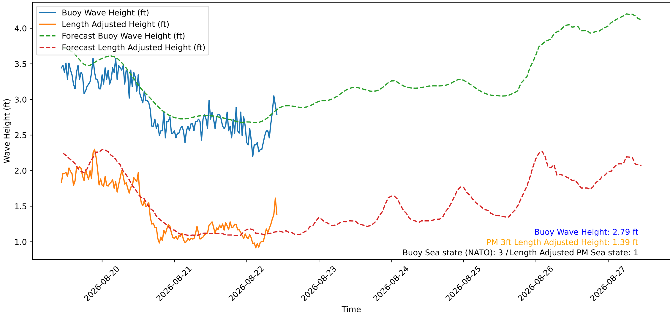
Wave Heights over Time for Oceanside Harbor at 2026-08-22 10:40:29
