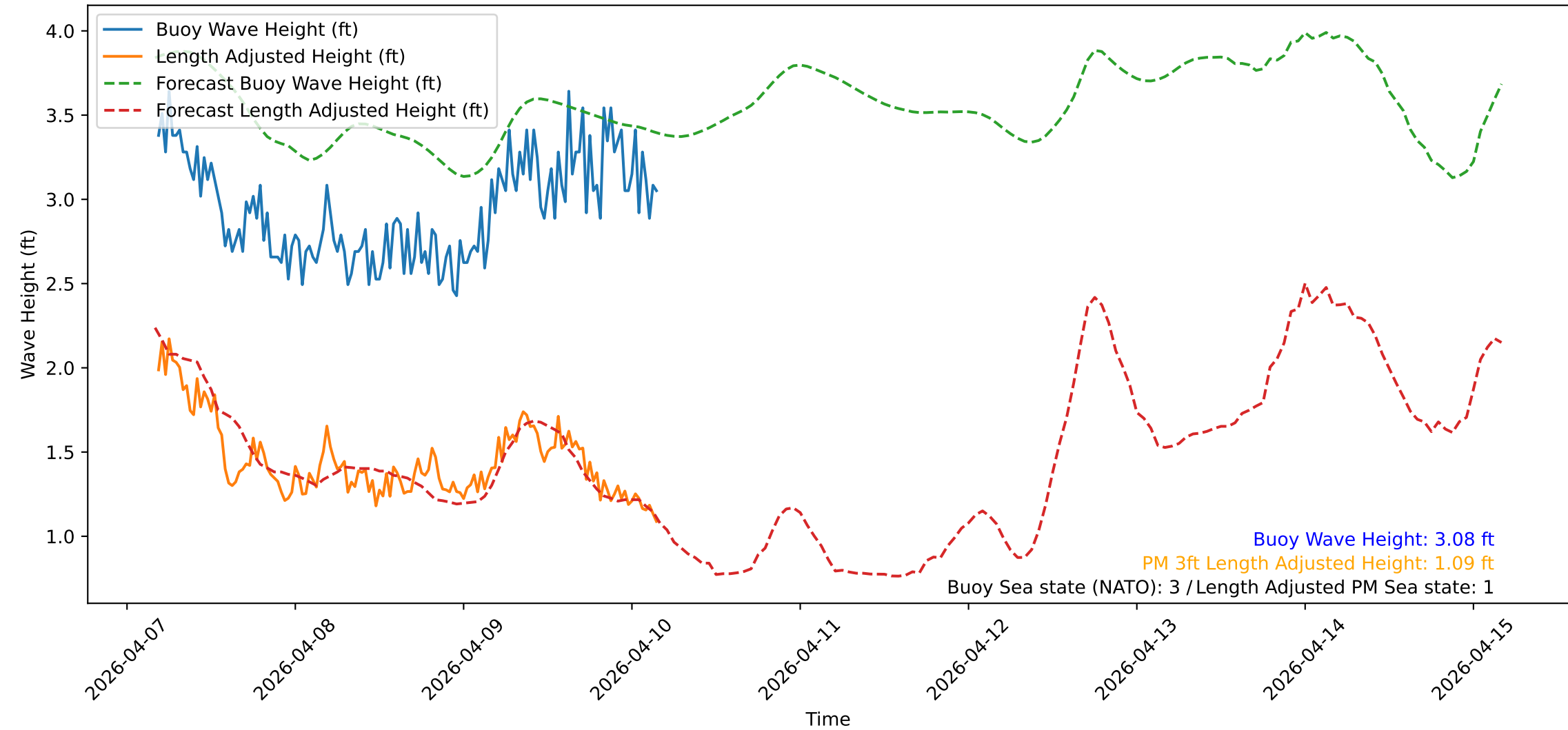
Wave Heights over Time for Oceanside Harbor at 2026-04-10 04:20:31
