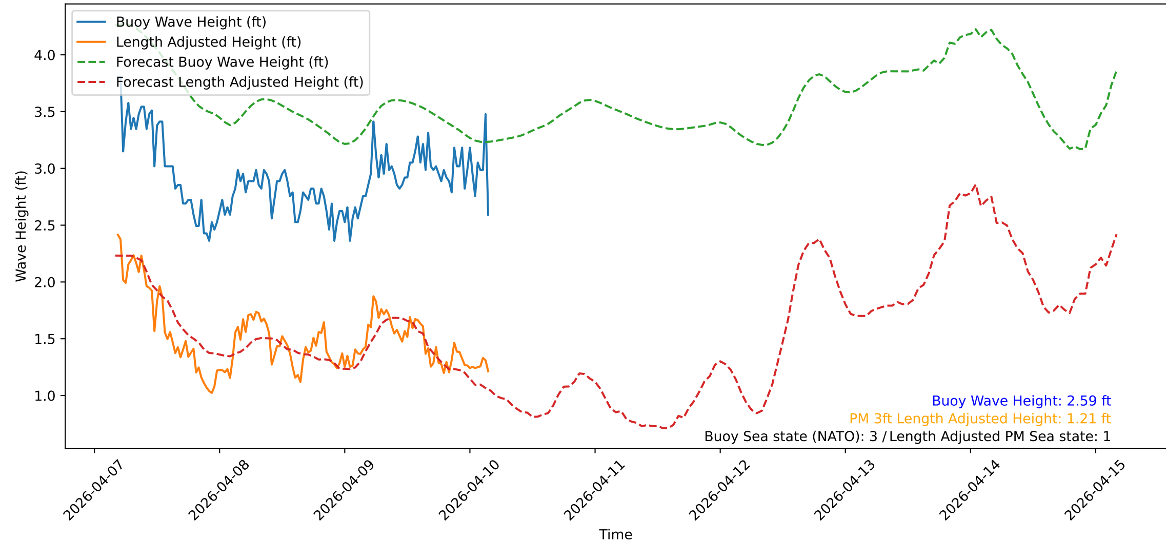
Wave Heights over Time for Green Beach at 2026-04-10 04:21:14
