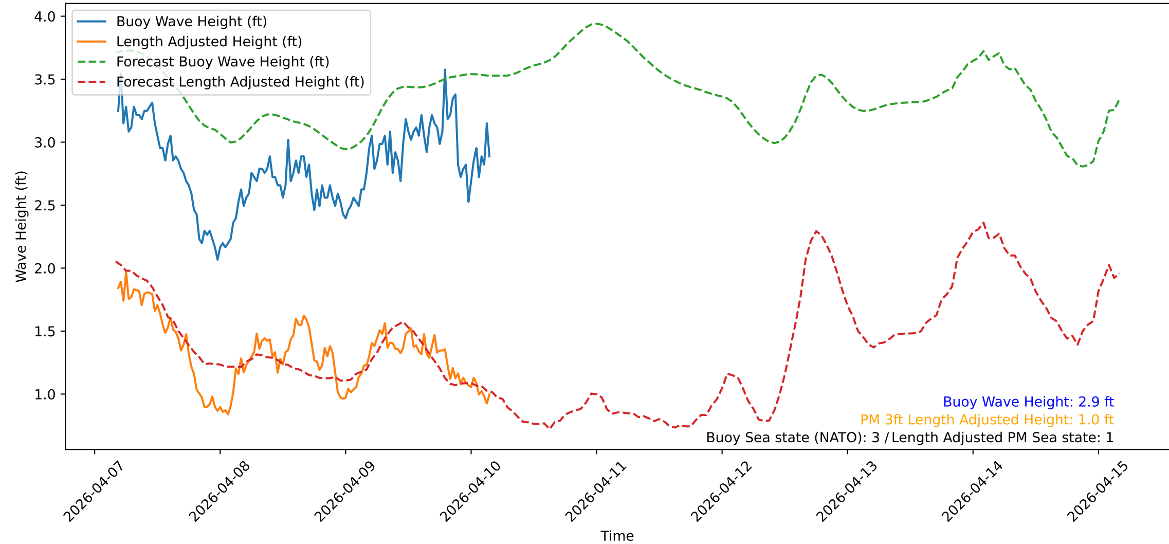
Wave Heights over Time for Red Beach at 2026-04-10 04:20:51
