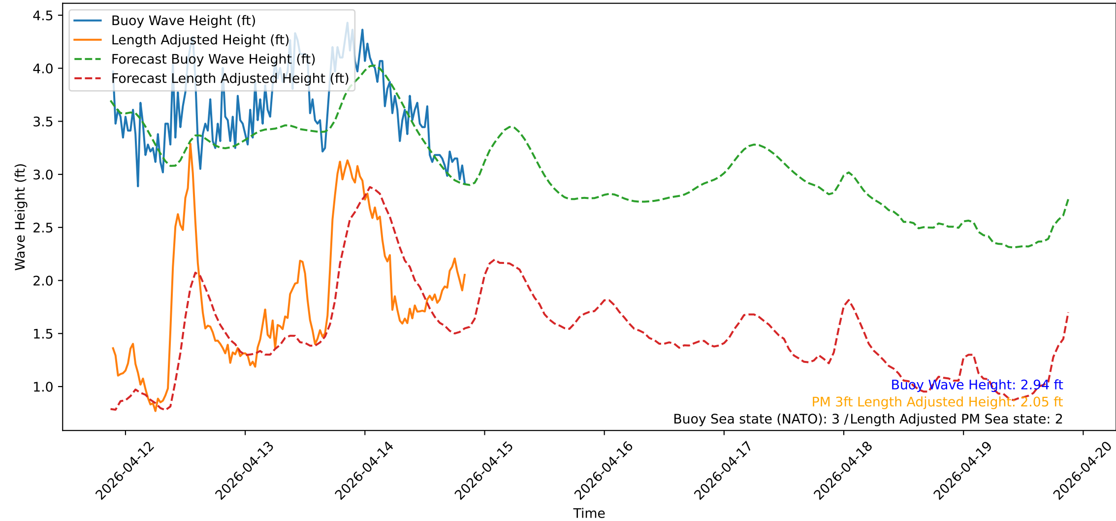
Wave Heights over Time for Red Beach at 2026-04-14 21:00:50
