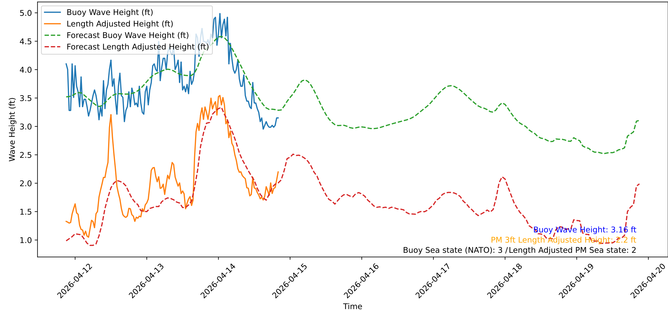
Wave Heights over Time for Green Beach at 2026-04-14 21:01:12
