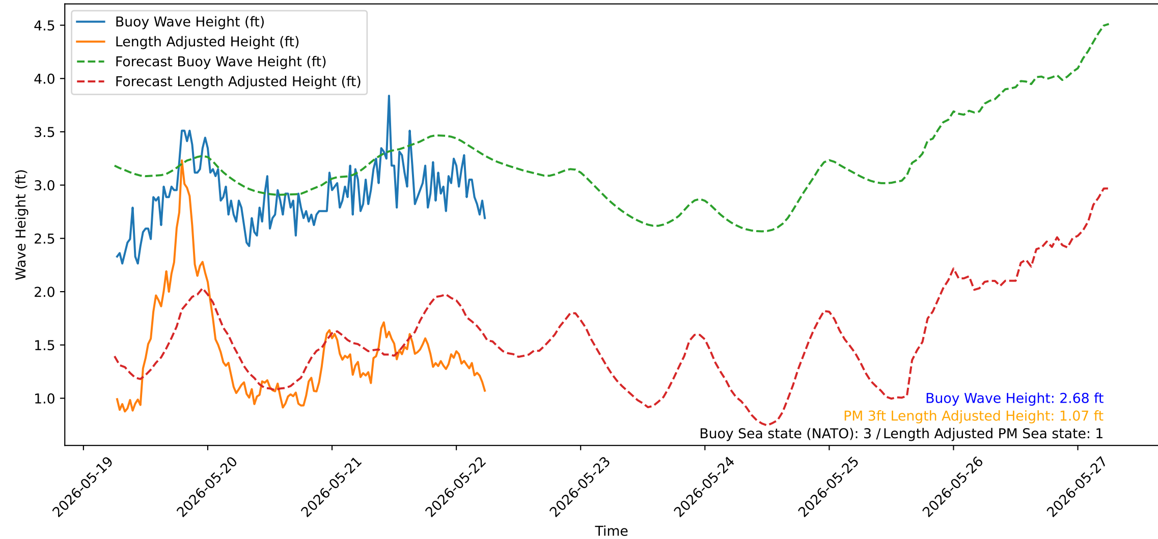
Wave Heights over Time for Oceanside Harbor at 2026-05-22 06:20:32
