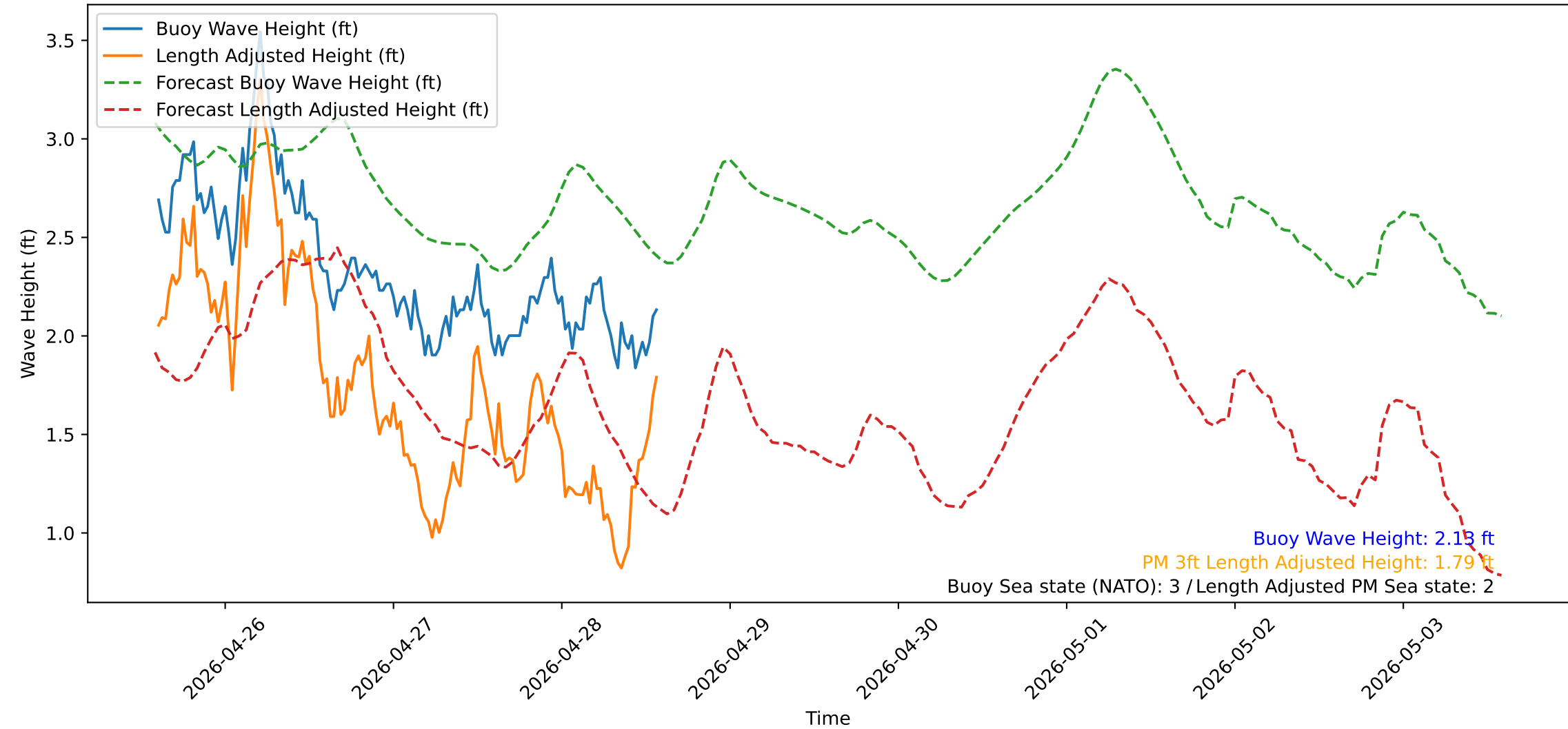
Wave Heights over Time for Red Beach at 2026-04-28 14:20:52
