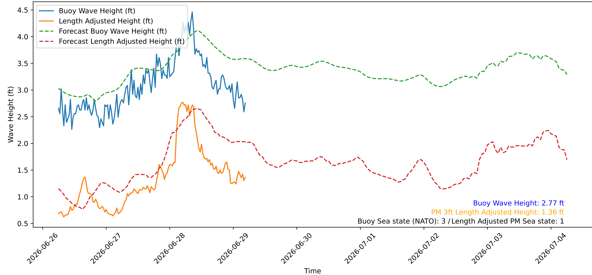
Wave Heights over Time for Red Beach at 2026-06-29 05:30:45
