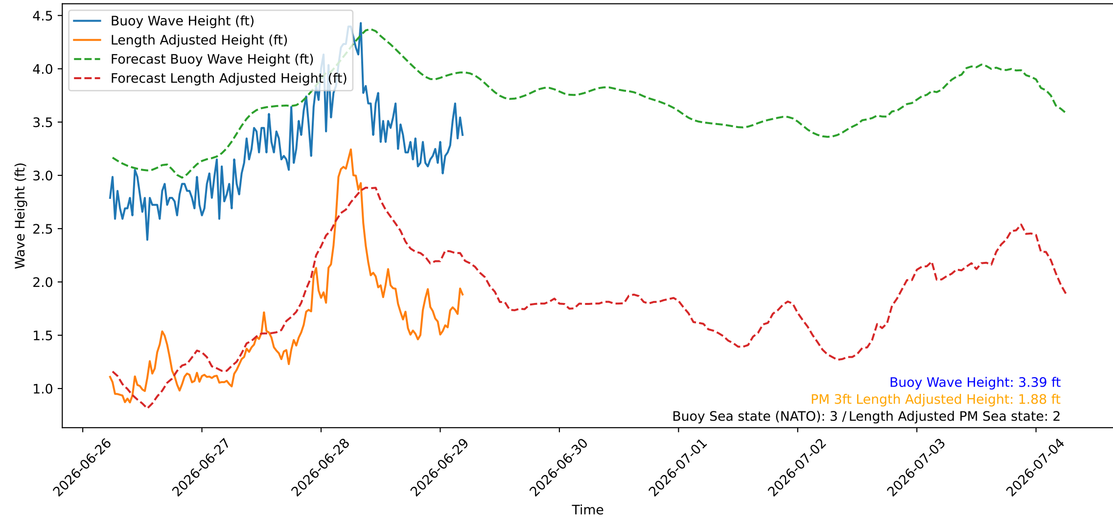
Wave Heights over Time for Oceanside Harbor at 2026-06-29 05:30:26
