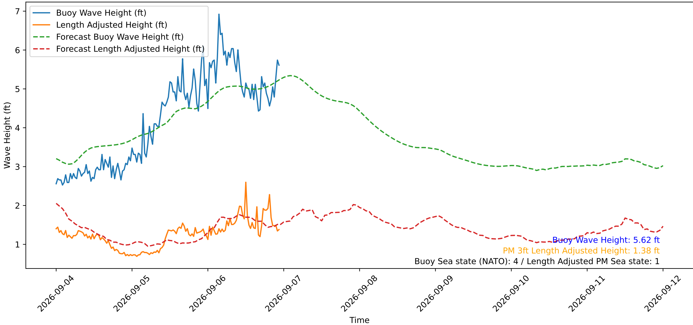
Wave Heights over Time for Red Beach at 2026-09-06 23:30:49
