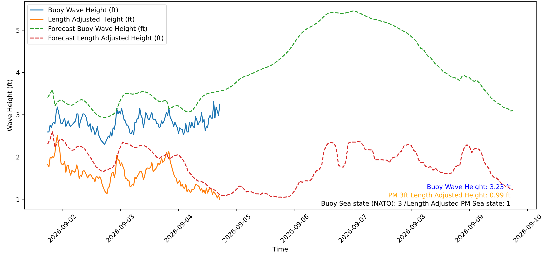
Wave Heights over Time for Red Beach at 2026-09-04 17:40:50
