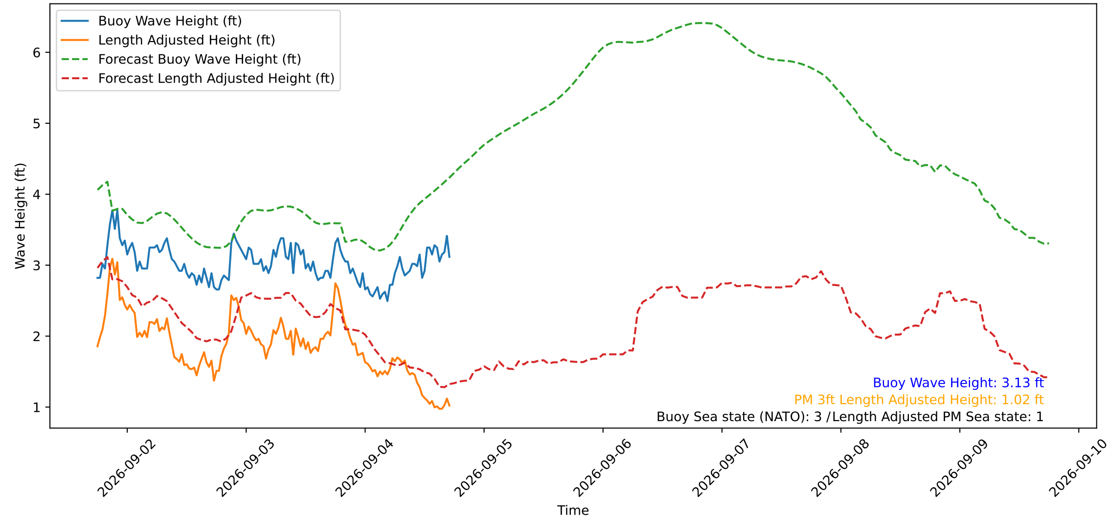
Wave Heights over Time for Green Beach at 2026-09-04 17:41:12
