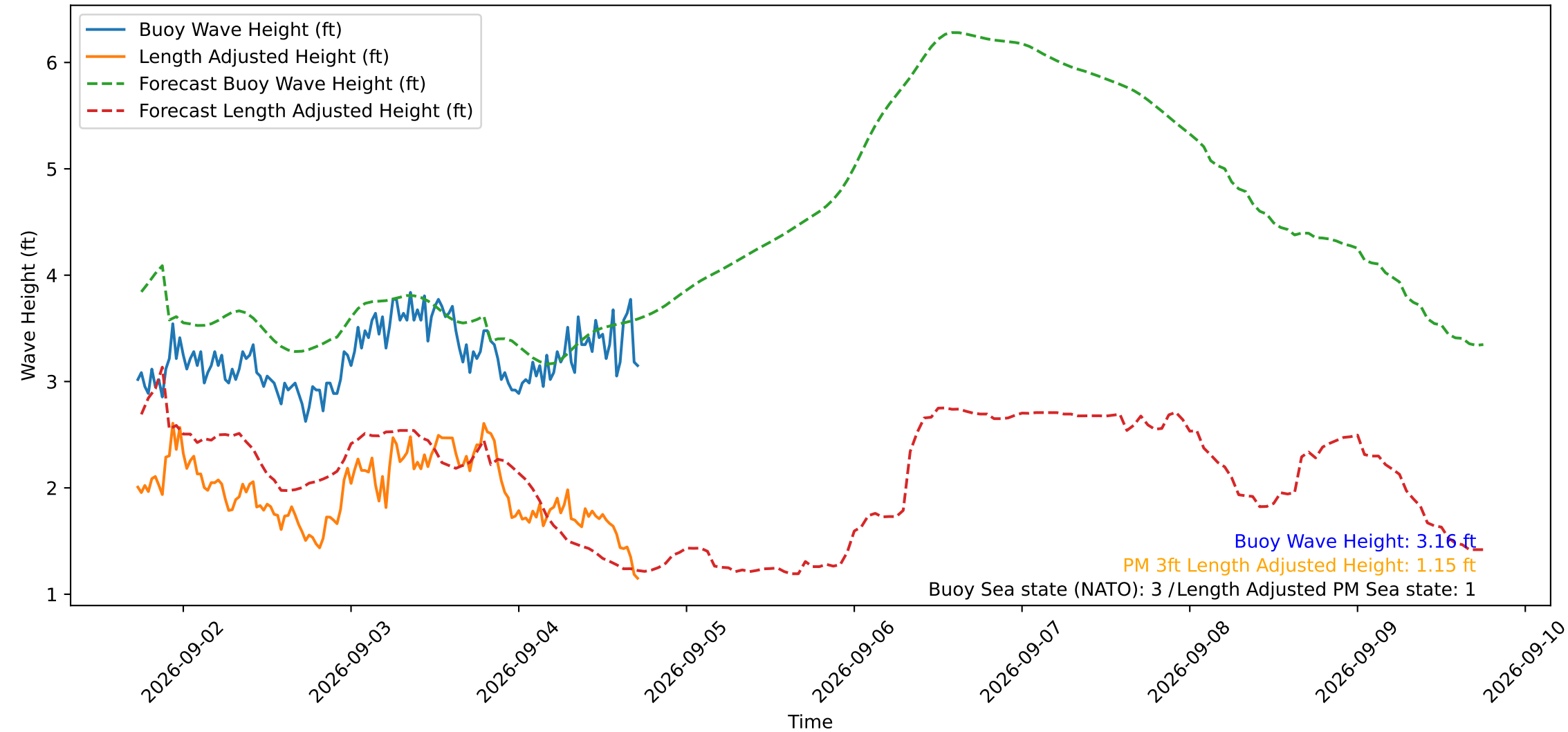
Wave Heights over Time for Oceanside Harbor at 2026-09-04 17:40:30
