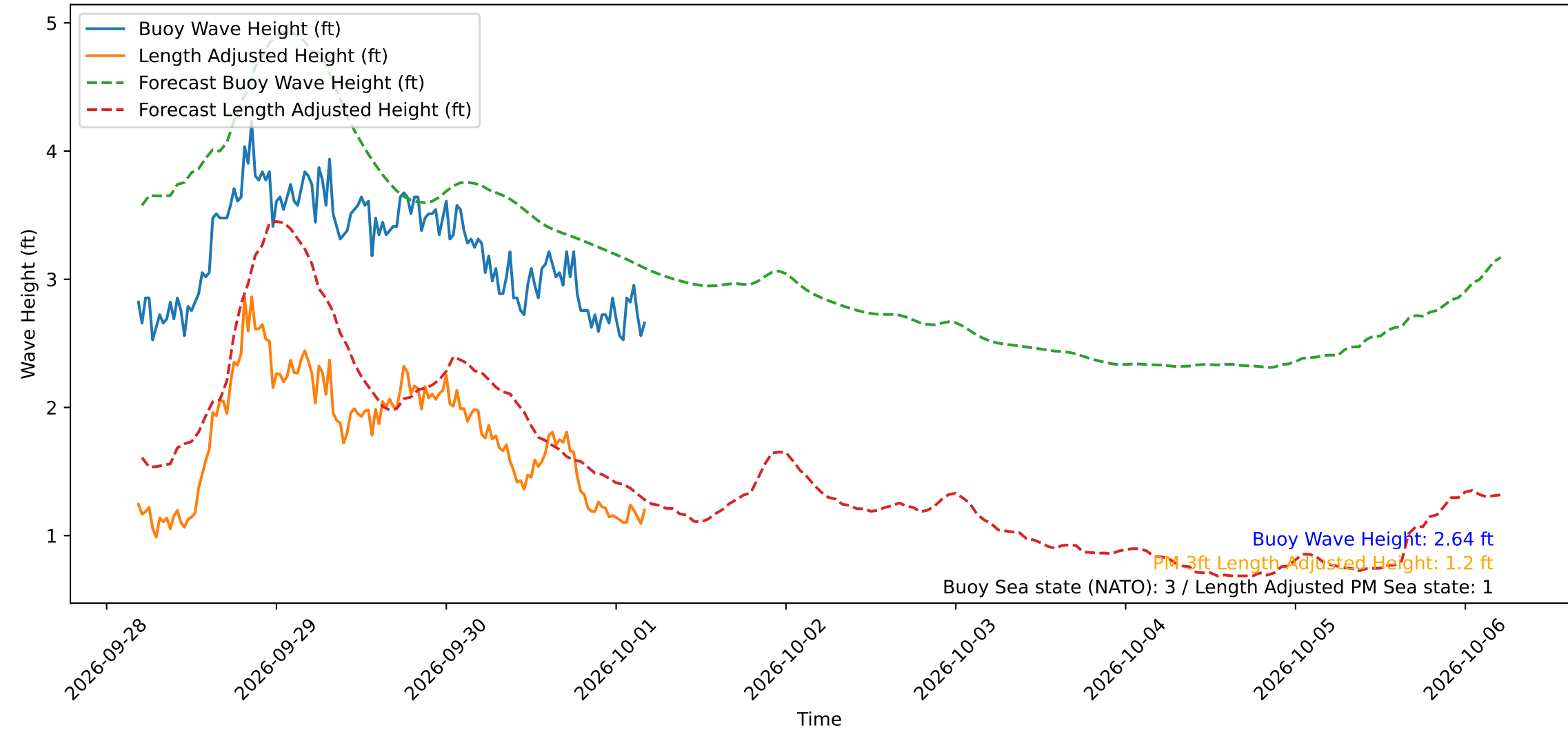
Wave Heights over Time for Oceanside Harbor at 2026-10-01 04:30:30
