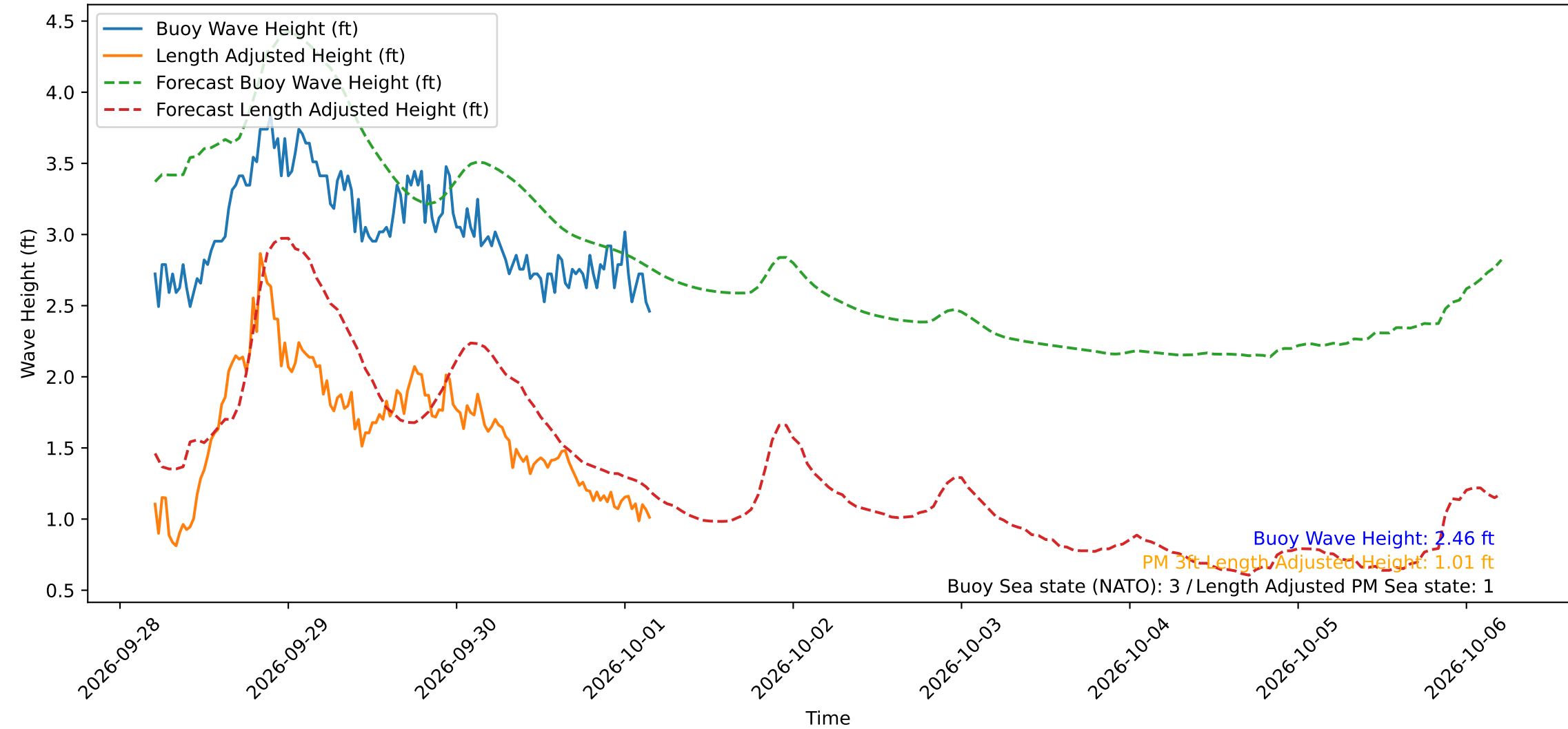
Wave Heights over Time for Red Beach at 2026-10-01 04:30:50
