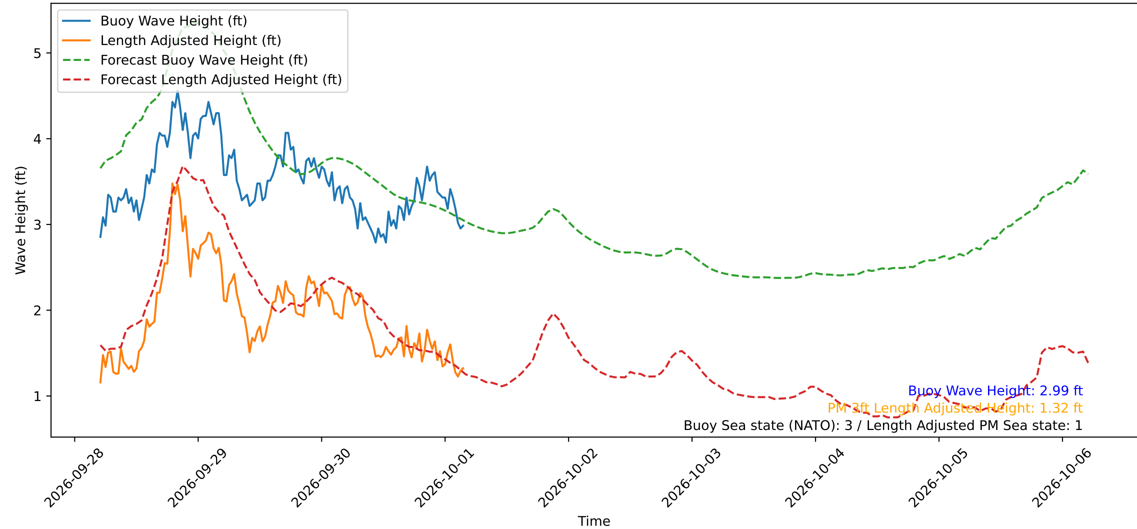
Wave Heights over Time for Green Beach at 2026-10-01 04:31:12
