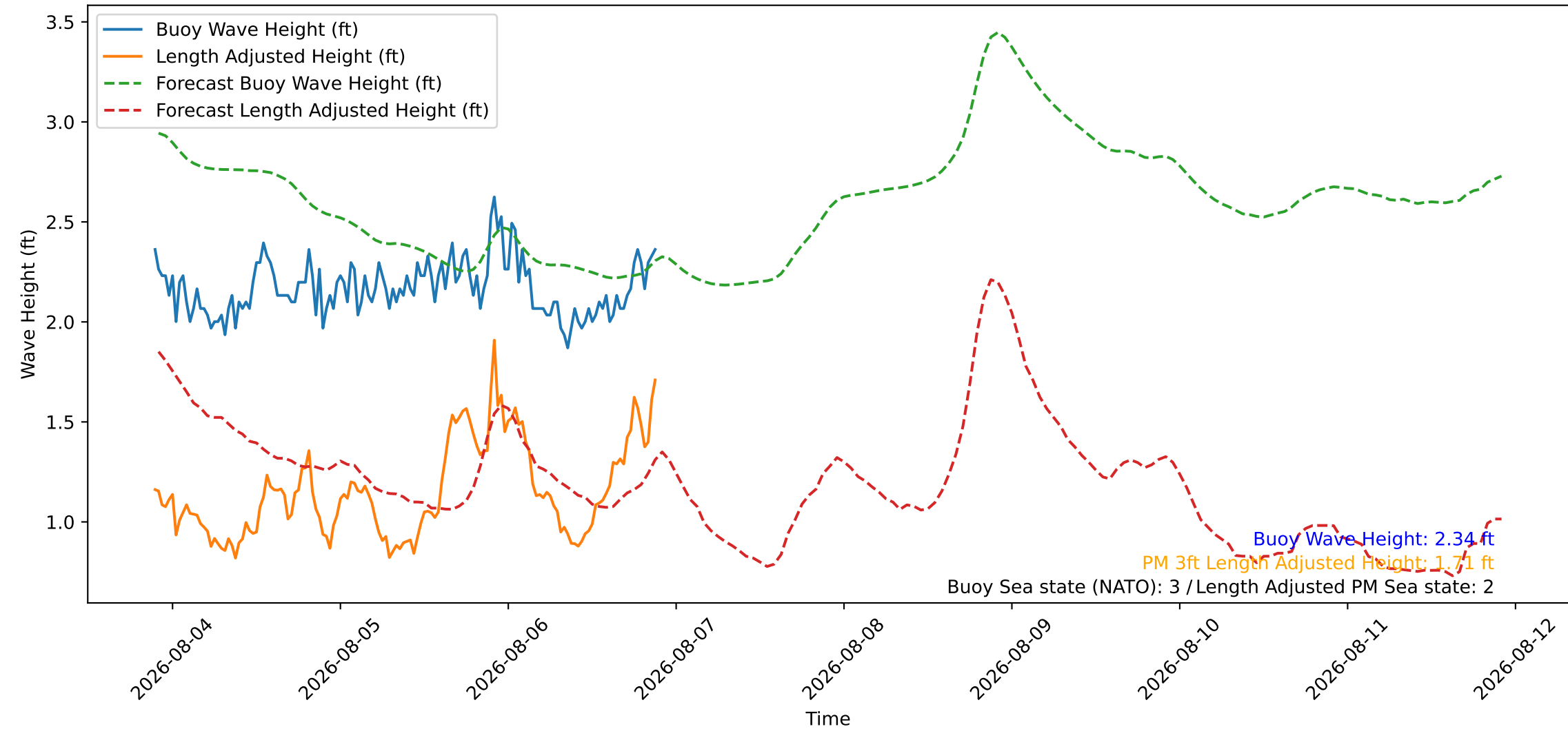
Wave Heights over Time for Green Beach at 2026-08-06 21:41:08
