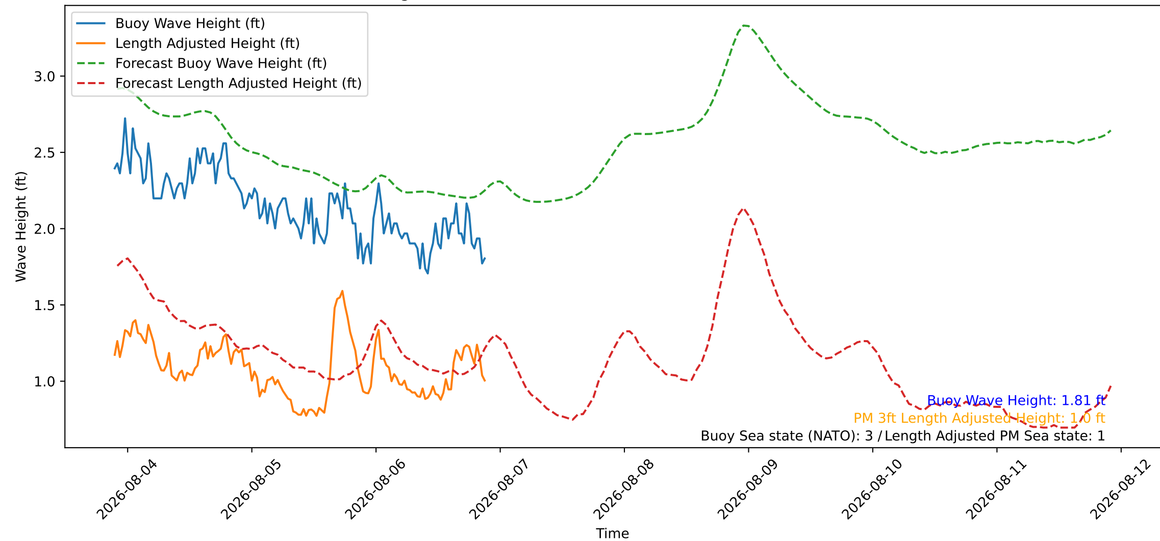
Wave Heights over Time for Oceanside Harbor at 2026-08-06 21:40:26
