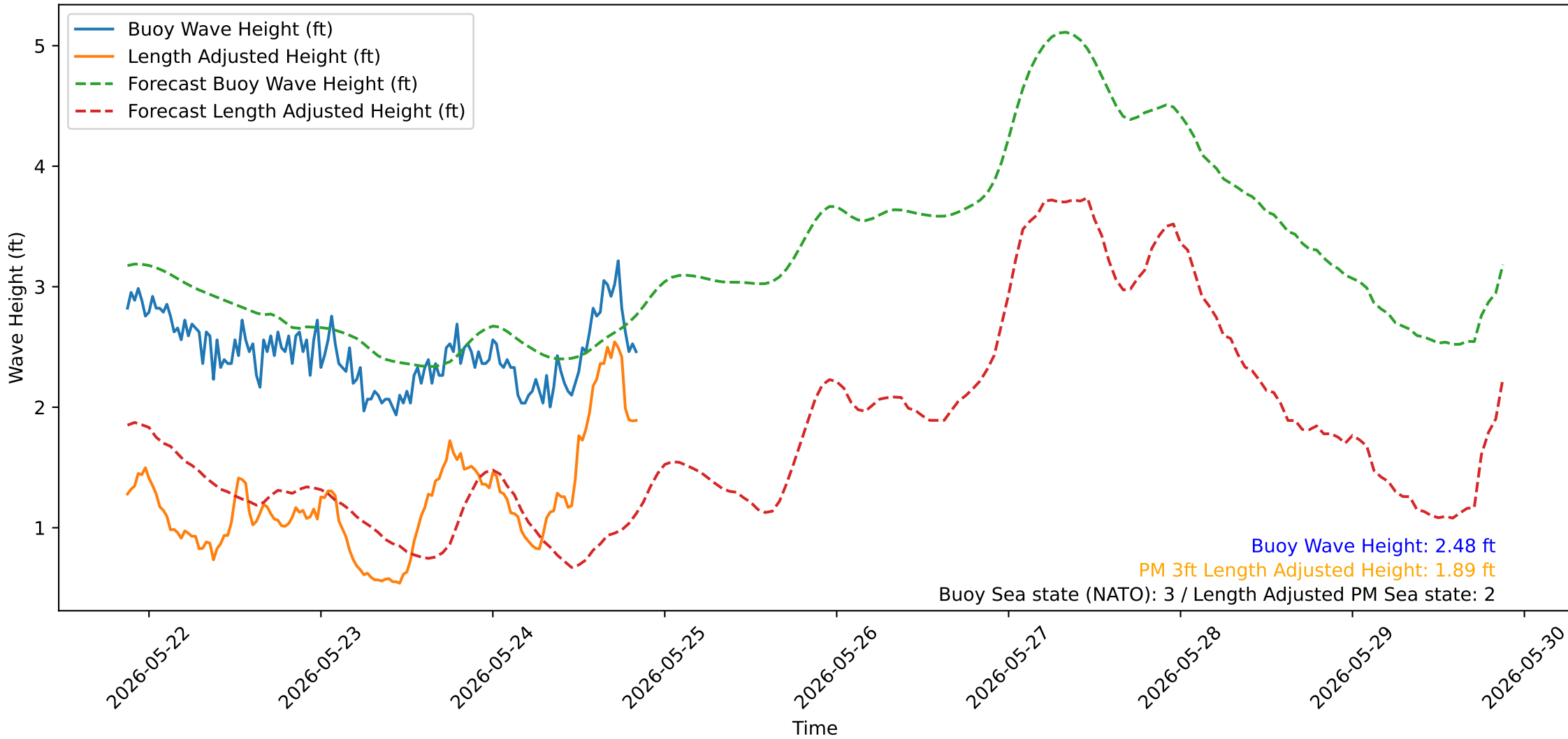
Wave Heights over Time for Red Beach at 2026-05-24 20:40:52
