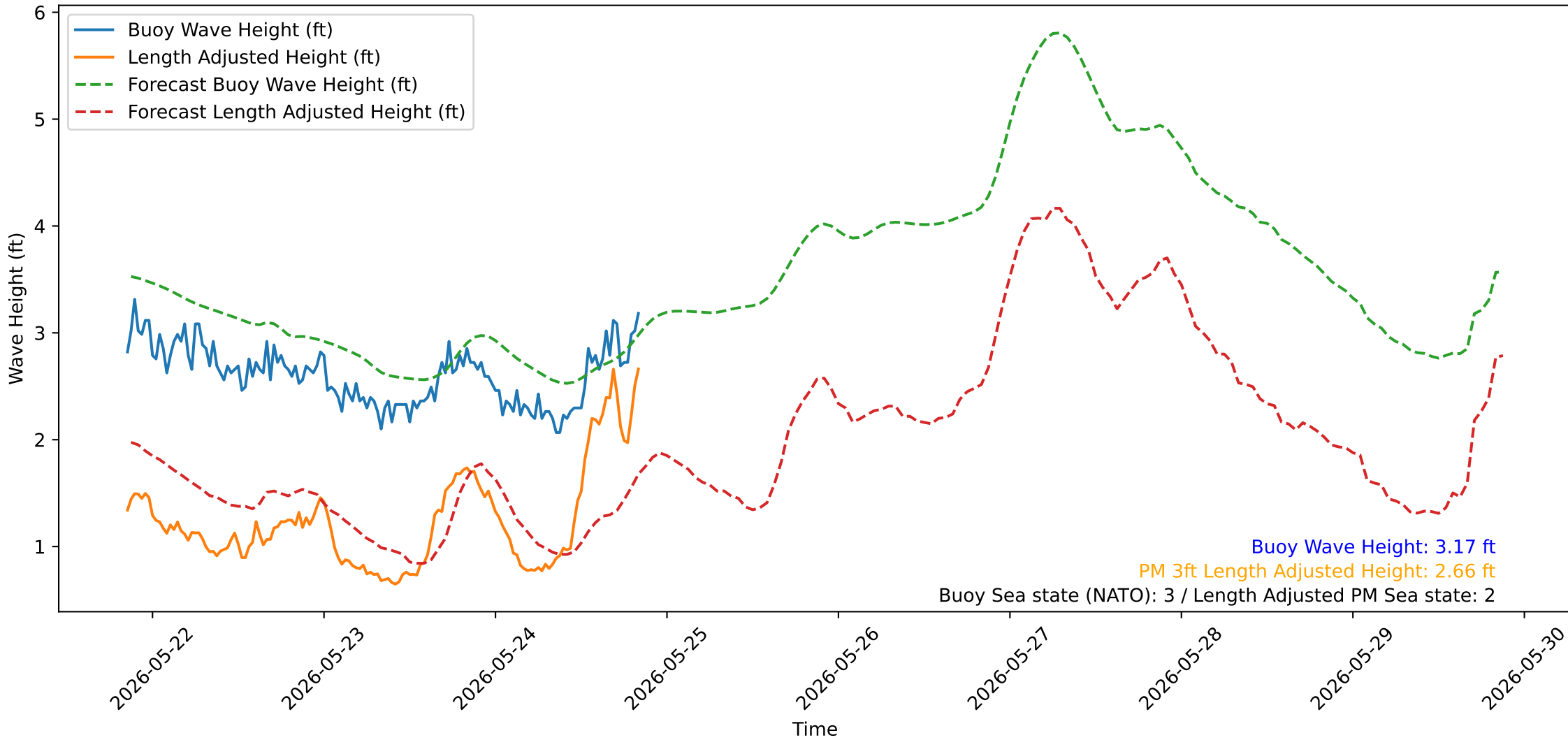
Wave Heights over Time for Green Beach at 2026-05-24 20:41:15
