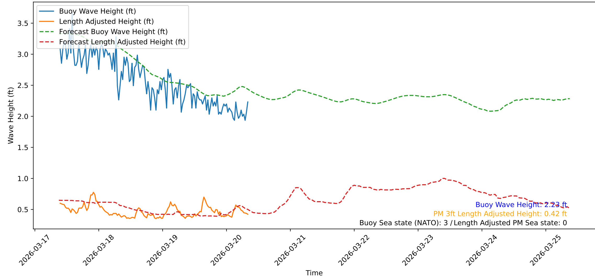
Wave Heights over Time for Red Beach at 2026-03-20 09:00:48
