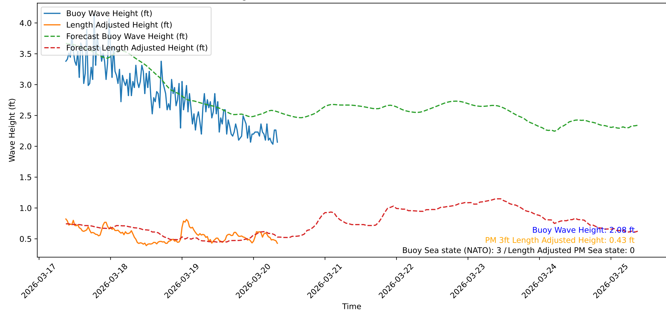
Wave Heights over Time for Green Beach at 2026-03-20 09:01:10
