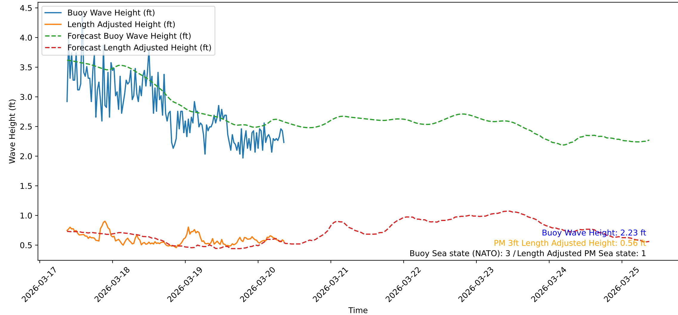
Wave Heights over Time for Oceanside Harbor at 2026-03-20 09:00:31
