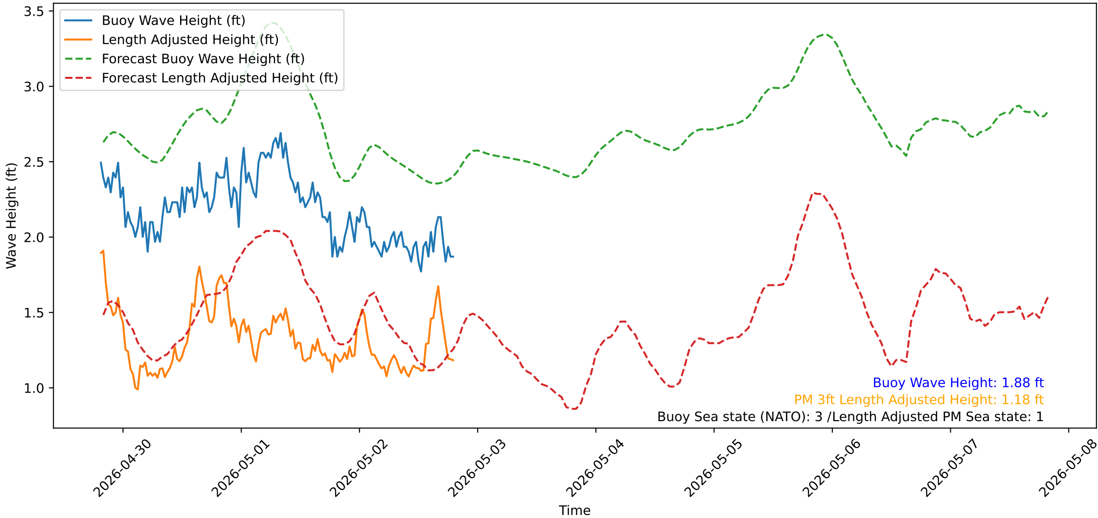
Wave Heights over Time for Oceanside Harbor at 2026-05-02 19:40:31
