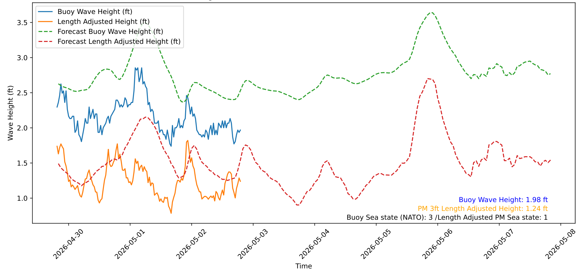
Wave Heights over Time for Green Beach at 2026-05-02 19:41:13
