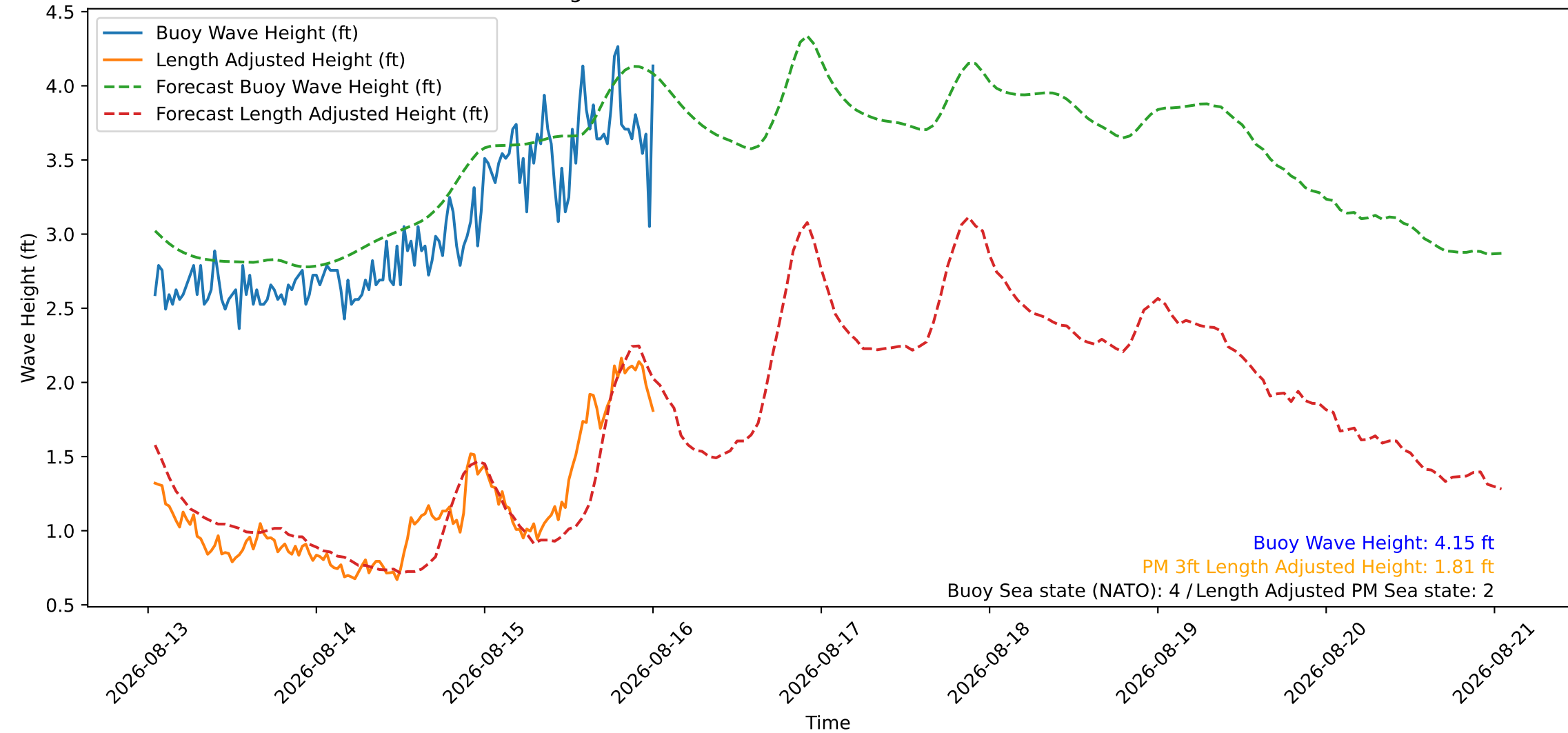
Wave Heights over Time for Green Beach at 2026-08-16 00:51:10
