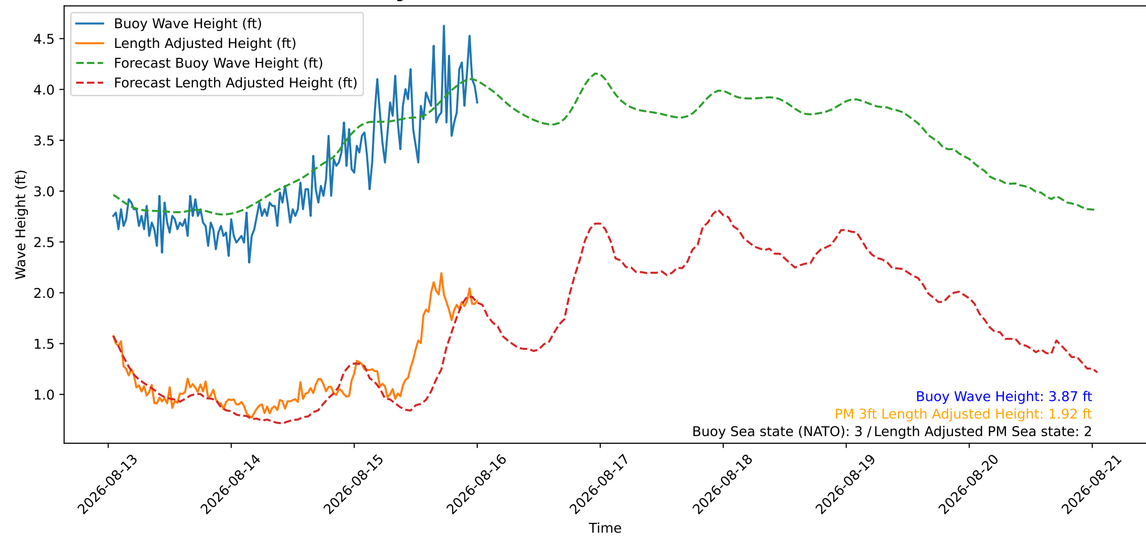
Wave Heights over Time for Oceanside Harbor at 2026-08-16 00:50:26
