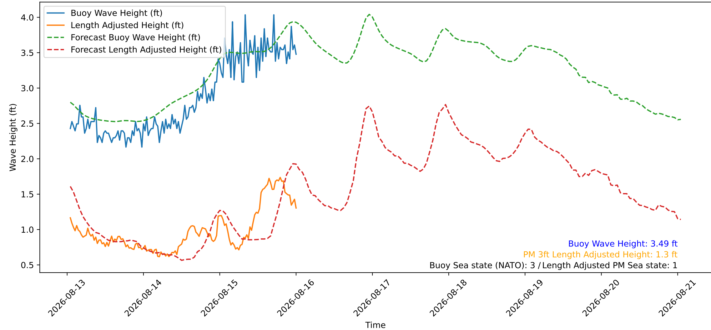
Wave Heights over Time for Red Beach at 2026-08-16 00:50:47
