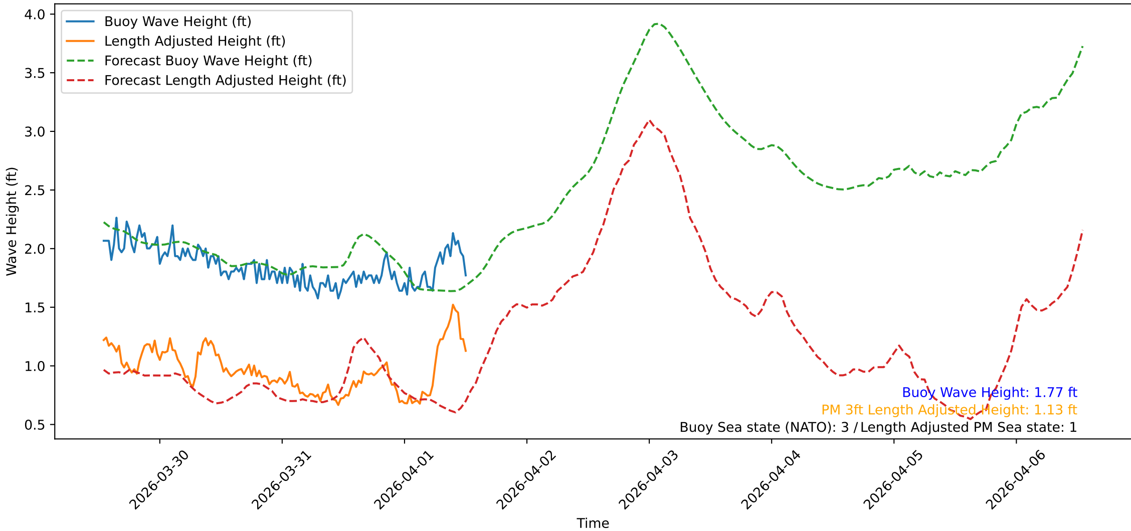
Wave Heights over Time for Oceanside Harbor at 2026-04-01 13:10:31
