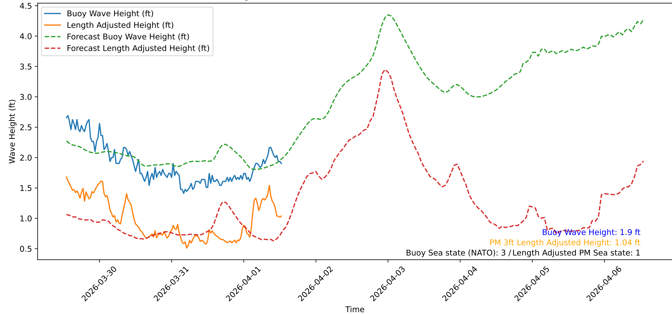
Wave Heights over Time for Green Beach at 2026-04-01 13:11:10
