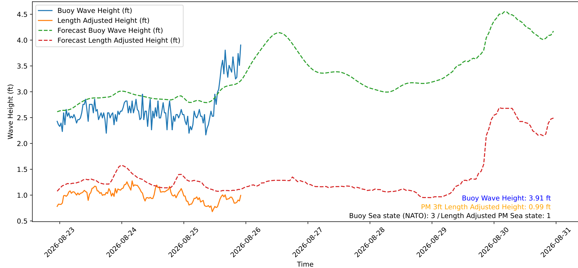
Wave Heights over Time for Red Beach at 2026-08-25 22:50:50
