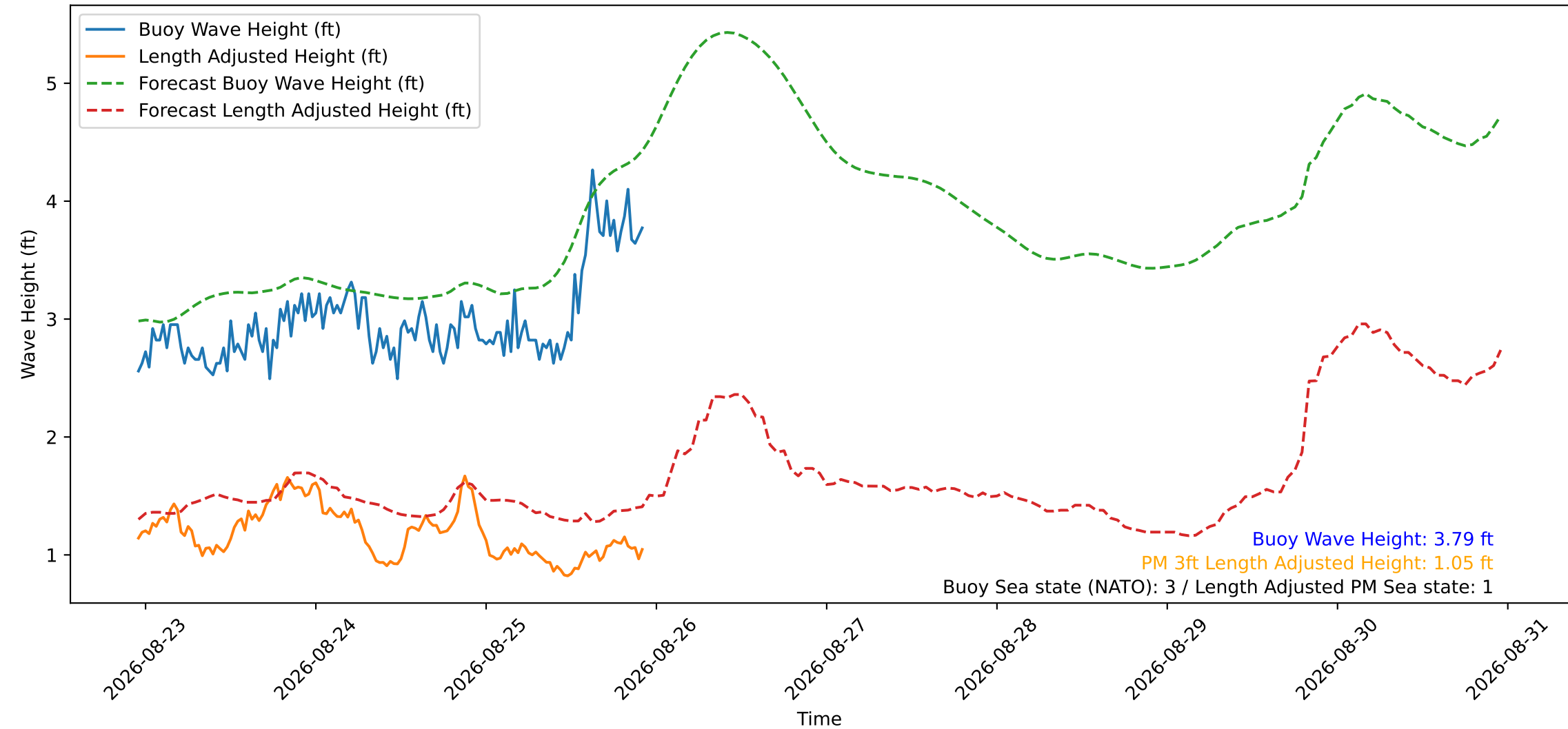
Wave Heights over Time for Green Beach at 2026-08-25 22:51:13
