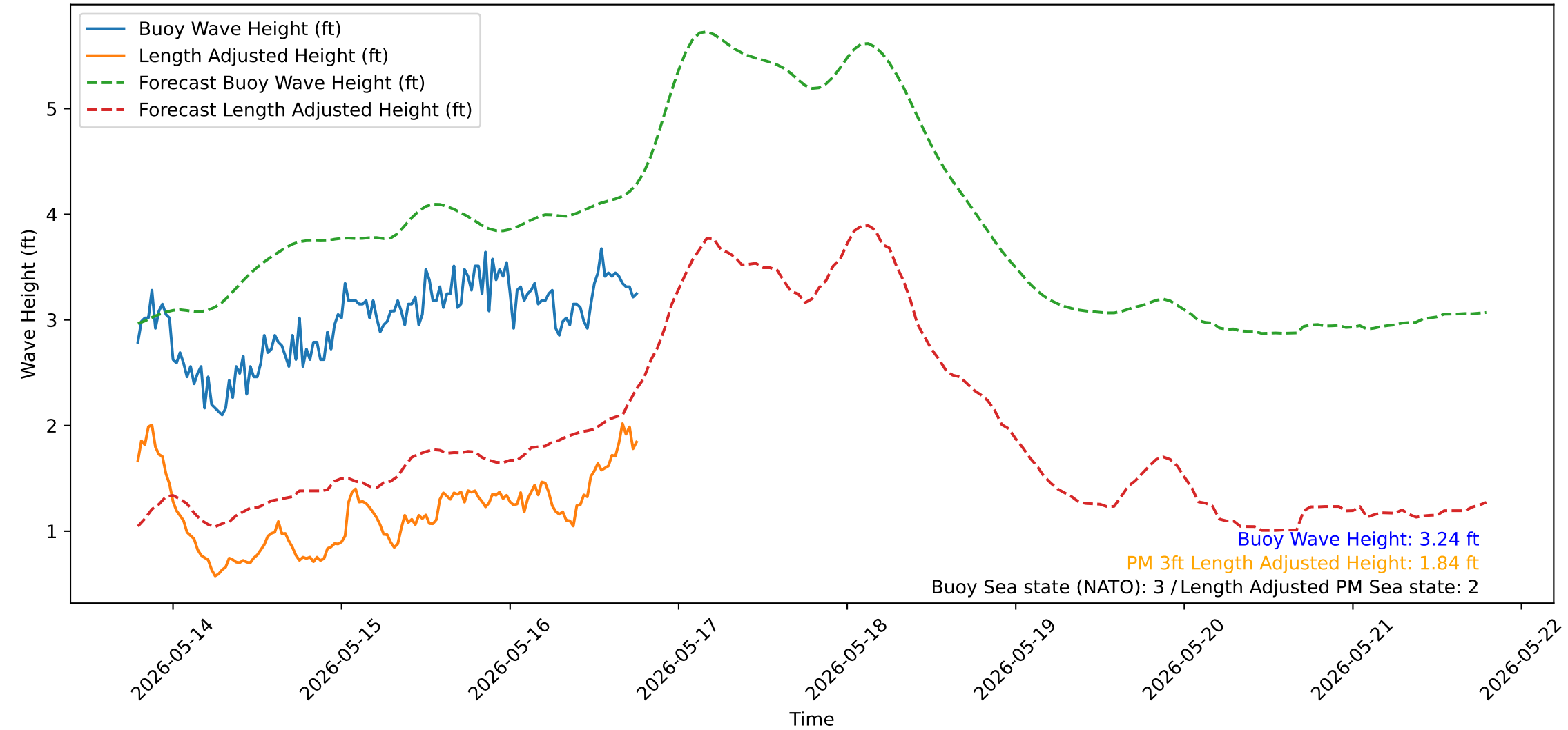
Wave Heights over Time for Green Beach at 2026-05-16 18:51:16
