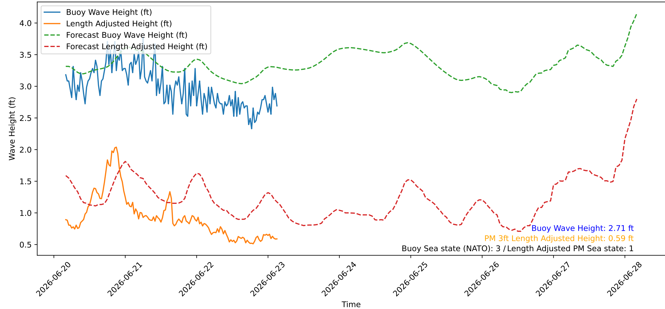
Wave Heights over Time for Red Beach at 2026-06-23 03:50:47
