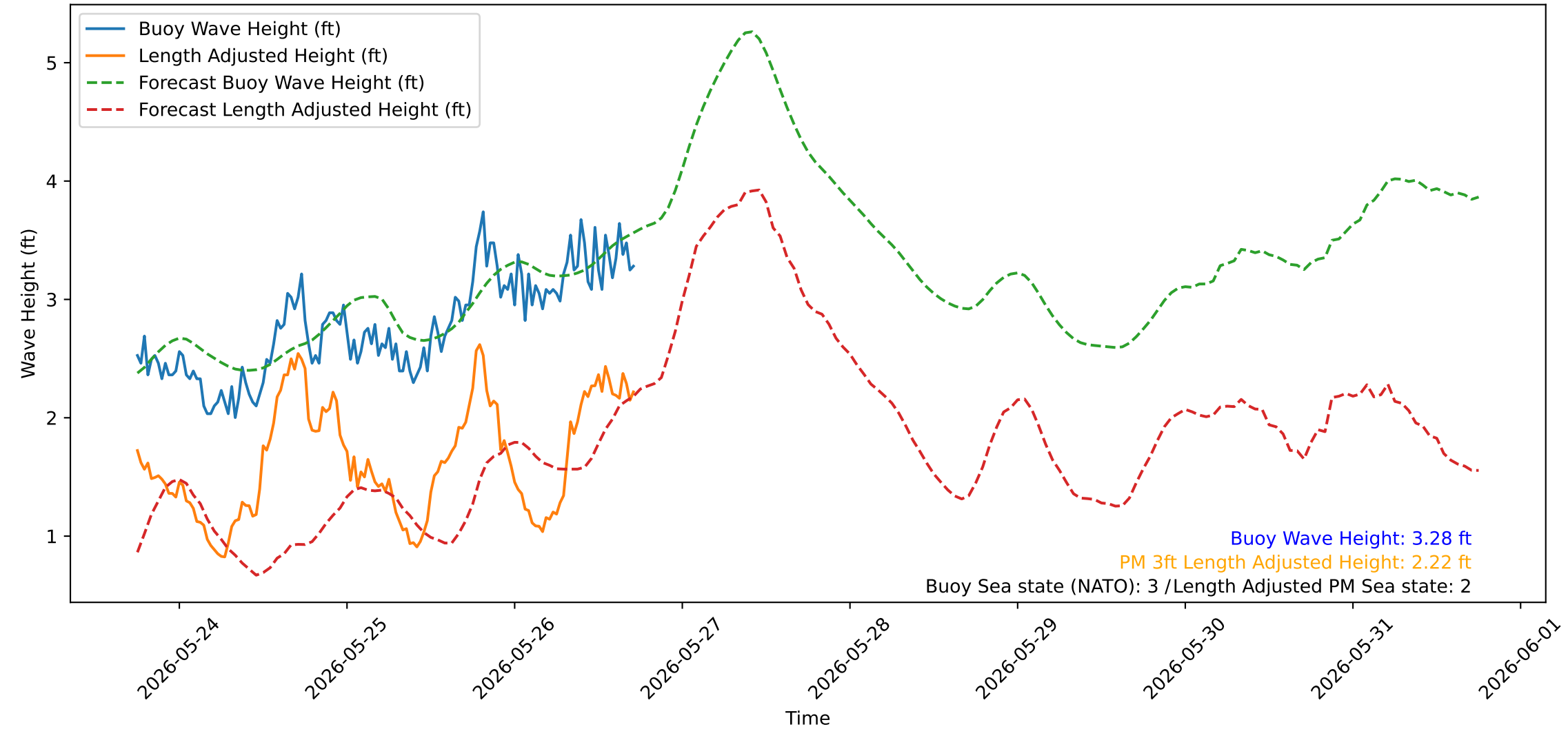
Wave Heights over Time for Red Beach at 2026-05-26 17:40:47
