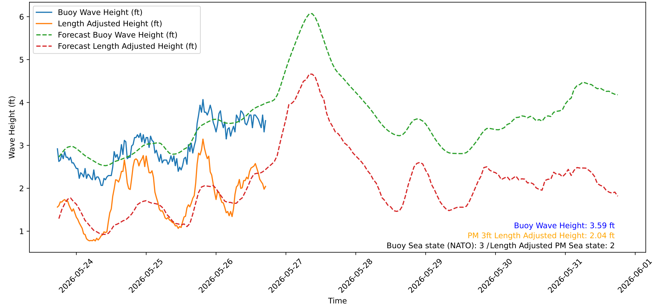
Wave Heights over Time for Green Beach at 2026-05-26 17:41:09
