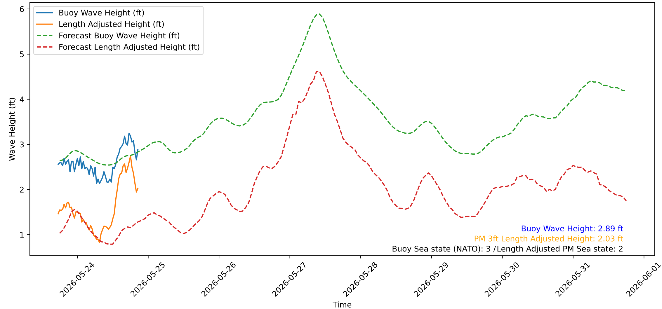
Wave Heights over Time for Oceanside Harbor at 2026-05-26 17:40:27
