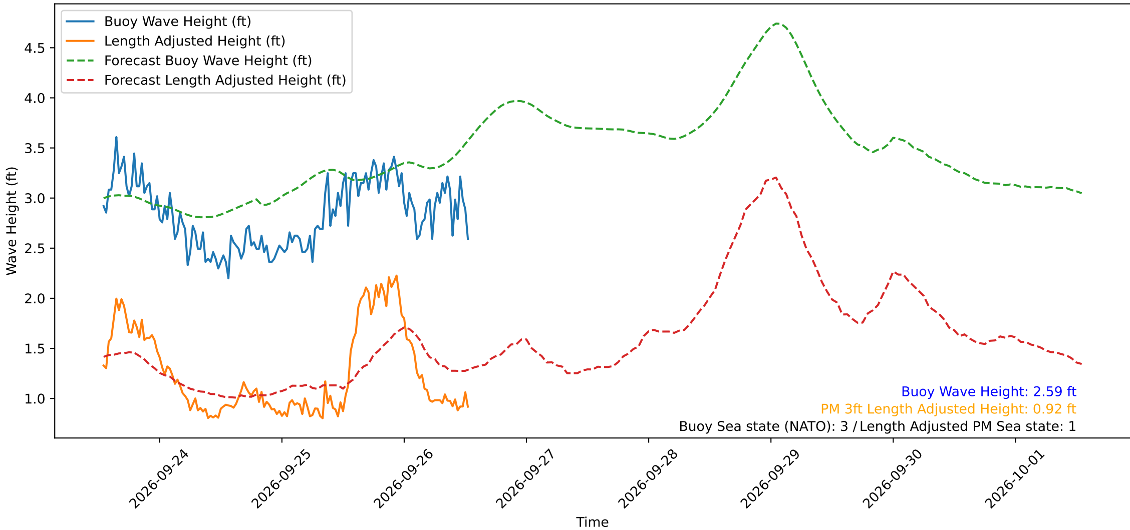
Wave Heights over Time for Oceanside Harbor at 2026-09-26 13:00:30
