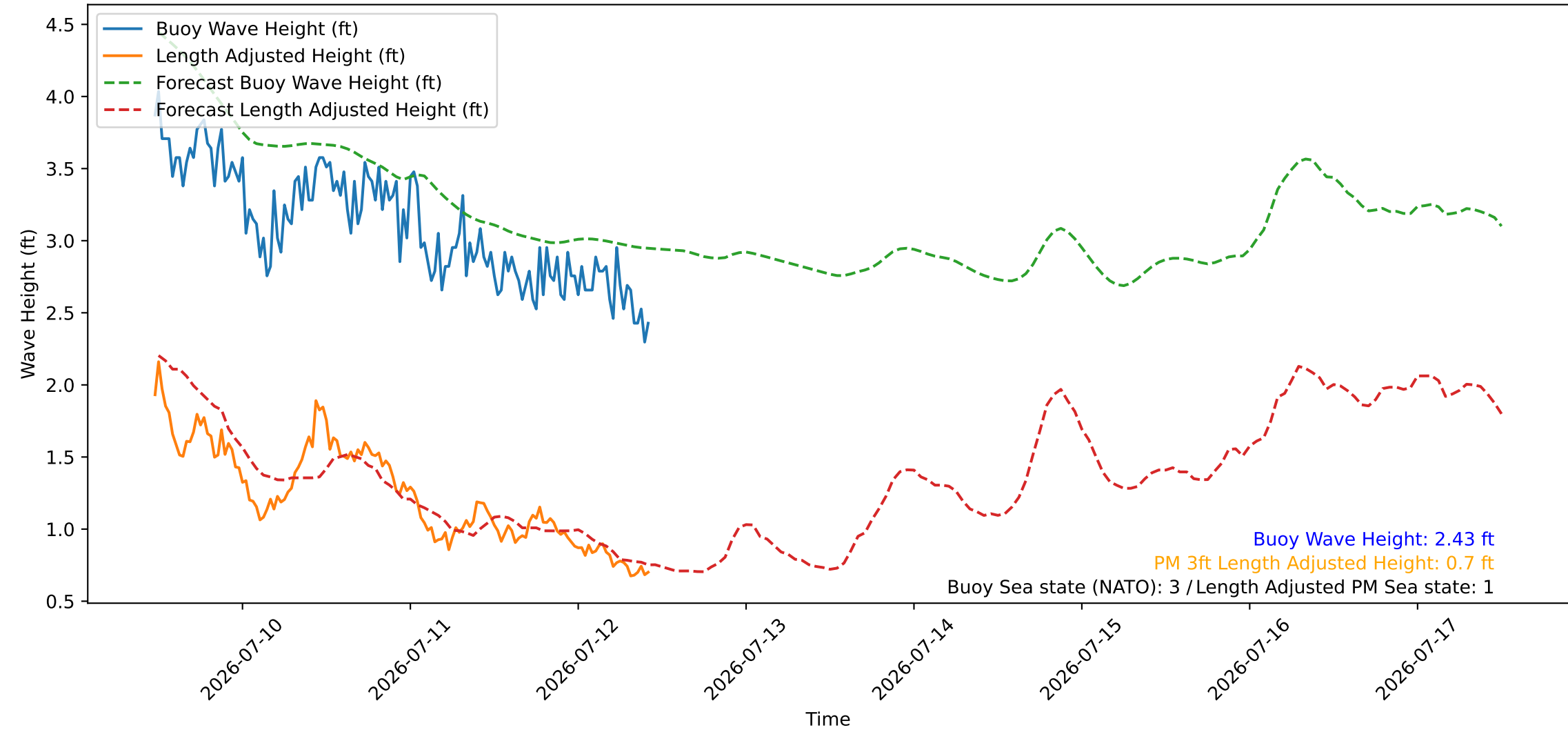
Wave Heights over Time for Green Beach at 2026-07-12 11:31:09
