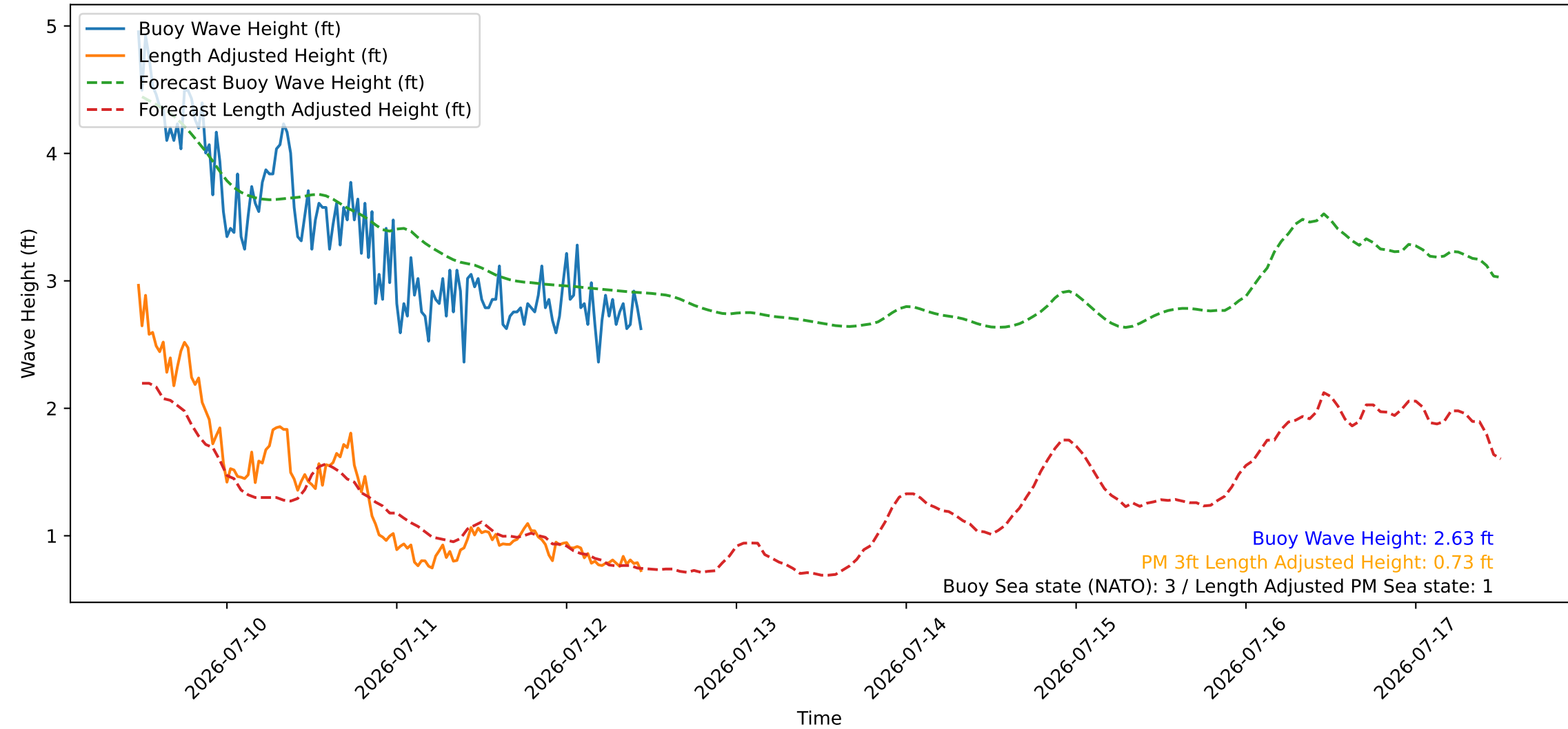
Wave Heights over Time for Oceanside Harbor at 2026-07-12 11:30:27
