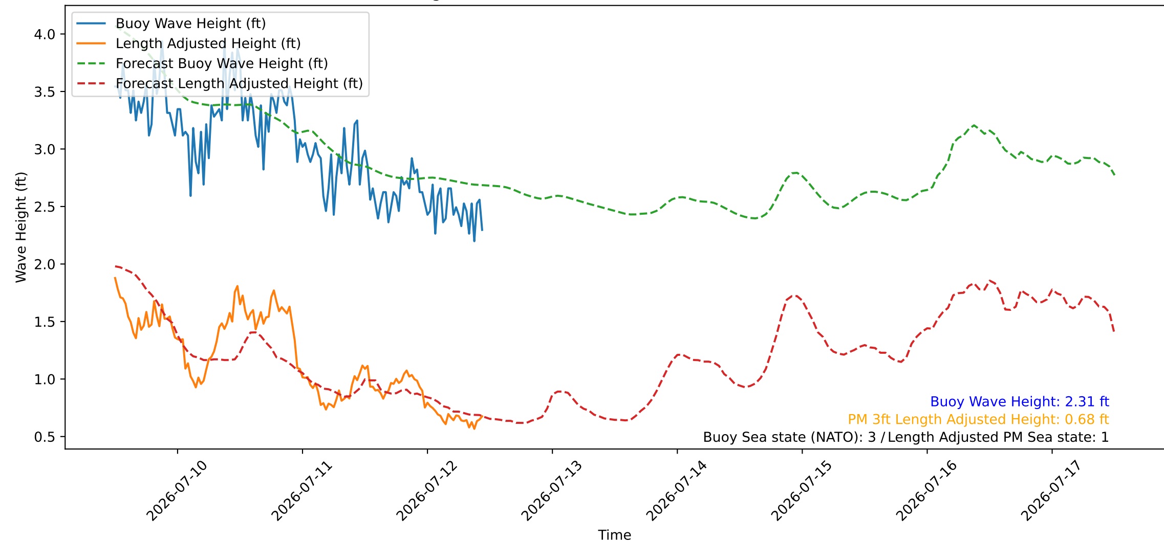
Wave Heights over Time for Red Beach at 2026-07-12 11:30:46
