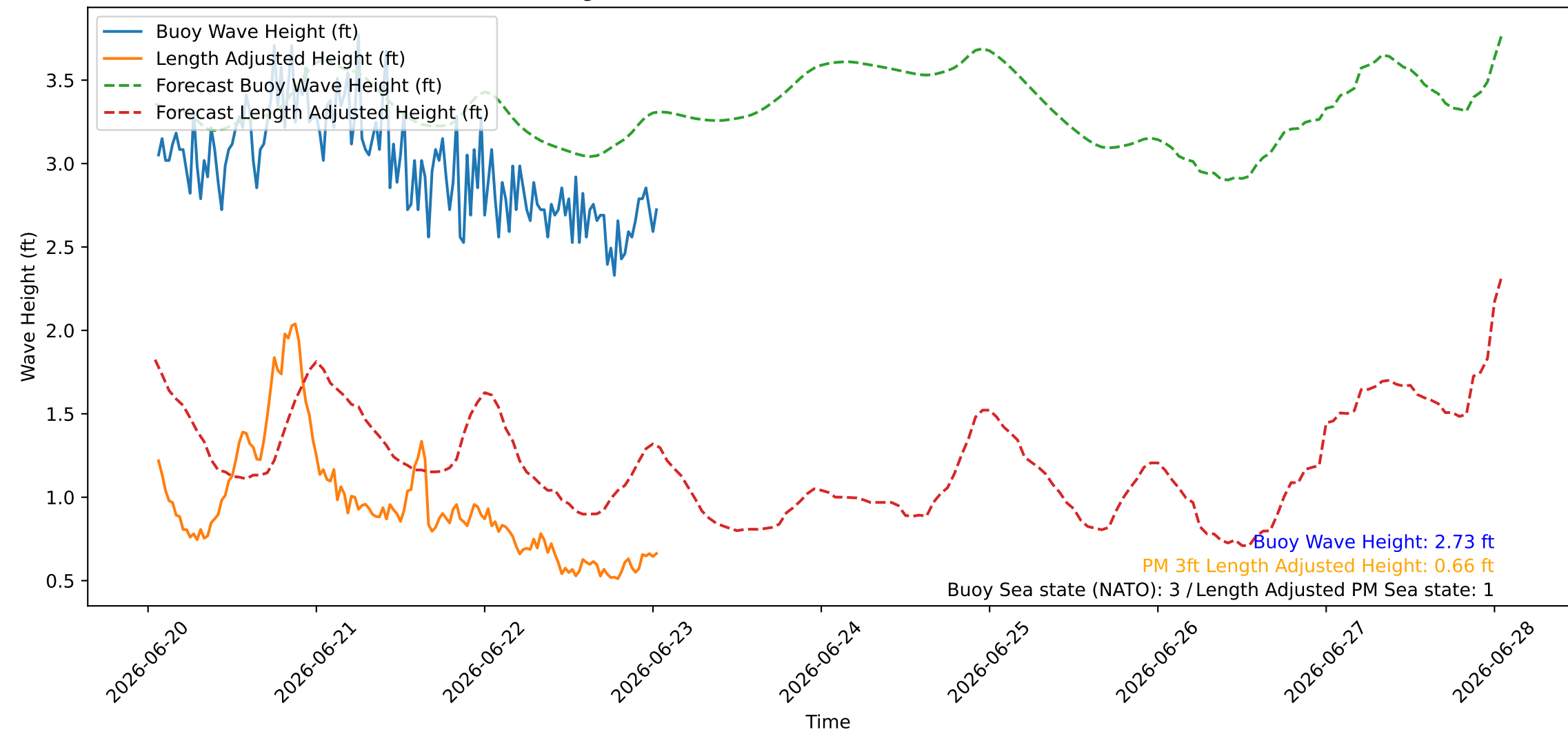
Wave Heights over Time for Red Beach at 2026-06-23 01:20:46
