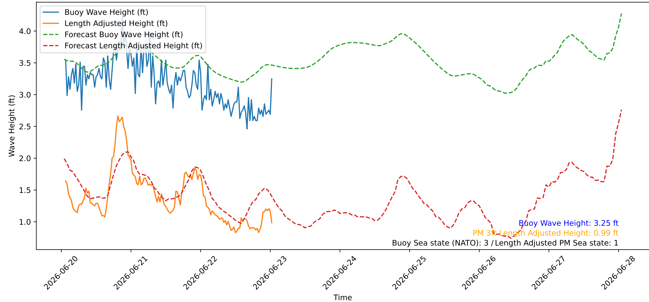
Wave Heights over Time for Green Beach at 2026-06-23 01:21:09
