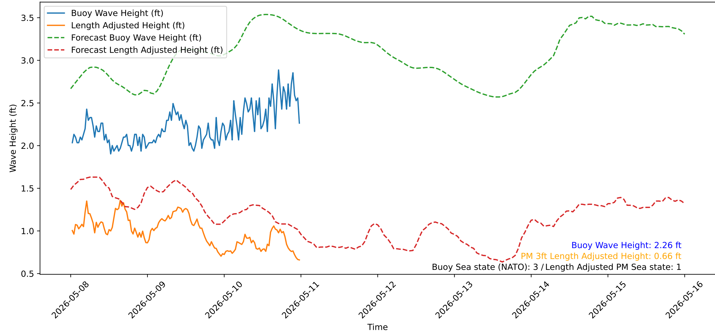
Wave Heights over Time for Red Beach at 2026-05-11 00:10:50
