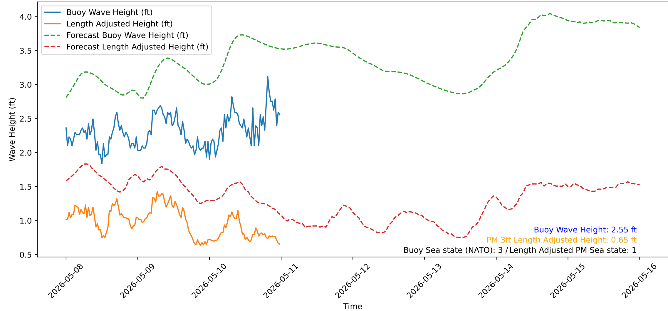
Wave Heights over Time for Green Beach at 2026-05-11 00:11:12
