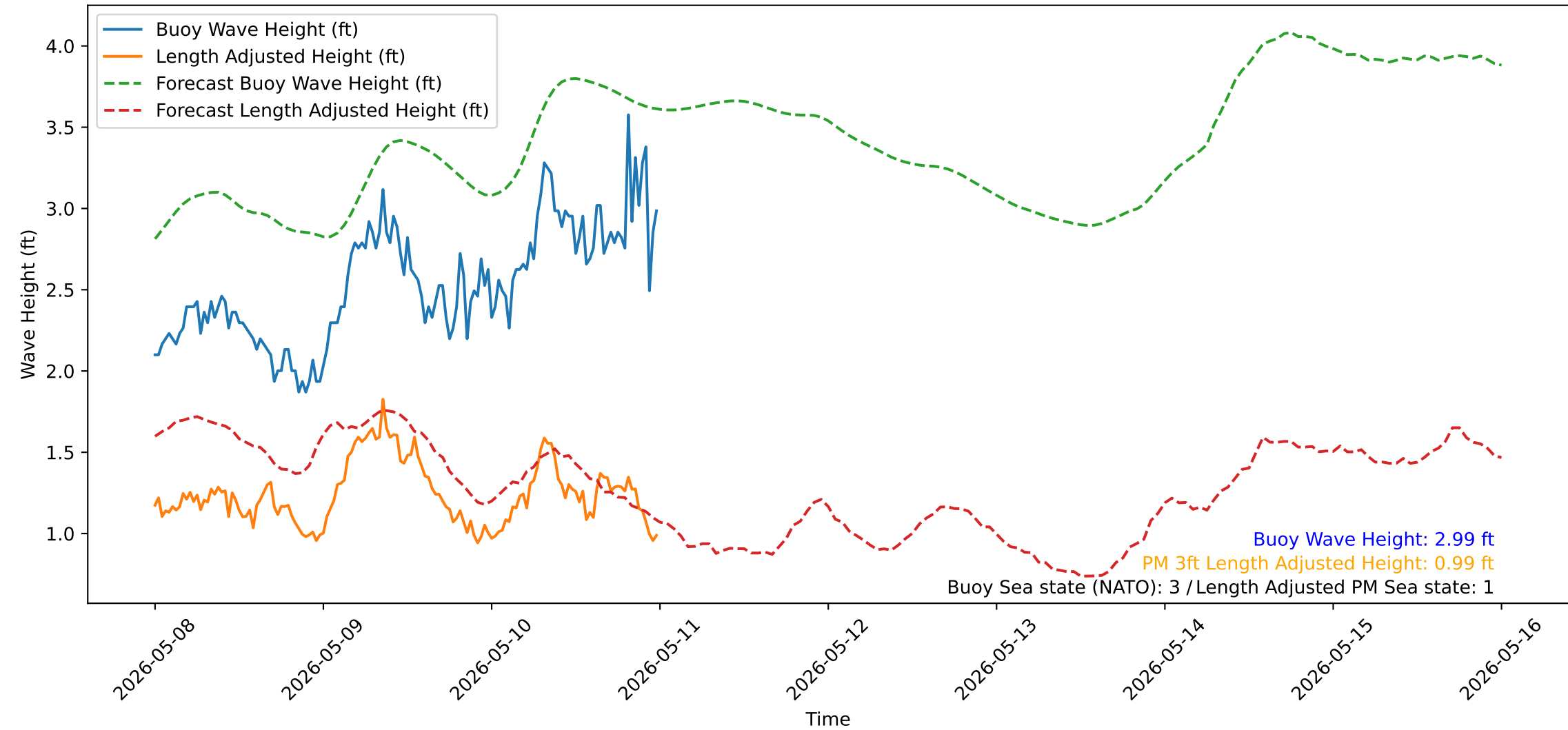
Wave Heights over Time for Oceanside Harbor at 2026-05-11 00:10:31
