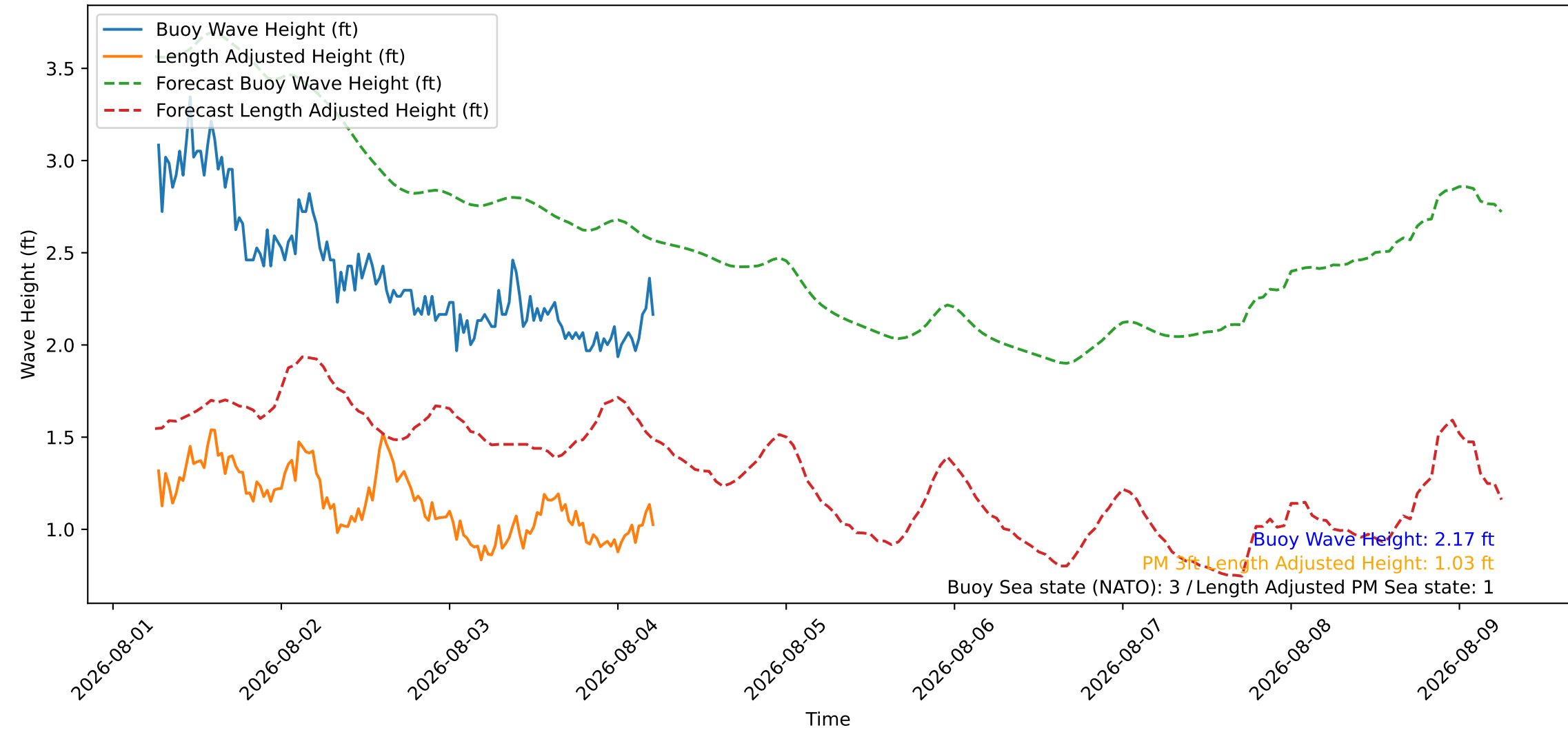
Wave Heights over Time for Red Beach at 2026-08-04 06:00:45
