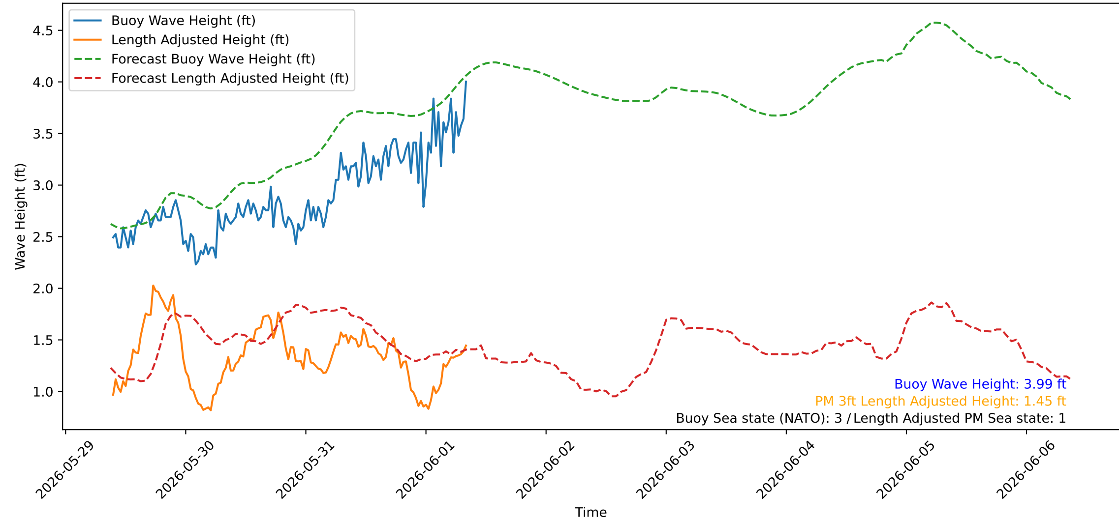
Wave Heights over Time for Red Beach at 2026-06-01 09:00:45
