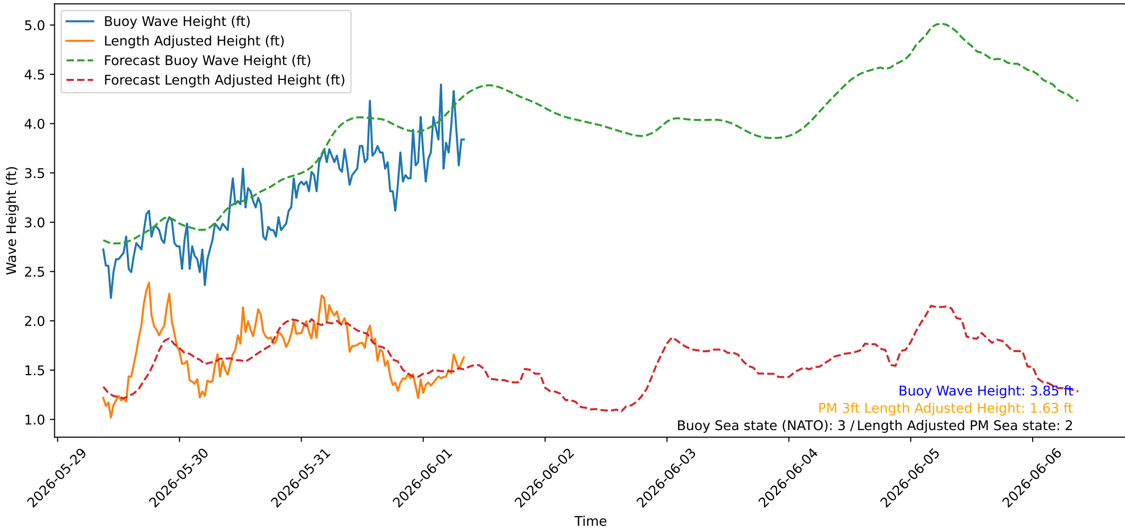
Wave Heights over Time for Oceanside Harbor at 2026-06-01 09:00:25
