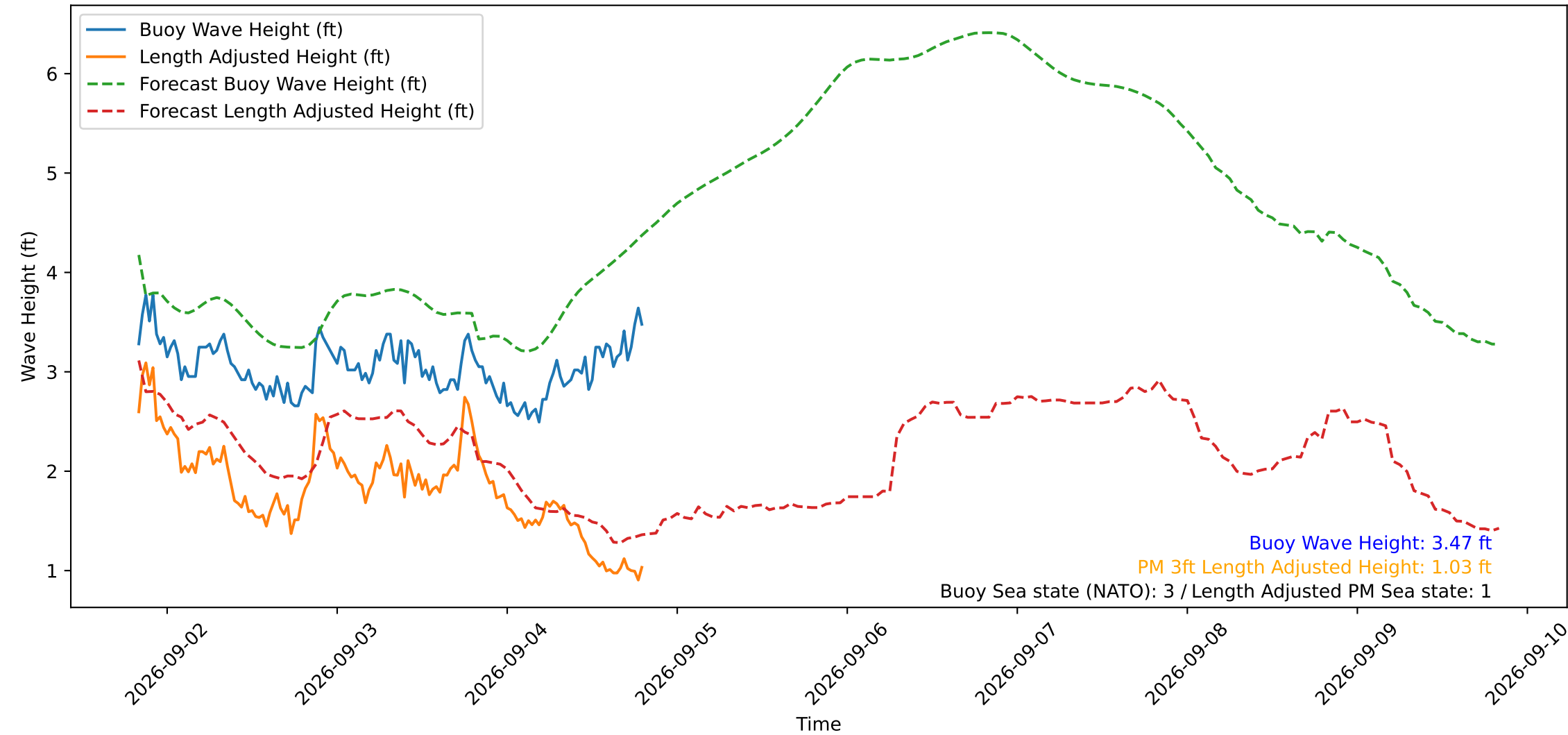
Wave Heights over Time for Green Beach at 2026-09-04 19:51:15
