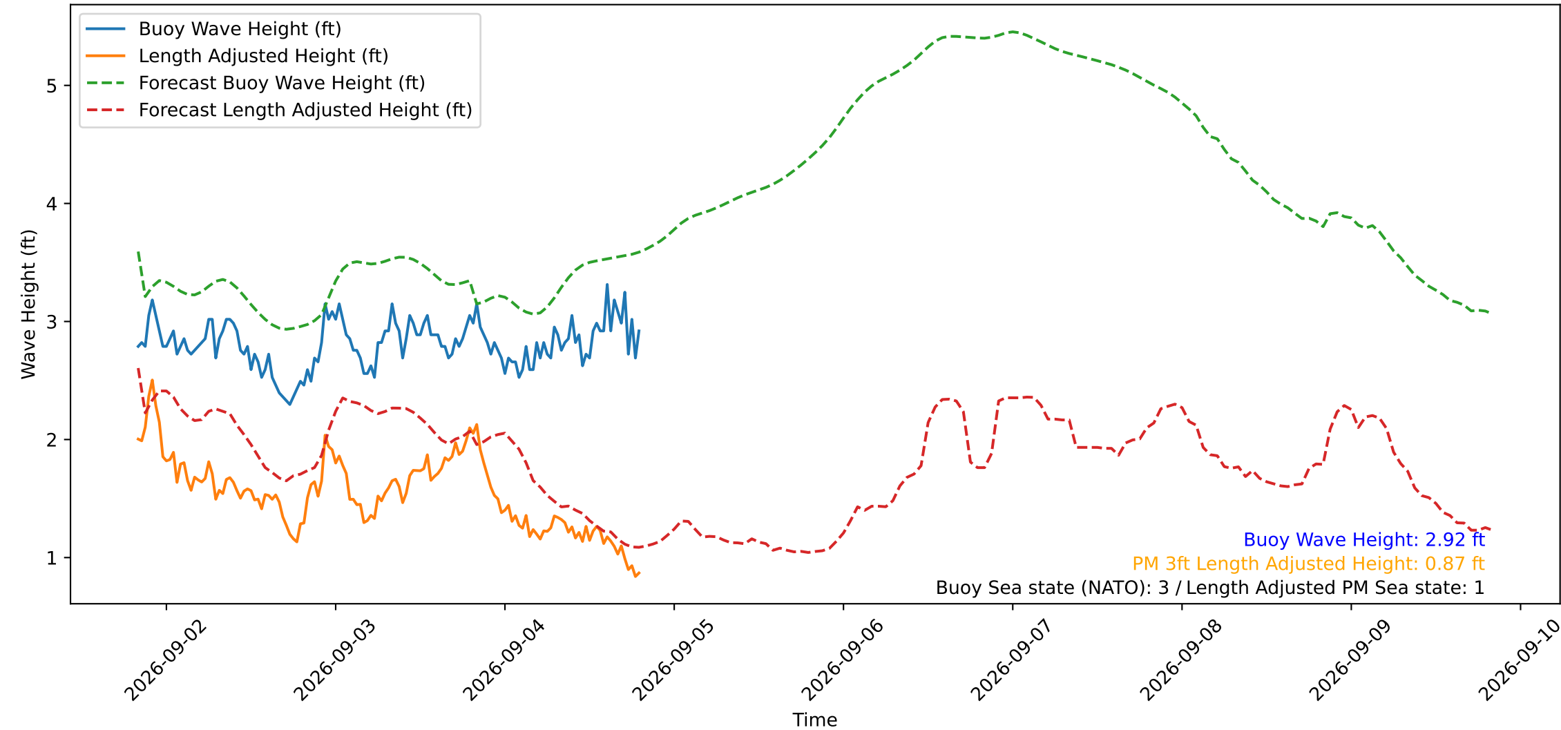
Wave Heights over Time for Red Beach at 2026-09-04 19:50:50
