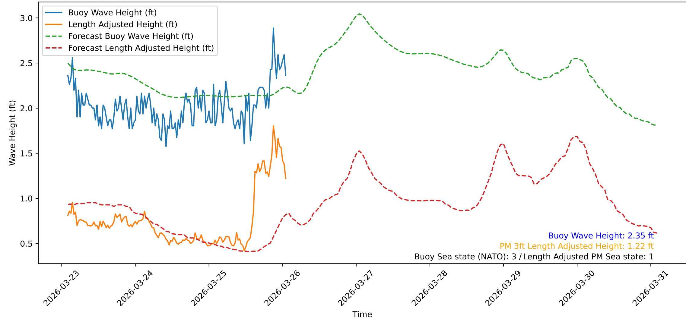
Wave Heights over Time for Oceanside Harbor at 2026-03-26 01:50:32
