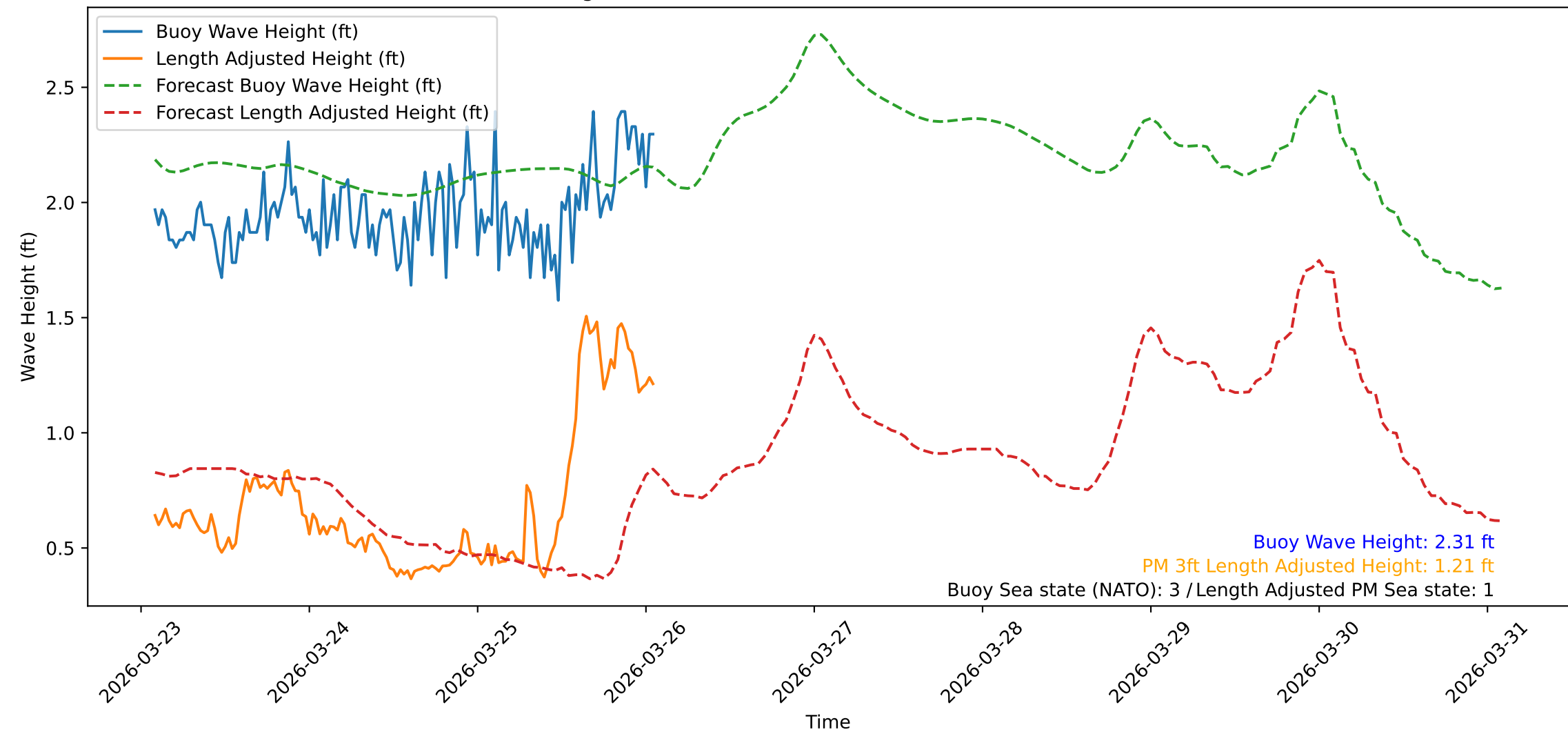
Wave Heights over Time for Red Beach at 2026-03-26 01:50:48
