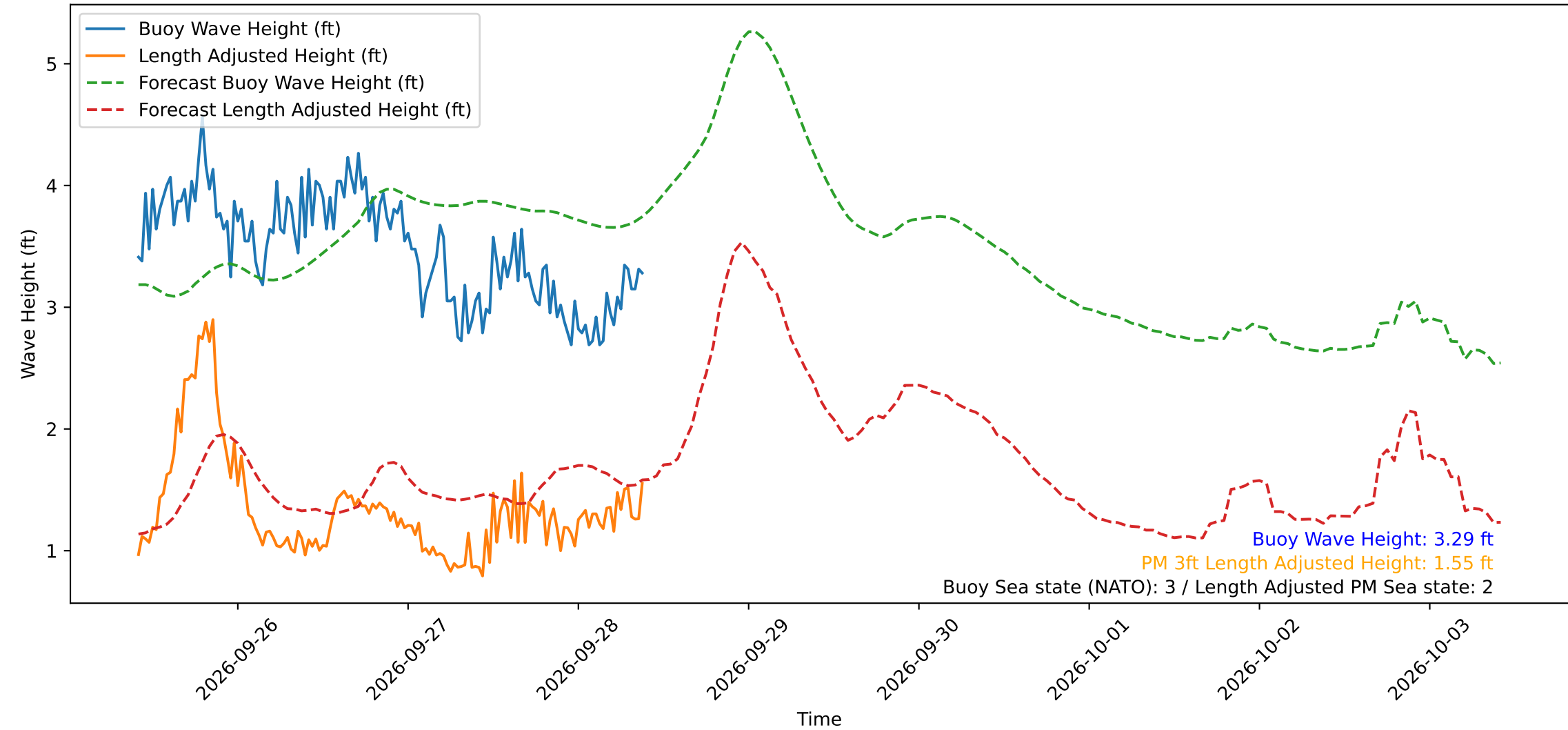
Wave Heights over Time for Green Beach at 2026-09-28 09:41:12
