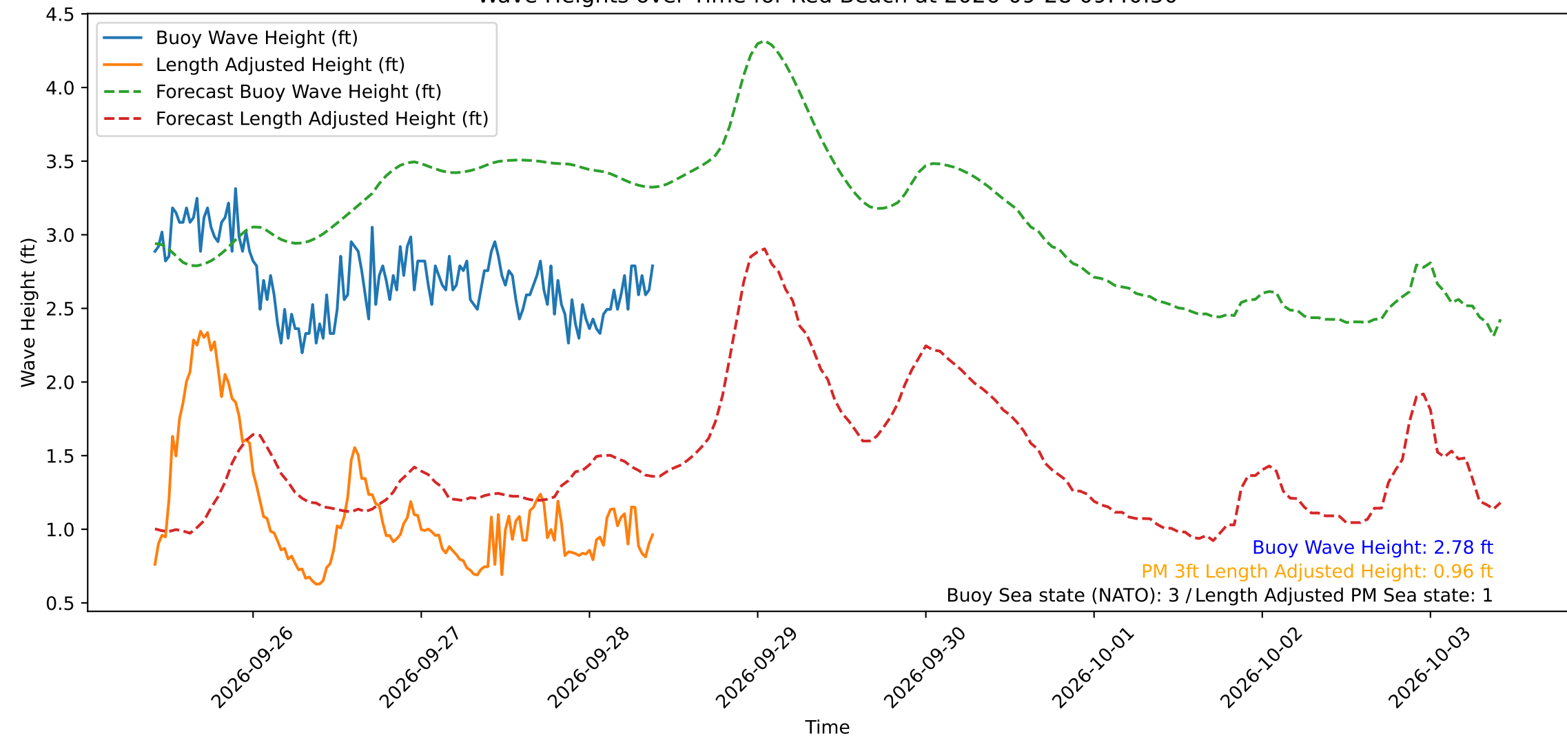
Wave Heights over Time for Red Beach at 2026-09-28 09:40:50
