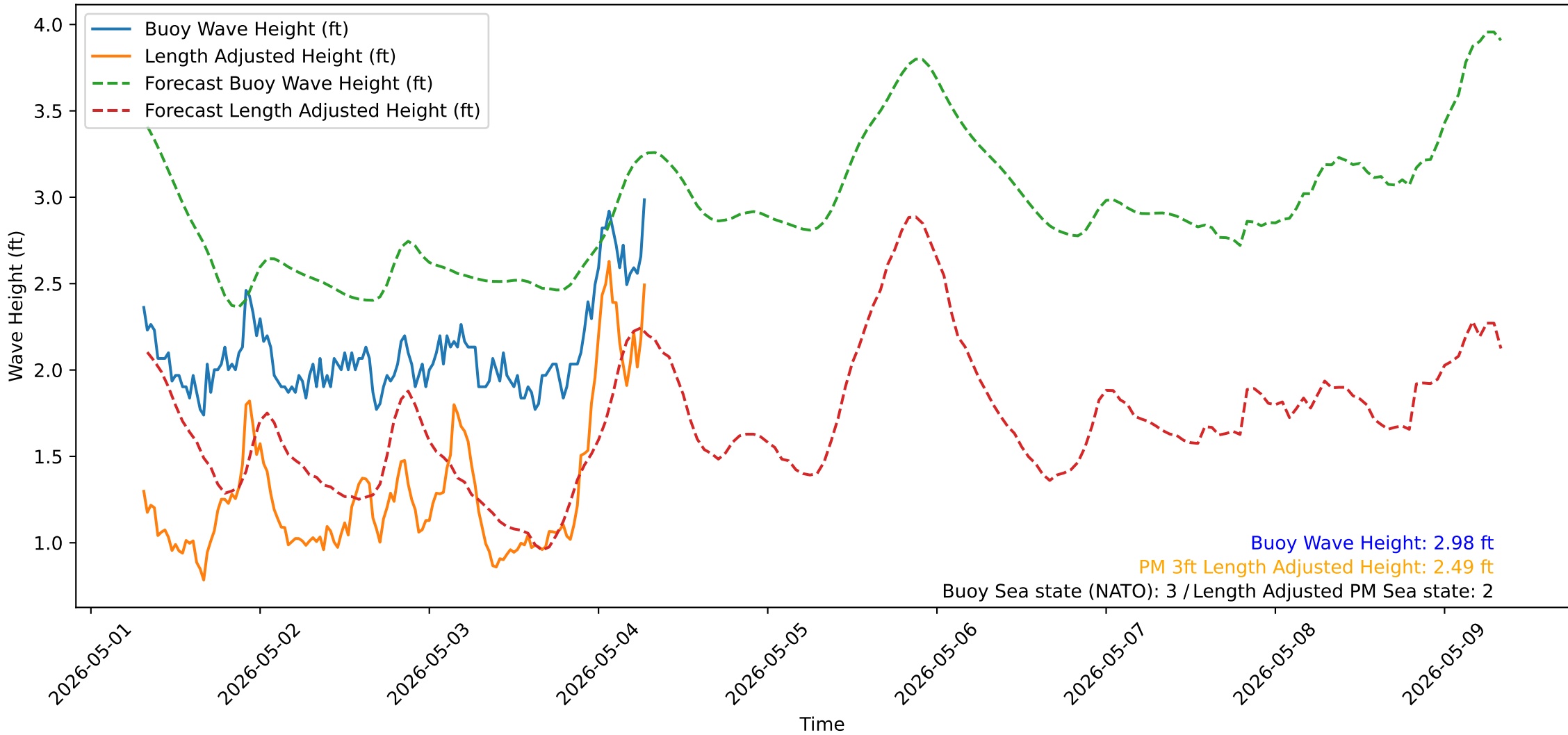
Wave Heights over Time for Green Beach at 2026-05-04 07:31:13
