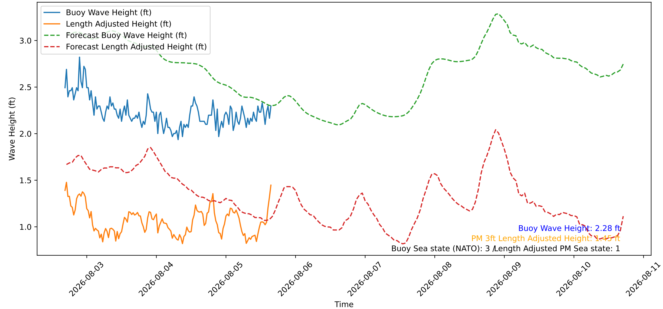
Wave Heights over Time for Green Beach at 2026-08-05 16:31:09
