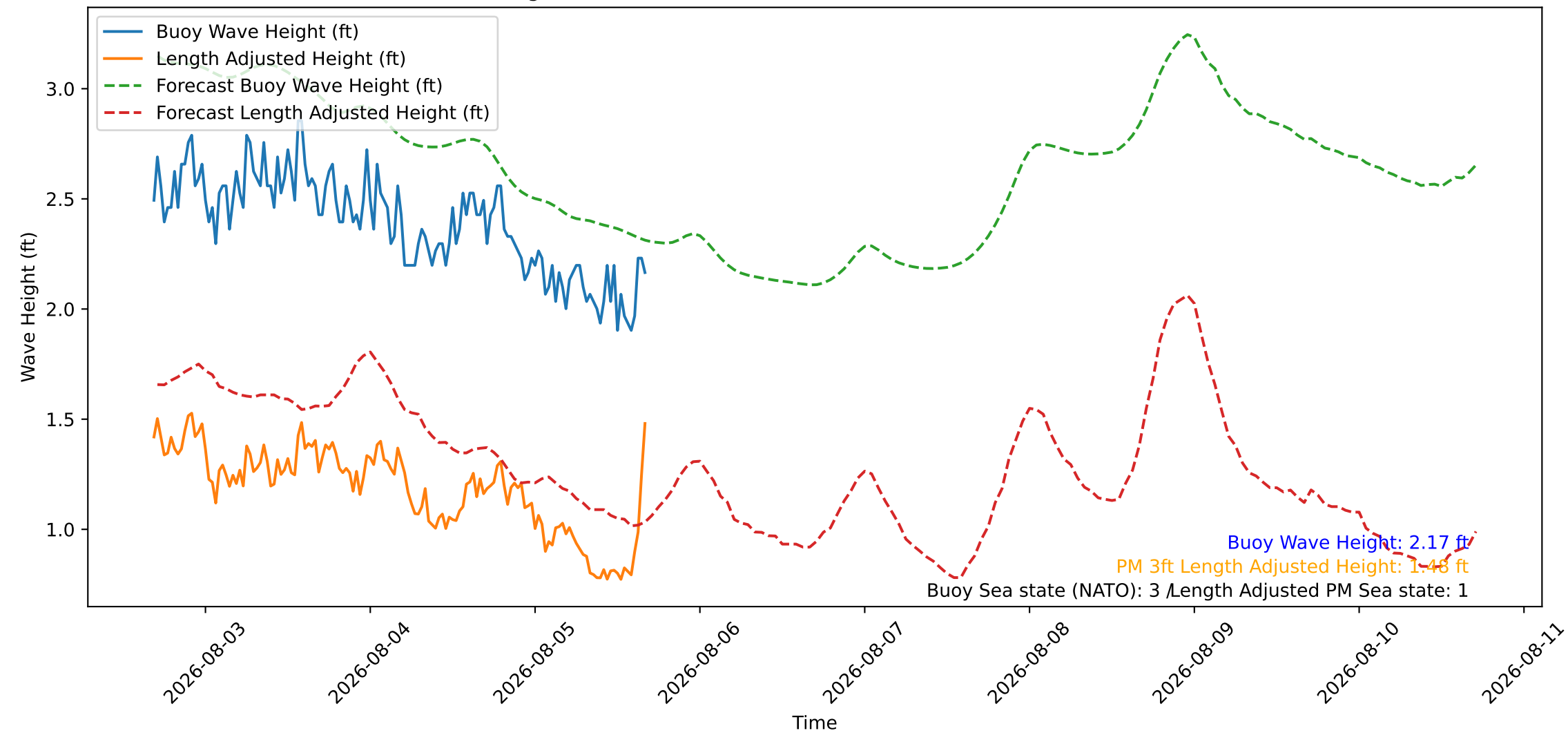
Wave Heights over Time for Oceanside Harbor at 2026-08-05 16:30:27
