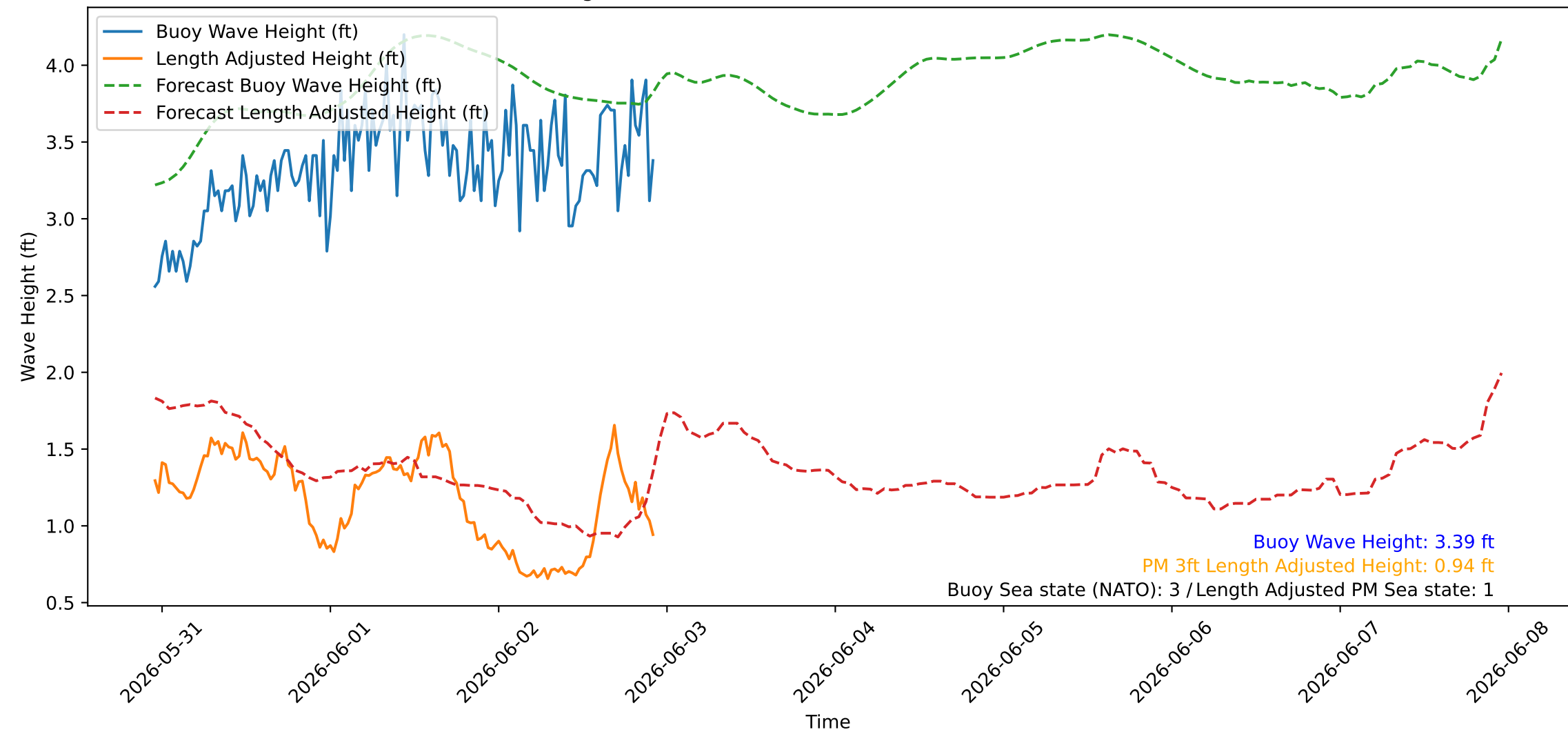
Wave Heights over Time for Red Beach at 2026-06-02 22:50:47
