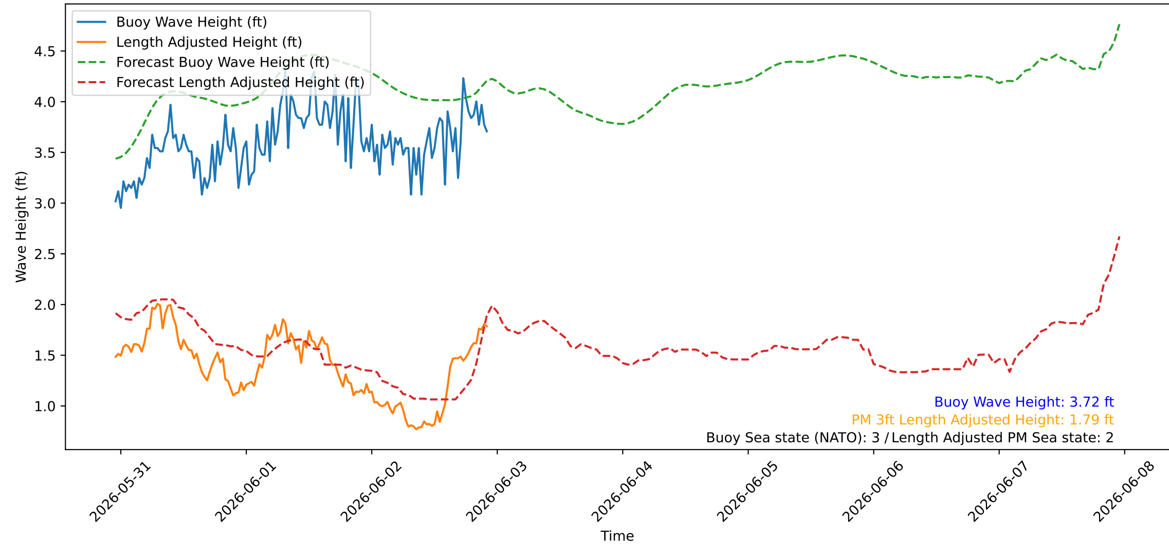
Wave Heights over Time for Green Beach at 2026-06-02 22:51:09
