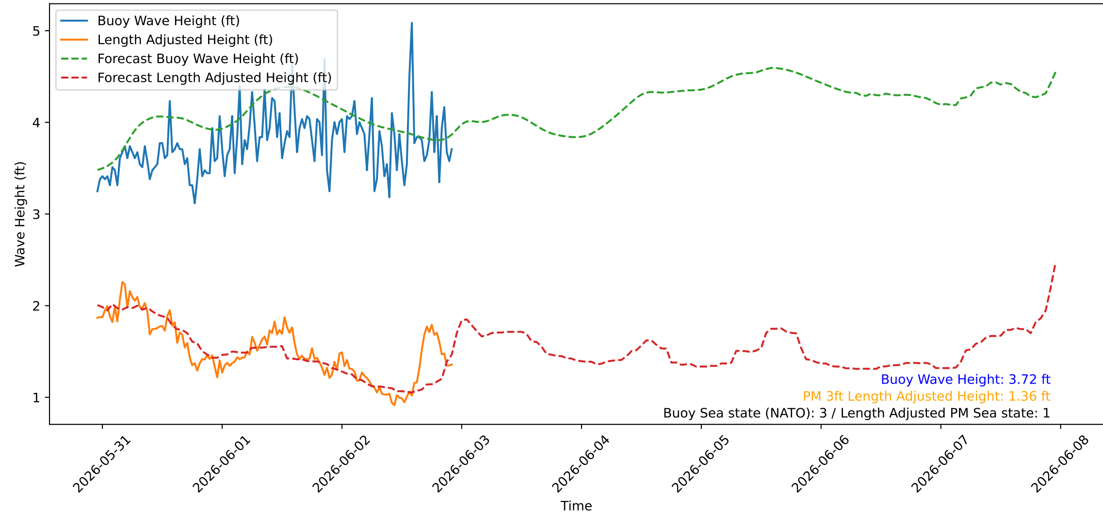
Wave Heights over Time for Oceanside Harbor at 2026-06-02 22:50:26
