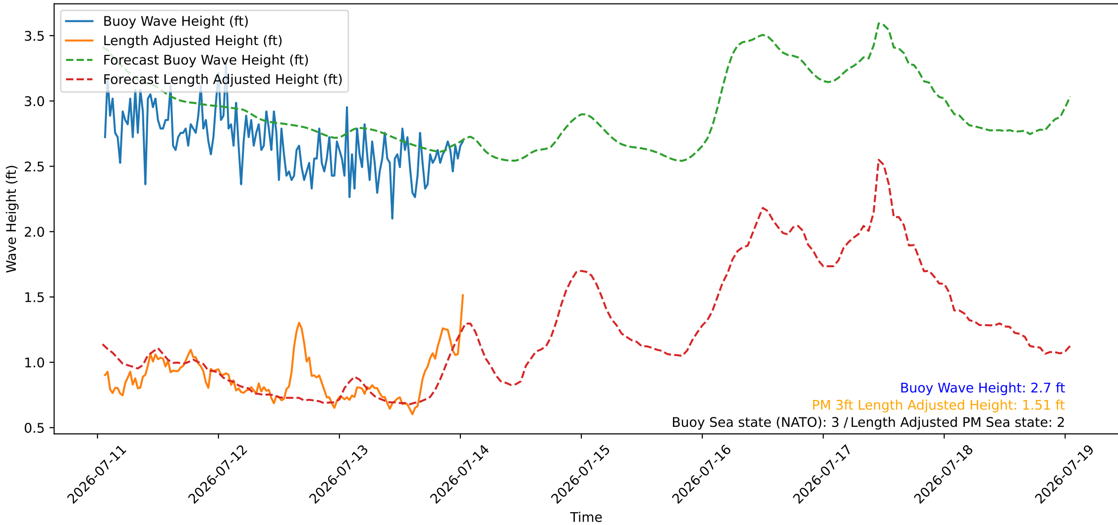
Wave Heights over Time for Oceanside Harbor at 2026-07-14 01:20:26
