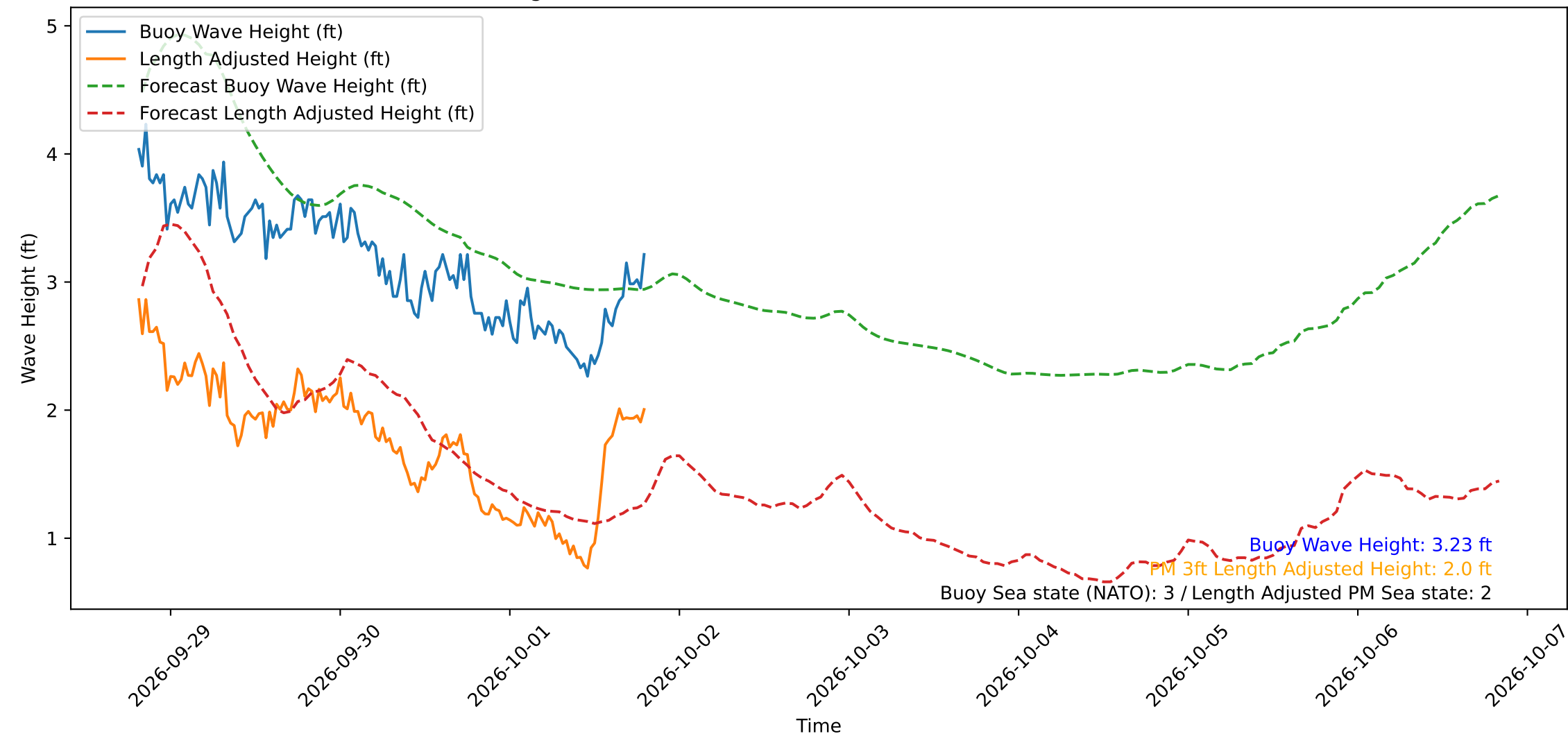
Wave Heights over Time for Oceanside Harbor at 2026-10-01 19:40:30
