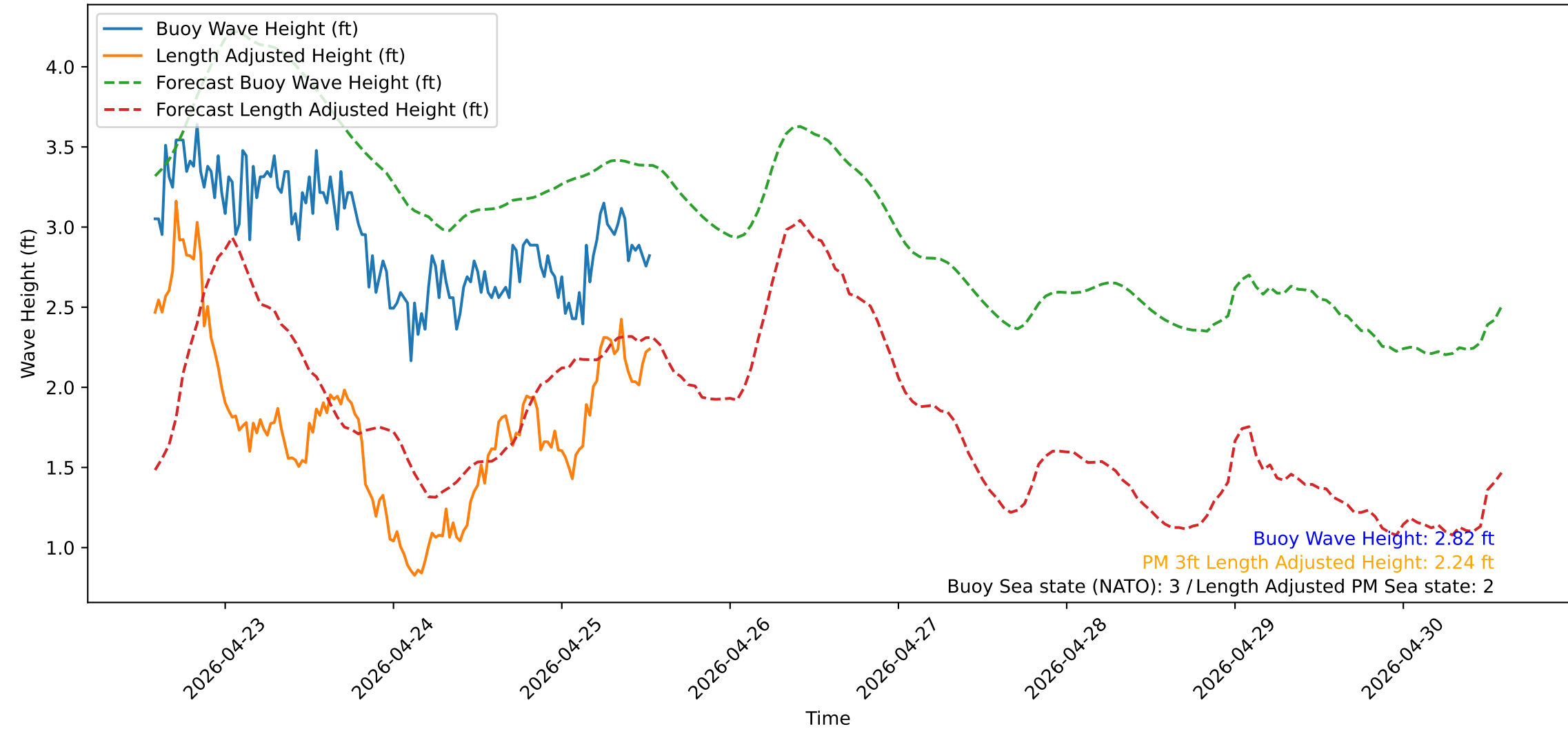
Wave Heights over Time for Red Beach at 2026-04-25 13:30:50
