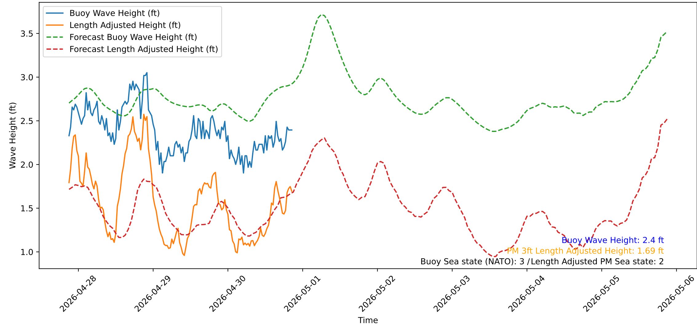
Wave Heights over Time for Oceanside Harbor at 2026-04-30 21:10:31
