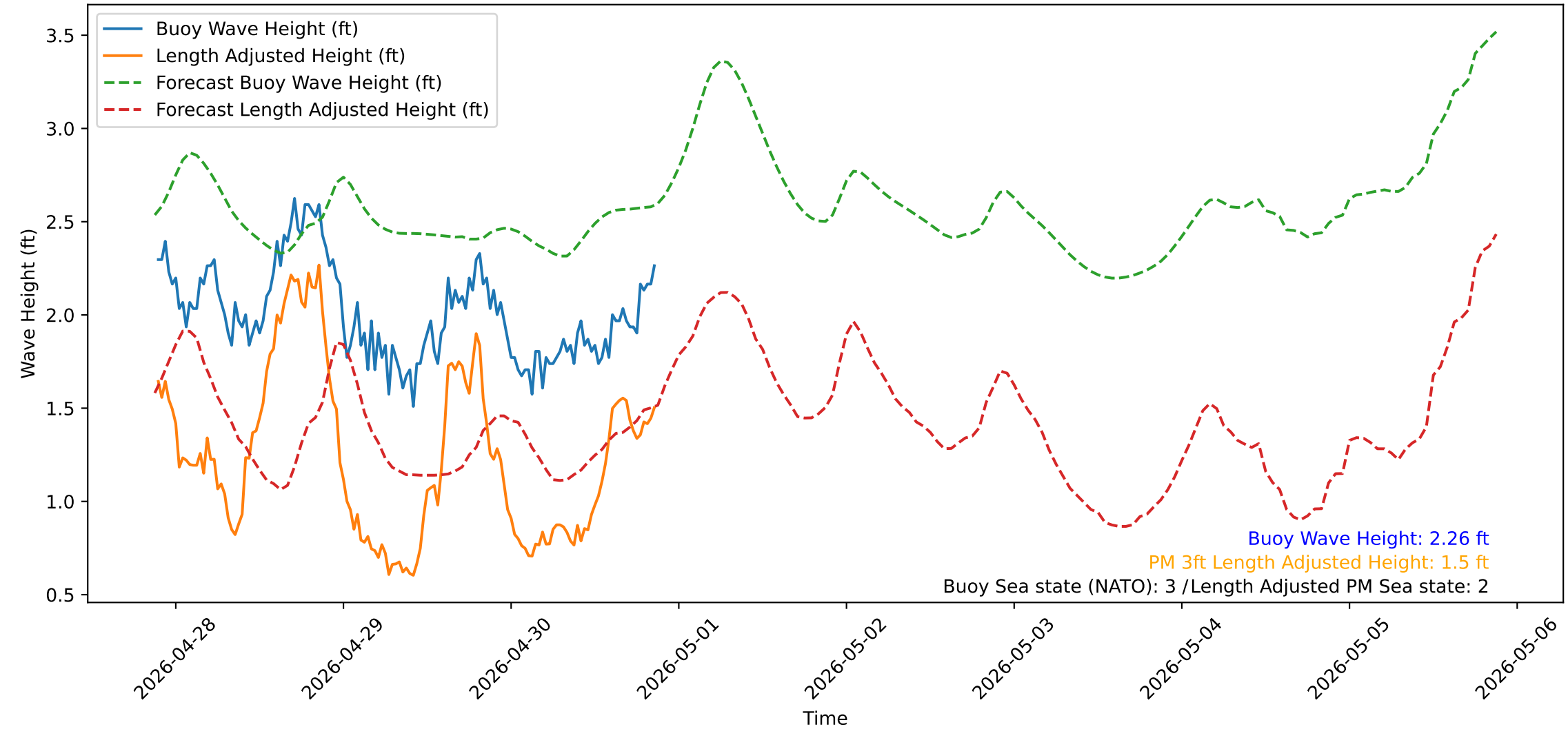
Wave Heights over Time for Red Beach at 2026-04-30 21:10:50
