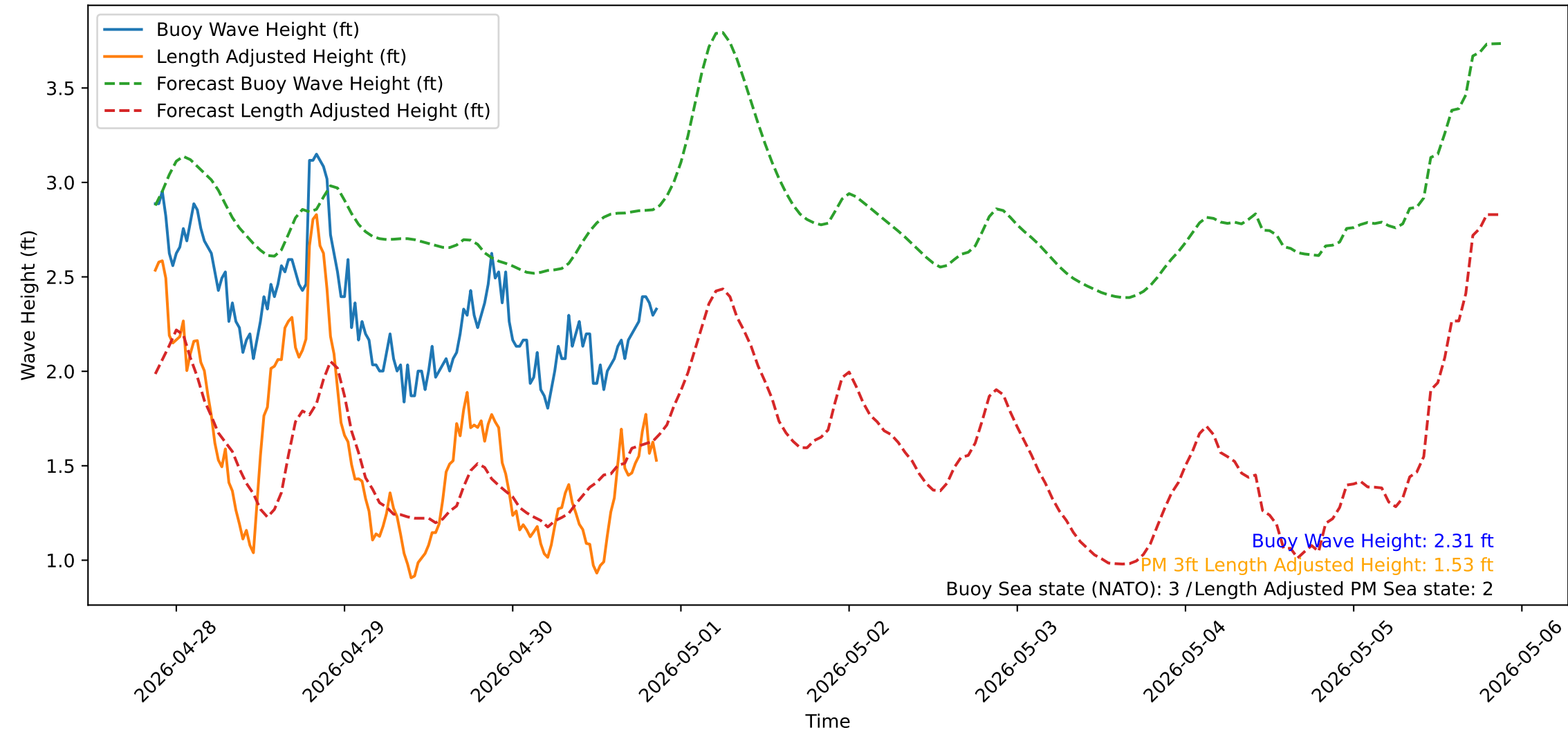
Wave Heights over Time for Green Beach at 2026-04-30 21:11:13
