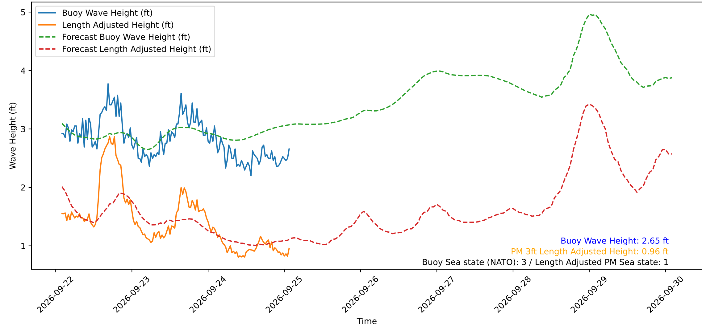
Wave Heights over Time for Oceanside Harbor at 2026-09-25 02:10:30
