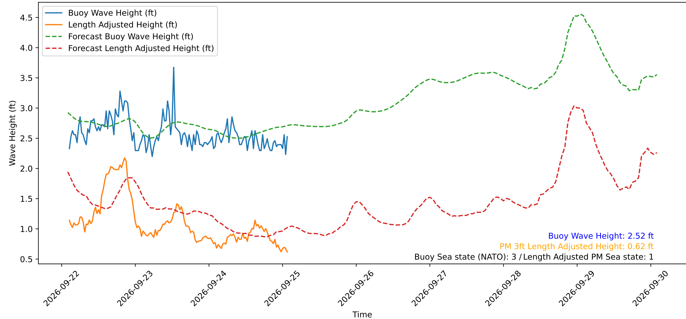
Wave Heights over Time for Red Beach at 2026-09-25 02:10:50
