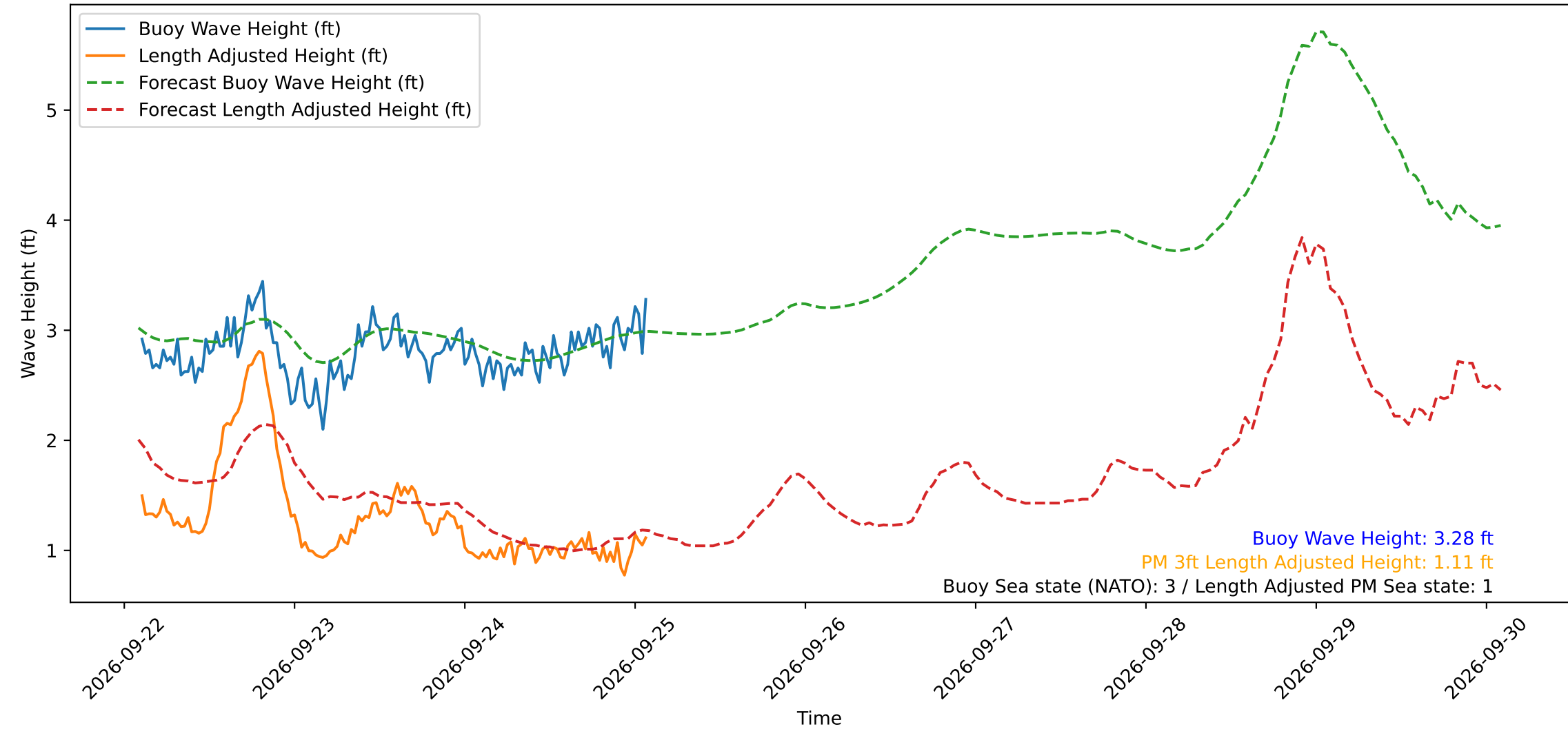
Wave Heights over Time for Green Beach at 2026-09-25 02:11:12
