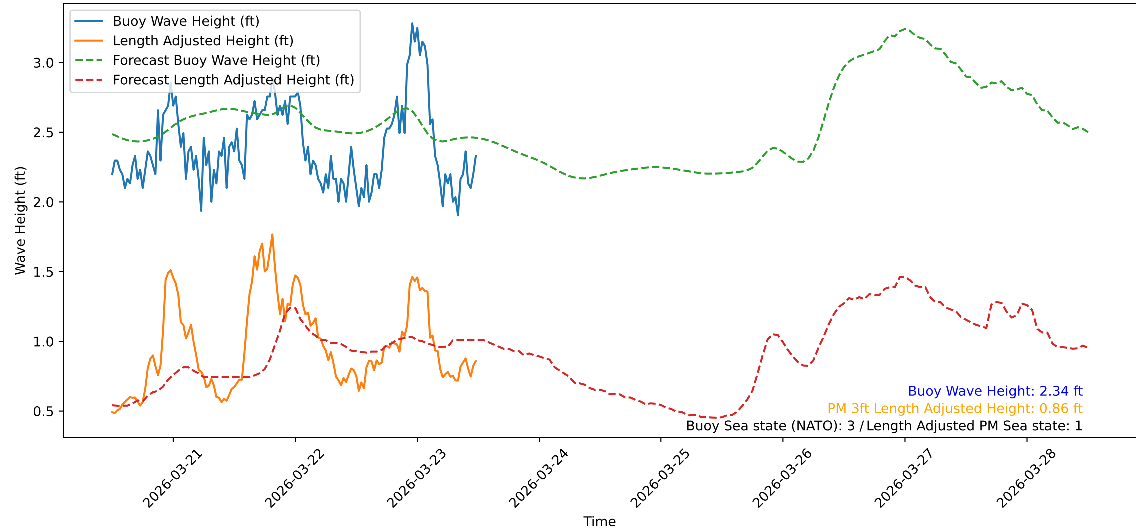
Wave Heights over Time for Green Beach at 2026-03-23 12:11:10
