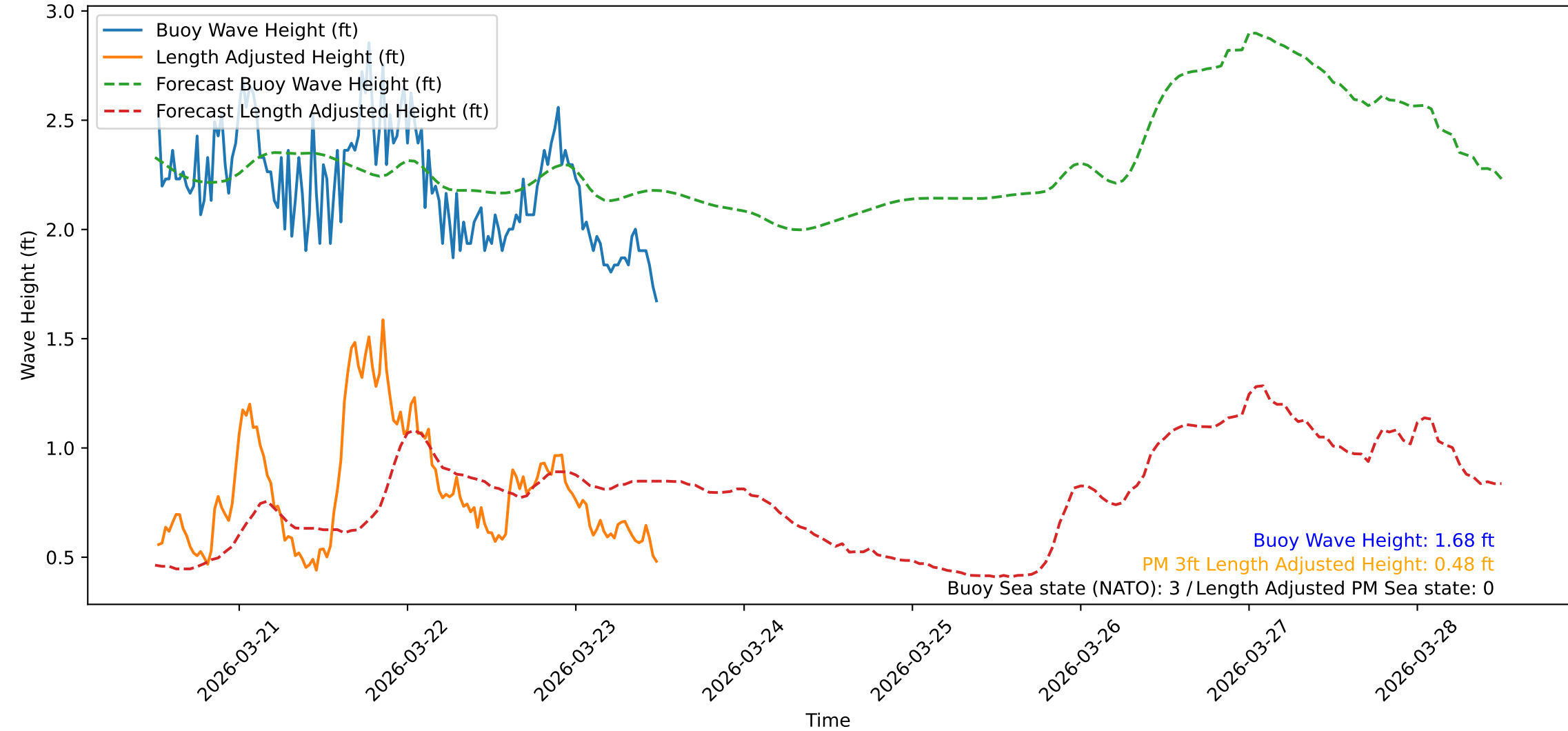
Wave Heights over Time for Red Beach at 2026-03-23 12:10:47
