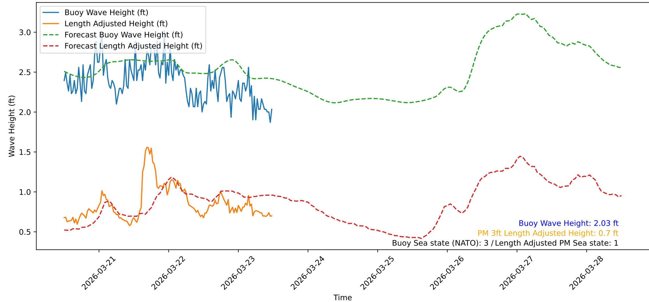
Wave Heights over Time for Oceanside Harbor at 2026-03-23 12:10:31
