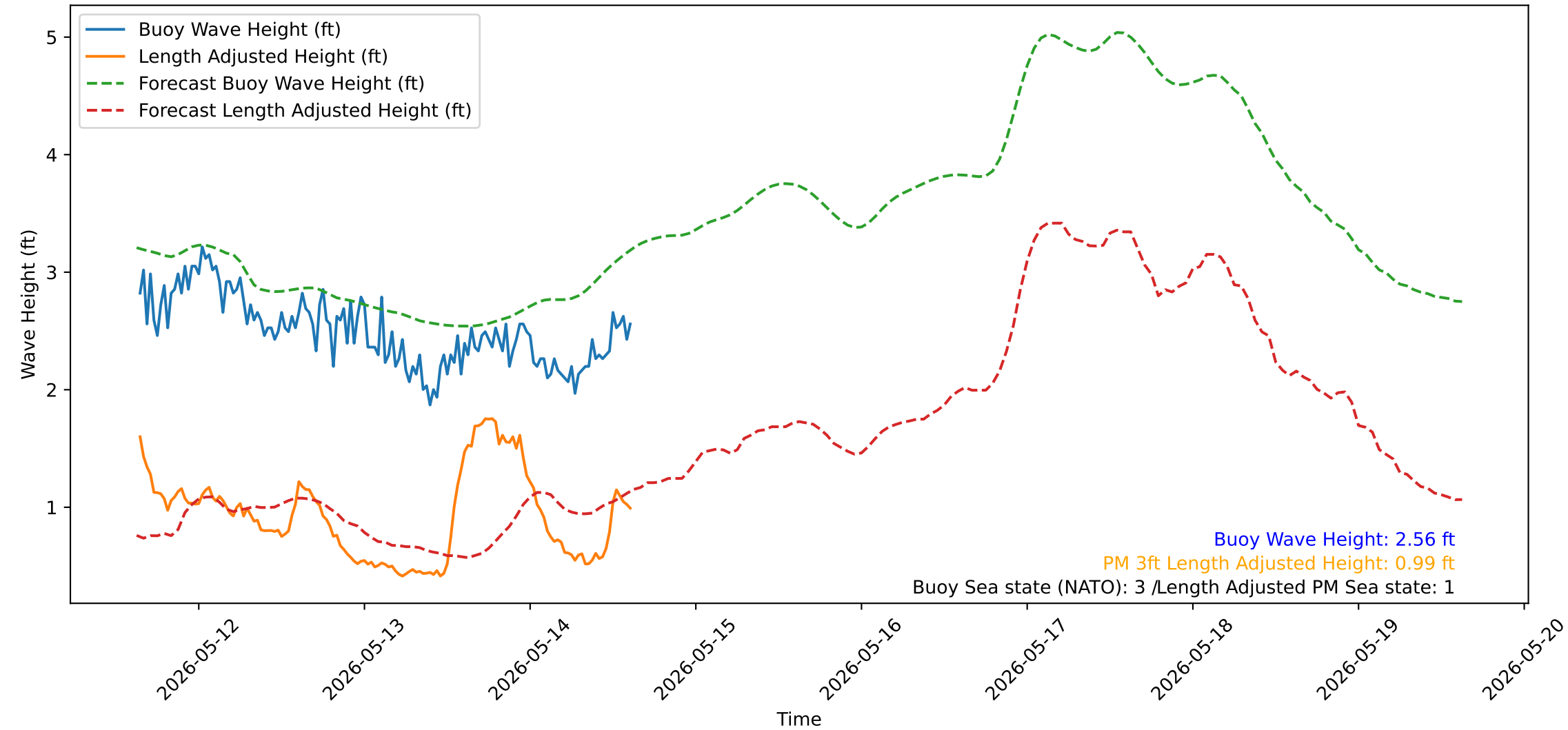
Wave Heights over Time for Red Beach at 2026-05-14 15:10:51
