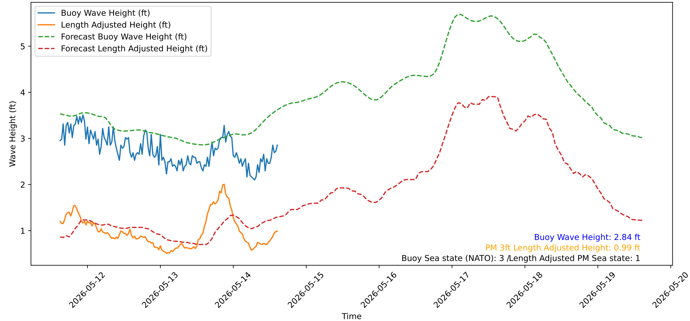
Wave Heights over Time for Green Beach at 2026-05-14 15:11:13
