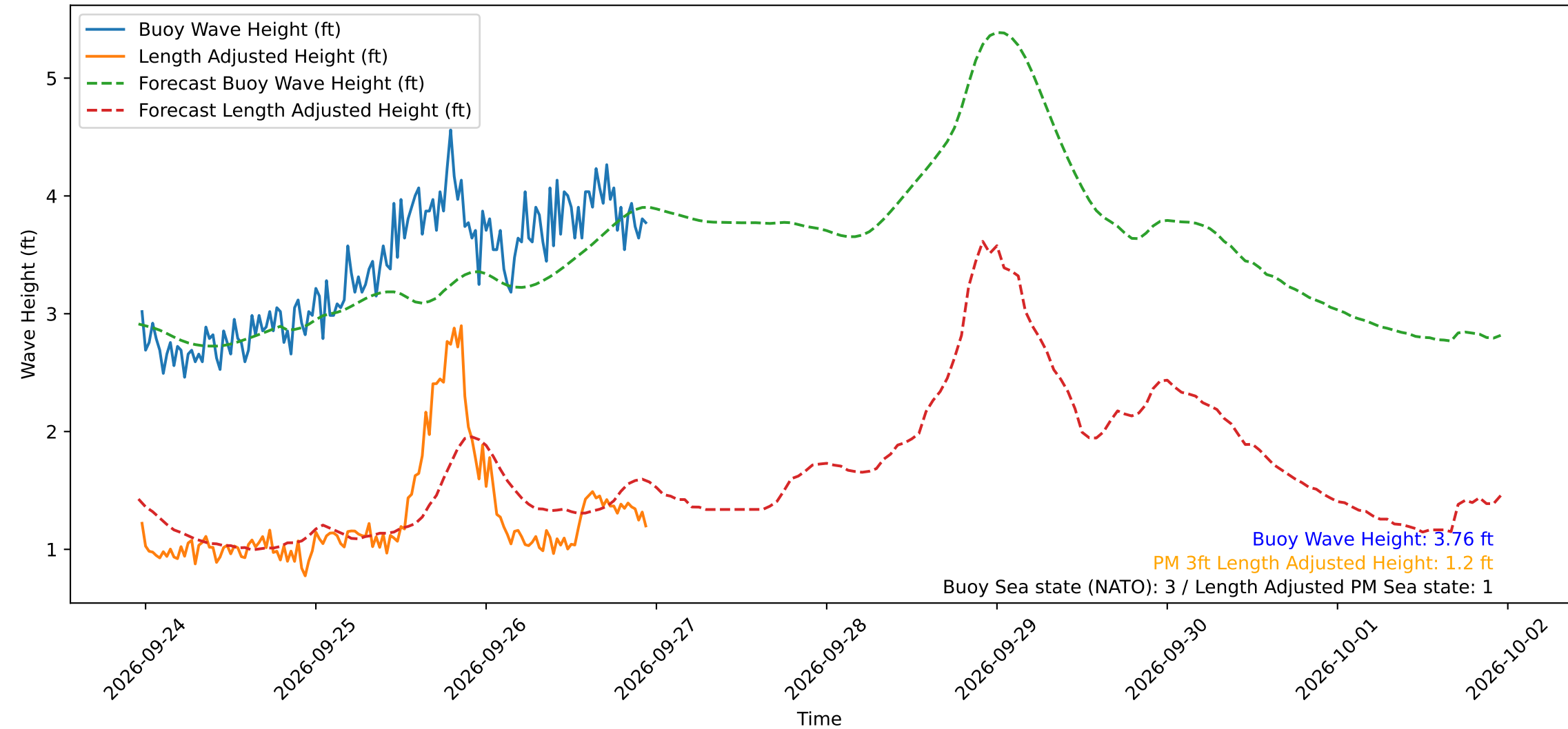
Wave Heights over Time for Green Beach at 2026-09-26 23:21:15
