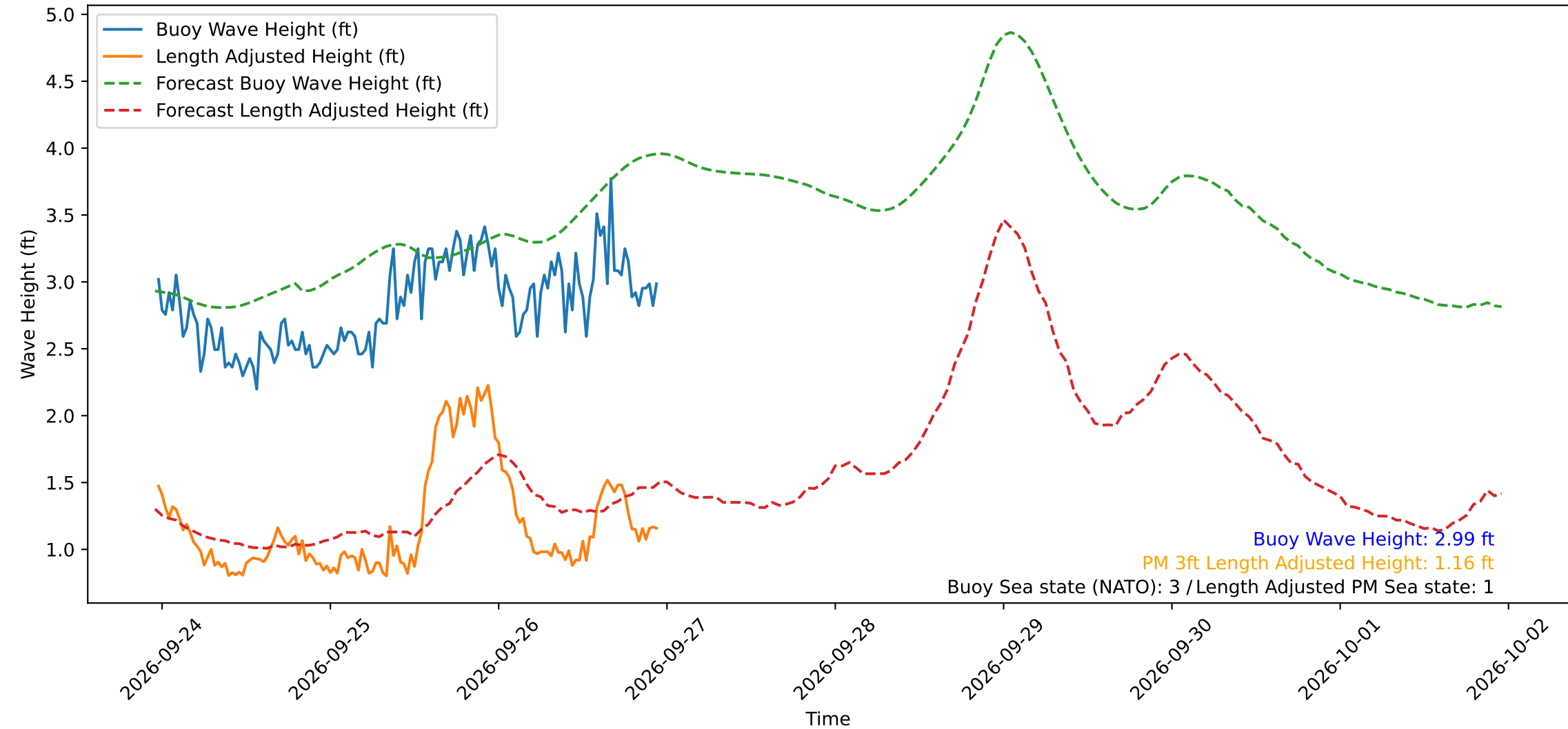
Wave Heights over Time for Oceanside Harbor at 2026-09-26 23:20:30
