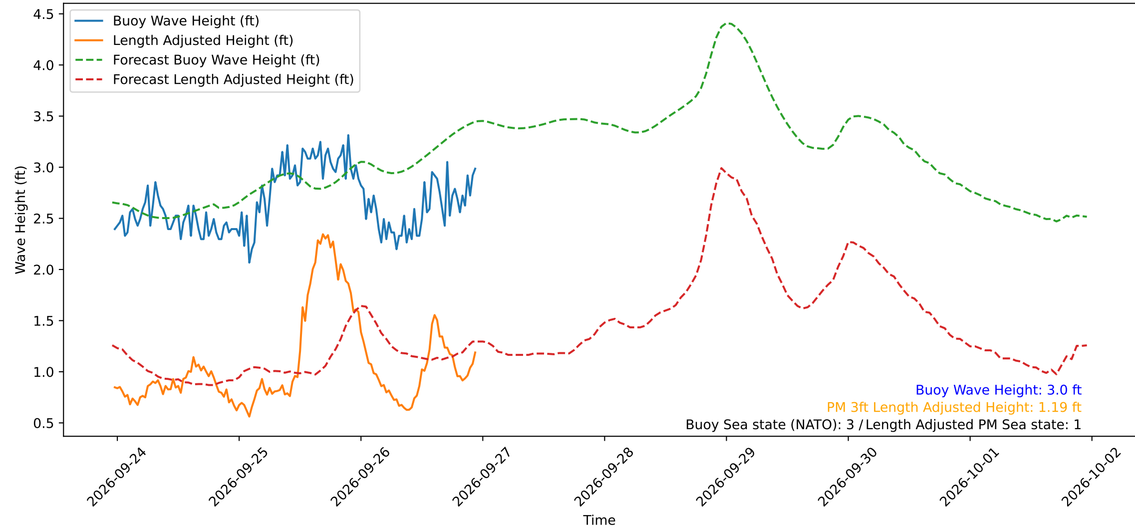
Wave Heights over Time for Red Beach at 2026-09-26 23:20:51
