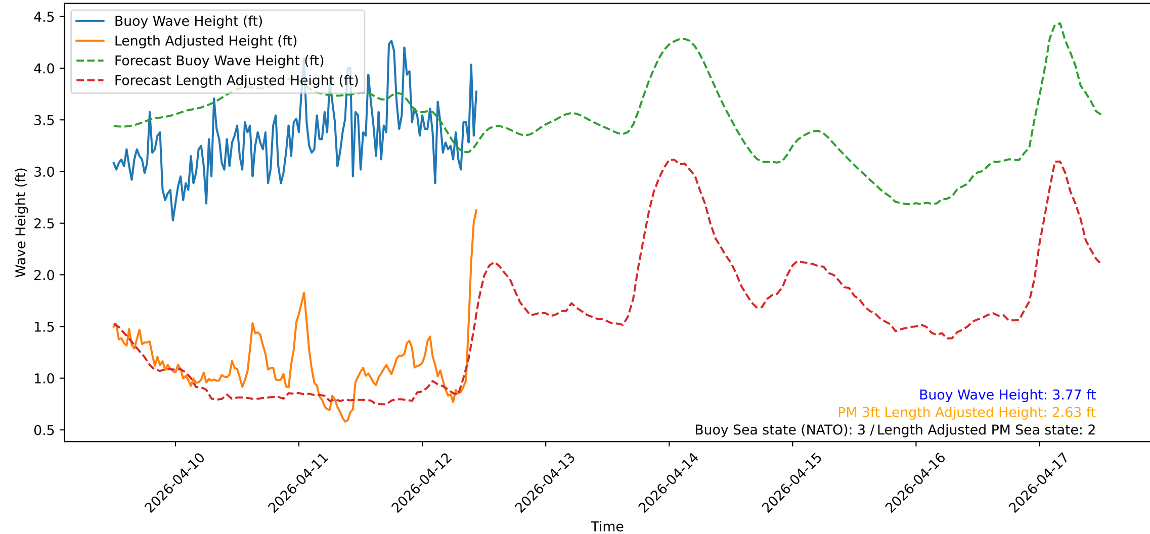
Wave Heights over Time for Red Beach at 2026-04-12 11:40:51
