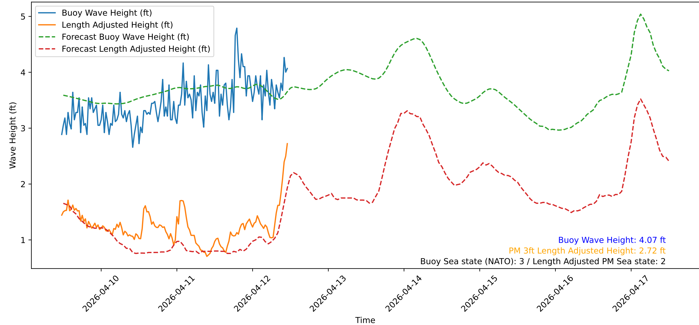
Wave Heights over Time for Oceanside Harbor at 2026-04-12 11:40:32
