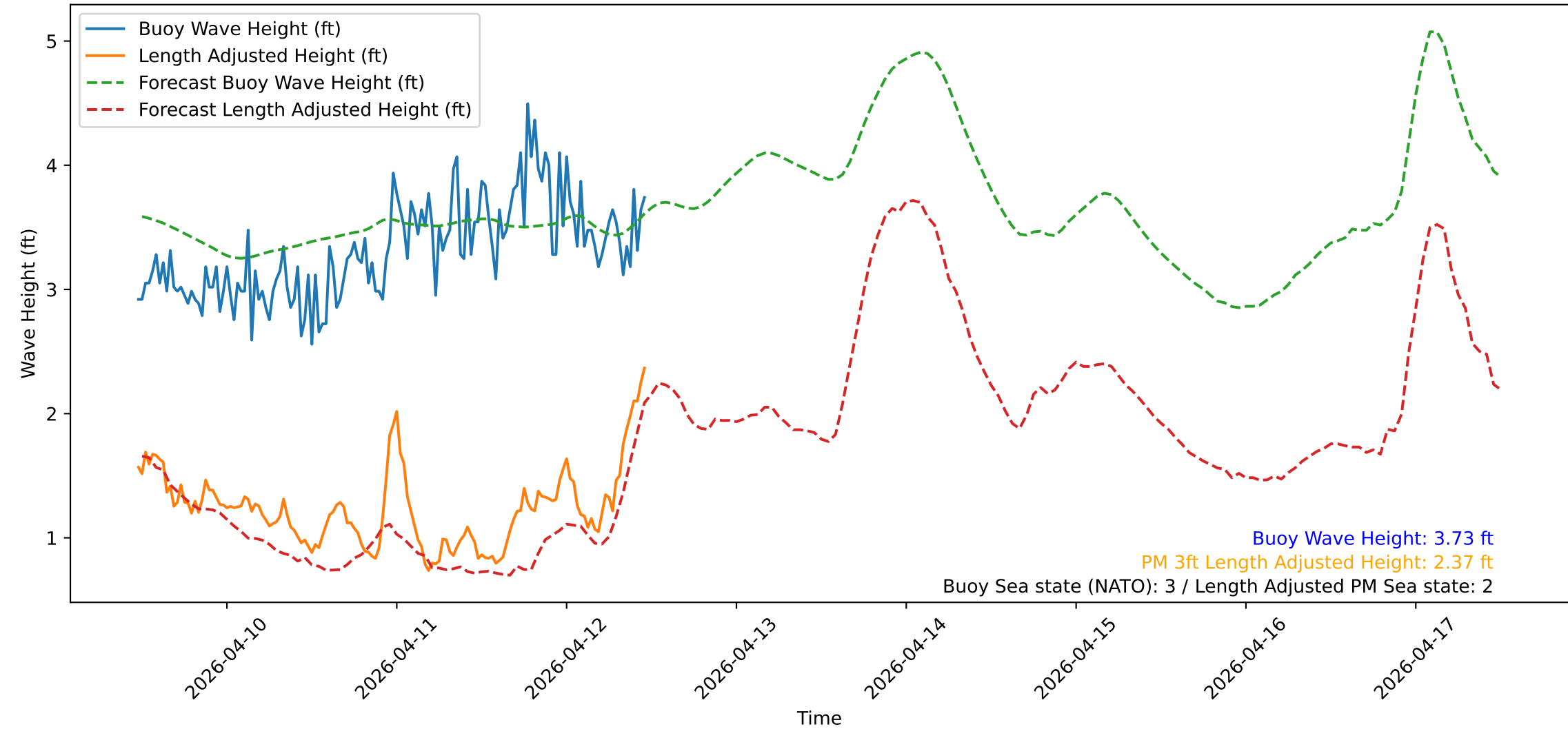
Wave Heights over Time for Green Beach at 2026-04-12 11:41:13
