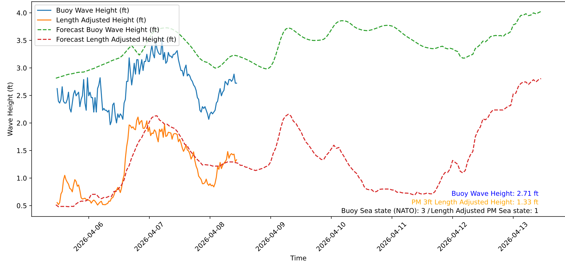
Wave Heights over Time for Red Beach at 2026-04-08 11:20:47
