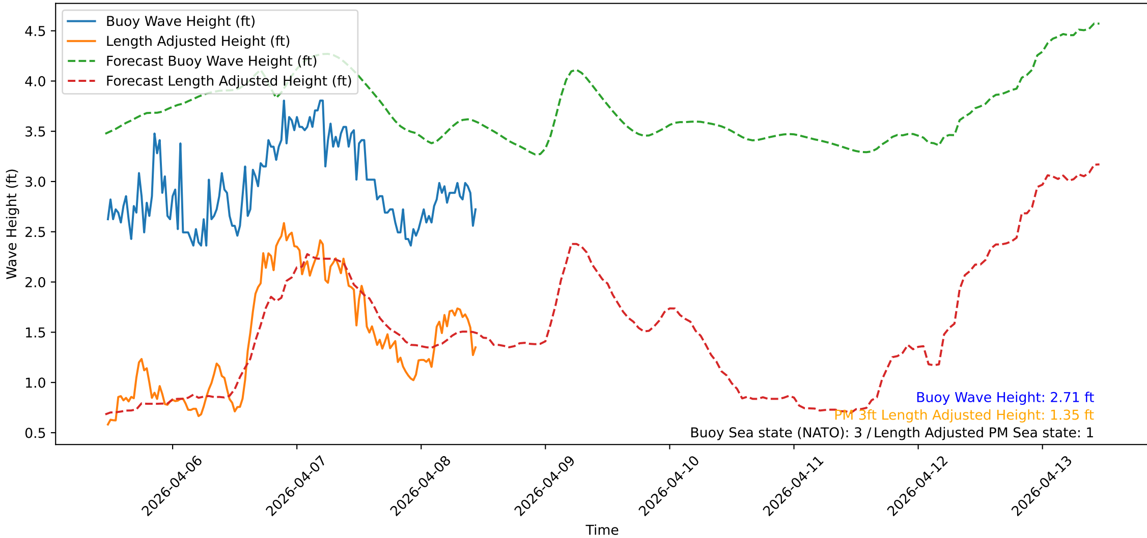
Wave Heights over Time for Green Beach at 2026-04-08 11:21:09
