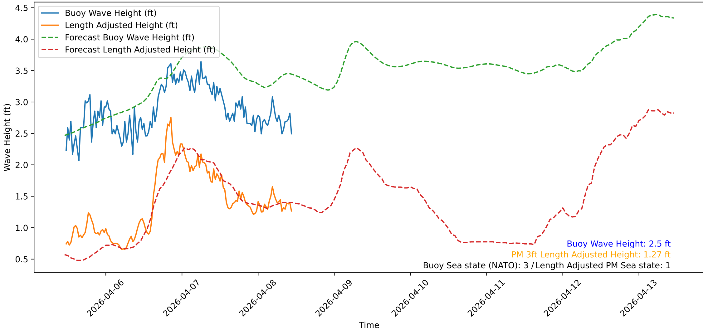
Wave Heights over Time for Oceanside Harbor at 2026-04-08 11:20:31
